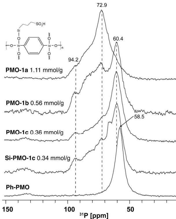
Figure 1. 31 P MAS NMR spectra of TEPO probe molecules adsorbed on PMO-1a, PMO-1b, PMO-1c, Si-PMO-1c and Ph-PMO.
