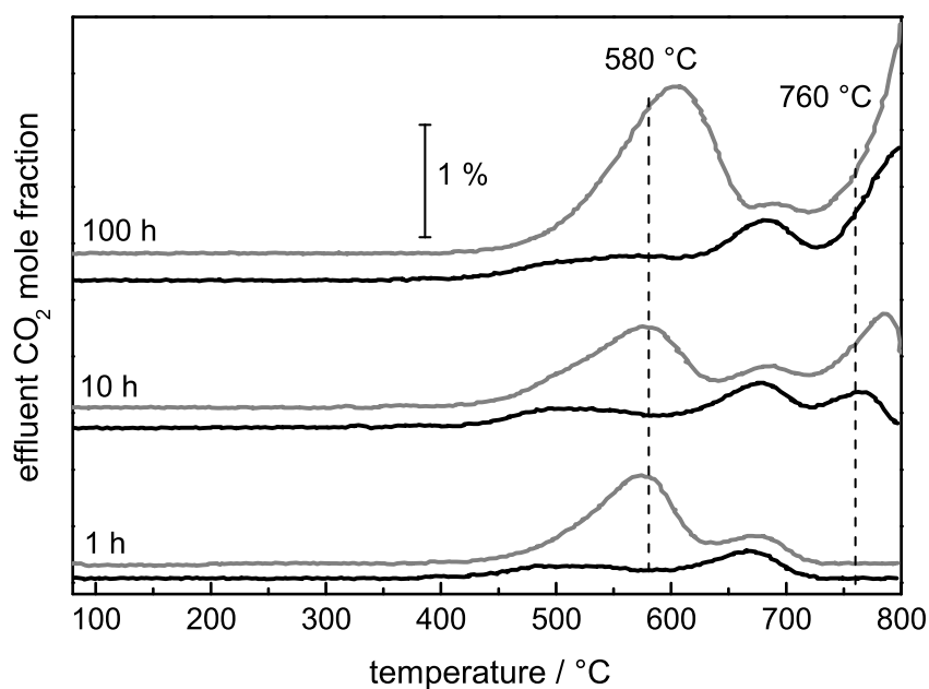
Figure 11: TPO profiles after 1, 10, and 100 h of DRM at 900 °C with 25 mol% after T_{Red} = 850 °C (black) and 50 mol% Ni after T_{Red} = 800 °C (grey). The effluent mole fractions of \text{CO}_2 were detected while heating with 5 °C \text{min}^{-1} up to 800 °C in a total flow of 40 \text{Nml min}^{-1} 4.5% \text{O}_2 in Ar.
