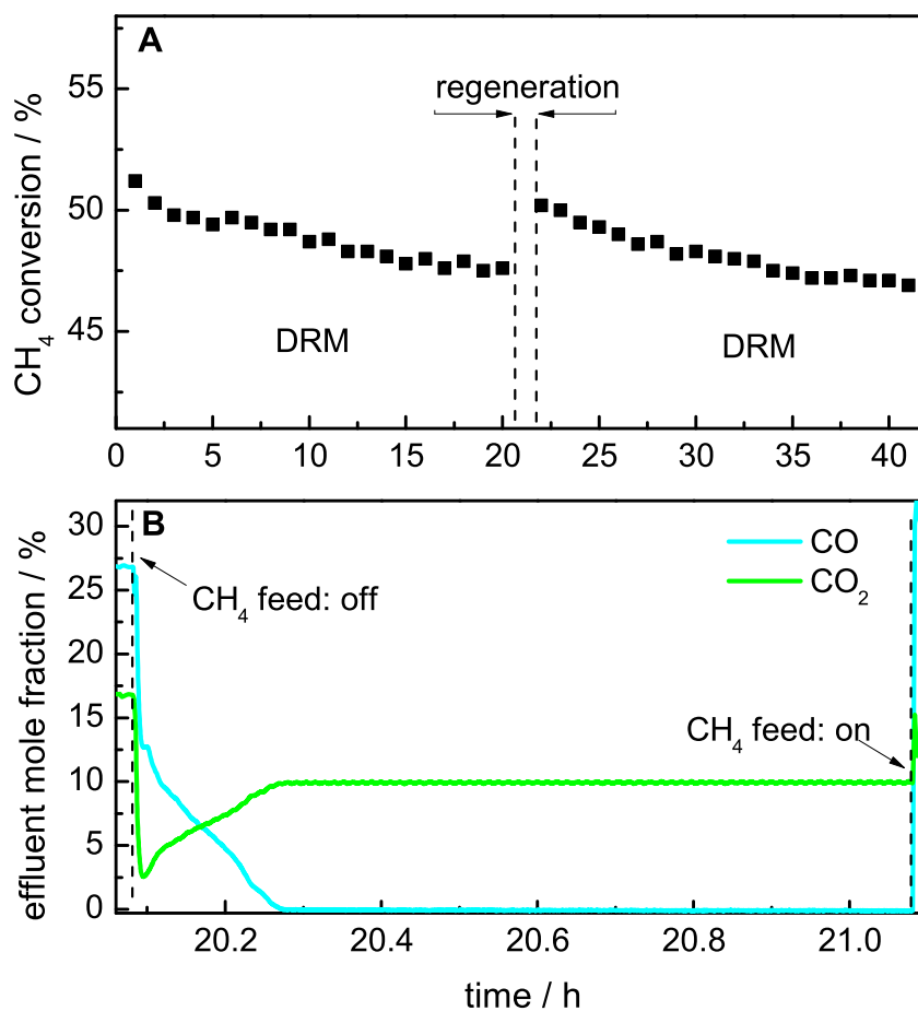
Figure 12: Isothermal regeneration with CO 2 of the 50 mol% Ni catalyst during DRM at 800 °C after thermal pre-treatment up to 800 °C, A) methane conversion in DRM as a function of time, B) effluent mole fraction of CO and CO 2 during the isothermal regeneration with 40 Nml min -1 of 10% CO 2 in Ar.
