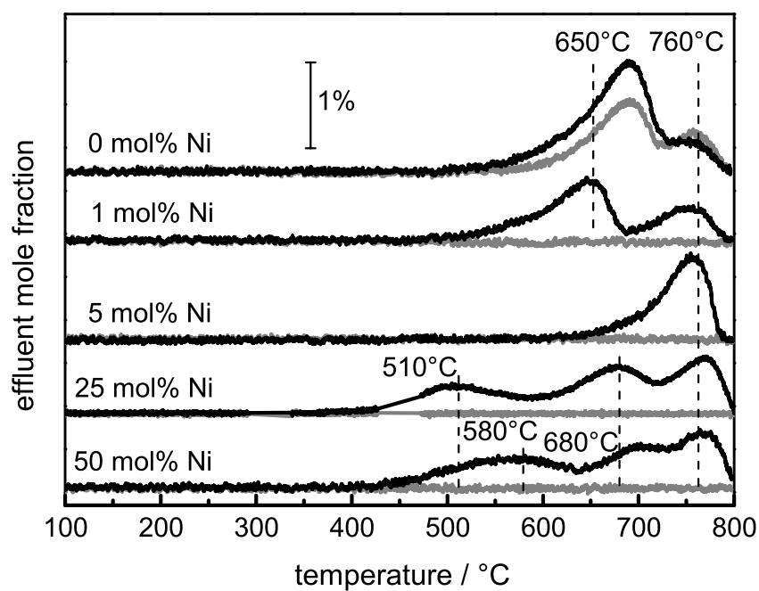
Figure 7: TPO profiles of all samples after 10 h of DRM at 900 °C. Effluent mole fraction of CO 2 (black) and CO (grey), heating with 5 °C min -1 up to 800 °C in a total flow of 20 Nml min -1 4.5% O 2 in Ar.
