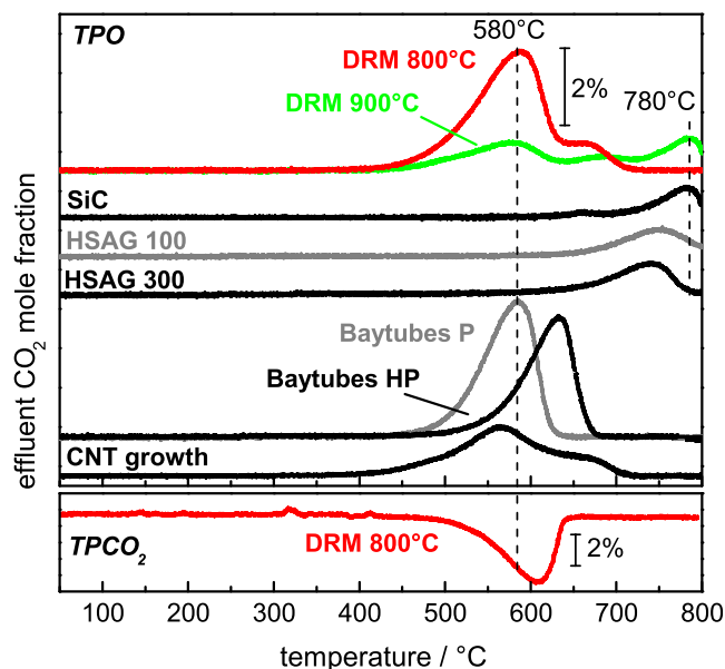
Figure 9: TPO profiles of 50 mol% Ni after DRM at 800 °C and 900 °C, of SiC after 10 h of DRM at 900 °C, following the CNT growth experiment using the 50 mol% Ni catalyst and of commercially available carbon for an assignment of the TPO peaks. The effluent mole fractions of CO 2 were detected while heating with 5 °C min -1 up to 800 °C in a total flow of 40 Nml min -1 4.5 % O 2 in Ar (top) or 10 % CO 2 in Ar (bottom).
