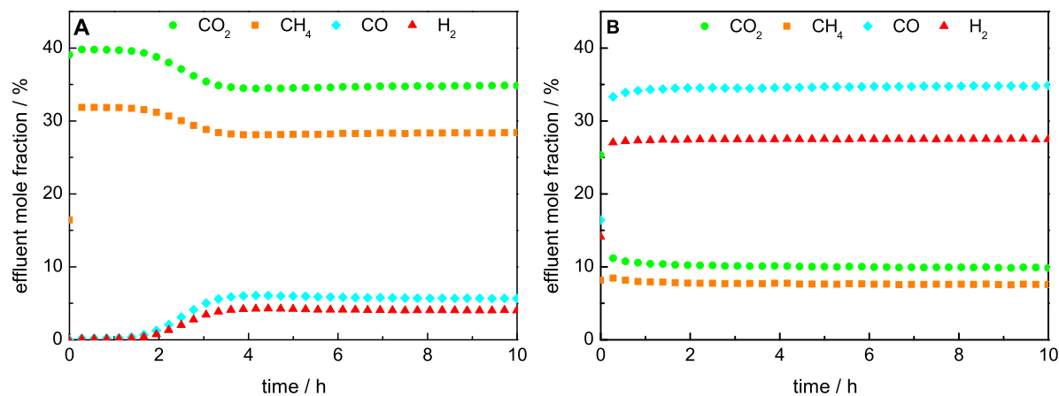
Figure 4: Effluent mole fraction during DRM at 900 °C in a total flow of 240 Nml min -1 consisted of 32% CH 4 and 40% CO 2 in Ar A) for the 1 mol% Ni, B) for the 50 mol% Ni catalyst.
