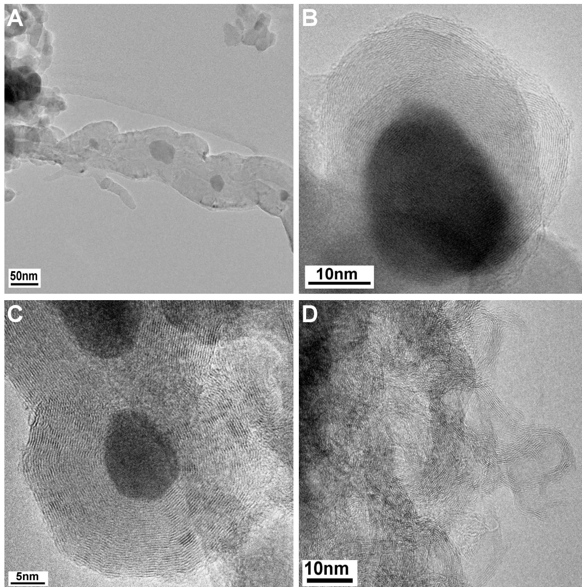
Figure 8: TEM micrographs after DRM of 50 mol% (A), 25 mol% (B), 5 mol% (C), 0 mol% (D) after 10 h of DRM at 900 °C in a total flow of 240 Nml min -1 and a composition of 32 % CH 4 and 40 % CO 2 in Ar.
