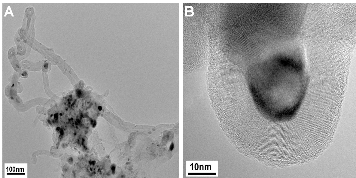
Figure 10: TEM micrographs after the CNT growth experiment using the 50 mol% Ni catalyst in a flow of 32 Nml min -1 CH 4 and 68 Nml min -1 H 2 at 680 °C. CNTs (left), graphite encapsulating Ni particles (right).
