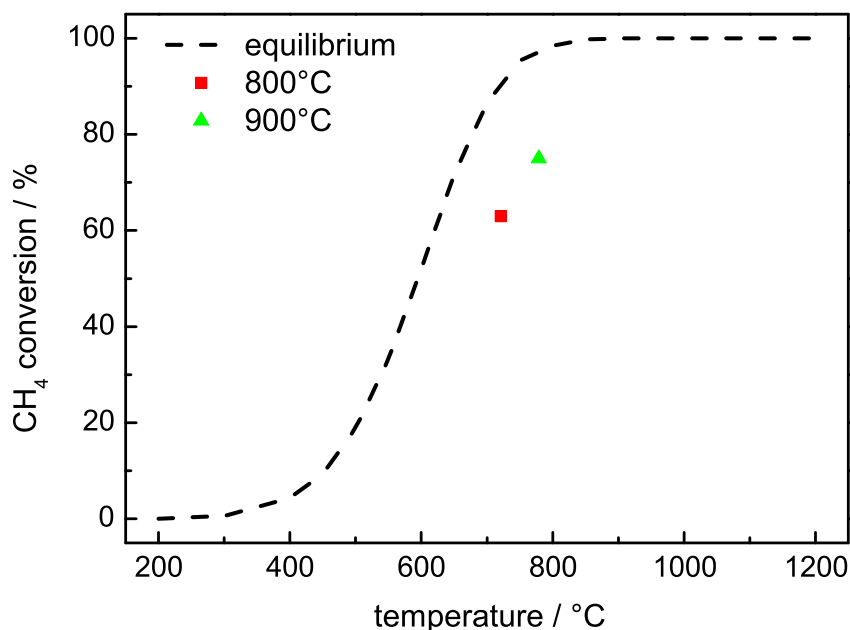
Figure 5: Comparison of experimental methane conversion over the 50 mol% Ni catalyst and equilibrium methane conversion in DRM. Equilibrium conversion was calculated using CHEMCAD and a feed composition of 32 % CH 4 , 40 % CO 2 and 28 % Ar.
