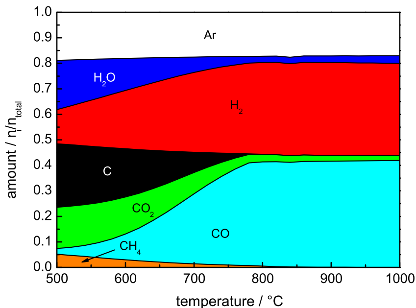
Figure 1: Calculated product distribution in thermodynamic equilibrium of 32 % \text{CH}_4 and 40 % \text{CO}_2 in Ar as a function of temperature considering the products C, \text{H}_2\text{O} , \text{CO}_2 , \text{CH}_4 , \text{H}_2 and CO. The calculations were based on a Gibbs free energy minimization implemented in CHEMCAD 6.4.2 by Chemstations.
