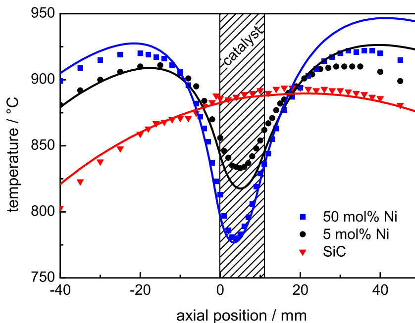
Figure 6: Measured axial temperature profiles (symbols) and corresponding simulated temperature profiles (lines). The catalyst bed is positioned between 0 and 11 mm using 10 mg of catalyst diluted in 490 mg SiC and a total flow rate of 240 Nml min -1 and a composition of 32 % CH 4 and 40 % CO 2 in Ar.
