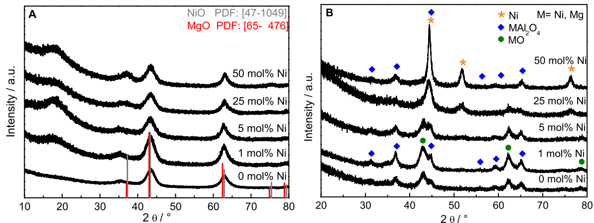
Figure 2: XRD patterns of the samples with different Ni contents A) after calcination of the htl precursor at 600 °C, B) after reduction at 1000 °C.
