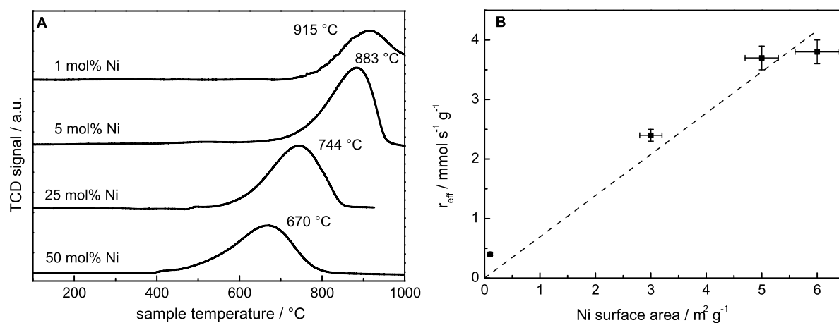
Figure 3: A) TPR profiles of the calcined samples with different Ni contents using 5% H 2 in Ar with a total flow of 80 Nml min -1 and a linear heating rate of 6 °C min -1 . B) Determined specific reaction rates during the DRM at 900 °C after reductive pre-treatment up to 1000 °C as a function of the specific Ni surface area. The accuracy of the measurements is estimated to be \pm 5\% in case of the average reaction rates and \pm 6\% for the specific Ni surface area.
