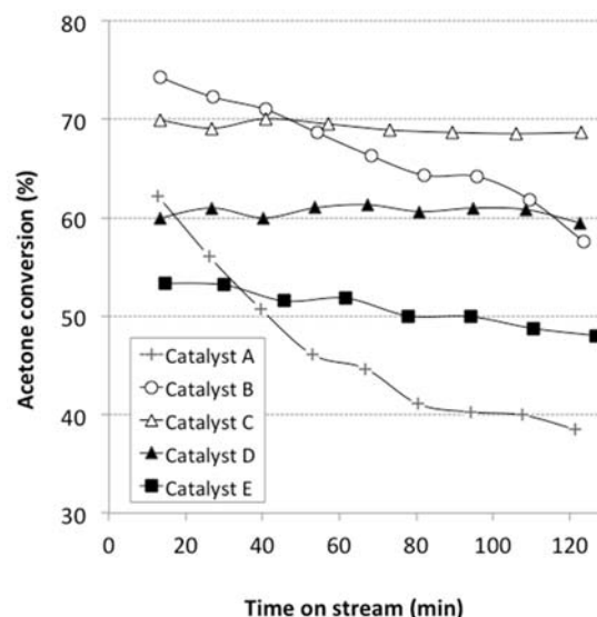
Fig. 2 Acetone conversion as a function of time on stream. Operating conditions: T = 200°C, P = 3 bar, WHSV = 1h -1 (1 g of catalyst, acetone = 1g/h), N 2 = 9L/h, H 2 = 1L/h. Conversion based on carbon weight.
