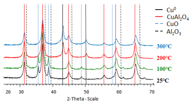
Figure 1 : XRD of Catalyst C after reducing 30 min at different temperature. Phases: CuO (ICDD n° 04-005-4712); CuAl 2 O 4 (ICDD n°04-015-0578); Cu 0 (ICDD n°04-003-1450); Al 2 O 3 (ICDD n°10-0425)
