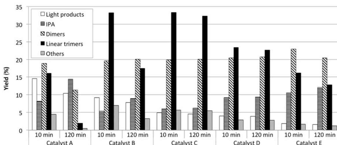
Fig.3 Yields of the main reaction products of acetone conversion after 10 and 120 min under time on stream for the various catalysts. Light products = propene, propane, cracking products; IPA = isopropanol; Dimers = MIBK, MIBA (4-methylpentan-2-ol), 2-MP (2-methylpentane) ; Linear trimers = DIBK, DIBA (2,6-dimethylheptan-4-ol) ; Others = TMB (1,3,5-trimethylbenzene), C 12 , unknown products. Operating conditions: T = 200°C, P = 3 bar, WHSV = 1h -1 (1 g of catalyst, acetone = 1g/h), N 2 = 9L/h, H 2 = 1L/h. Conversion based on carbon weight. Yields are based on carbon weight %. product distribution is given in the ESI section. The samples A and
