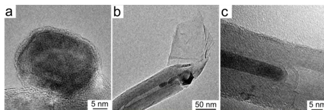
Fig. 8 TEM micrographs of CNT taken from the monolith surface showing a) exposed nanoparticles on the surface of the nanotube b) exposed nanoparticle at the end of the nanotube c) nanoparticles still enclosed by the nanotube
