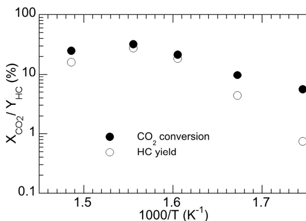
Fig. 5 Effect of temperature variation on CO 2 conversion. The reaction was performed at 7.5 bar over a 10 cm bed of Fe@CNT/monolith (synthesised at 790 °C for 60 minutes, approximately 0.15 g of Fe@CNT), temperature was varied from 300 to 400 °C.
