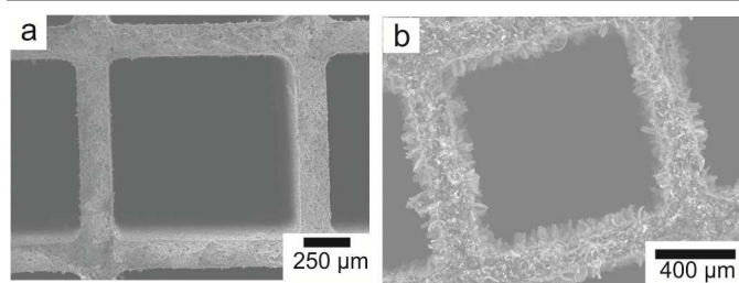
Fig. 1 SEM micrographs of a) bare cordierite monolith and b) cordierite monolith coated with CNT layer
