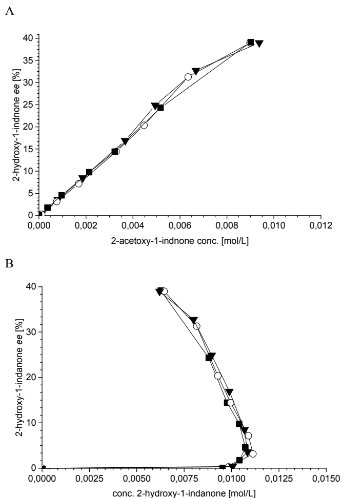
Figure 3. (A) enantiomeric excess ( ee = 100 \cdot \frac{[(R)\text{-}3] - [(S)\text{-}3]}{[(R)\text{-}3] + [(S)\text{-}3]} ) of 2-hydroxy-1-indanone versus concentration of 2-acetoxy-1-indanone in one-pot reactions using ■ 93 mg, ○ 130 mg and ▼ 163 mg lipase AK; (B) enantiomeric excess ( ee ) of 2-hydroxy-1-indanone versus 2-hydroxy-1-indanone concentration in one-pot reactions using ■ 93 mg, ○ 130 mg and ▼ 163 mg lipase AK.
