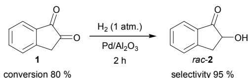
Scheme 2. Hydrogenation of 1 to rac - 2 with H 2 using Pd/Al 2 O 3 (2 mol-%) as the catalyst.
