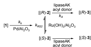
Scheme 6. One-pot reactions sequence including: i) hydrogenation of 1 ; ii) racemization of ( S )- 2 and ( R )- 2 ; iii) acylation of the formed ( R )- 2 with acyl donor forming ( R )- 3 .
