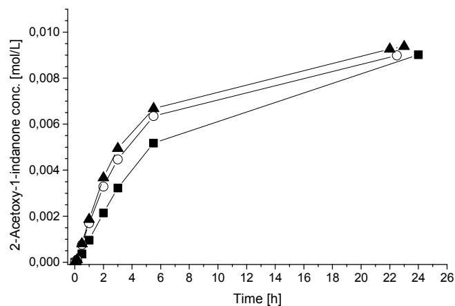
Figure 1. 2-Acetoxy-1-indanone concentration during the one-pot reactions using ■ 93 mg, ○ 130 mg and ▲ 163 mg of lipase AK, 51.6-51.9 mg Pd/Al 2 O 3 , 89.5-90.1 mg Ru(OH) 3 /Al 2 O 3 and 4 equivalents (550 μL) of the acyl donor 9 at 40 °C.
