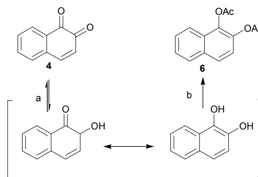
Scheme 3. Hydrogenation (a) and subsequent esterification (b) of 4 to 6 with H 2 (1 atm.) and Pd/Al 2 O 3 as catalyst.
