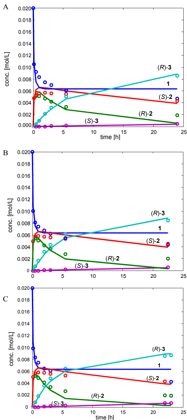
Figure 4. Comparison between the experimental data and the model predictions for the reactants in the three one-pot reactions using (A) 93 mg, (B) 130 mg and (C) 163 mg lipase AK. Solid lines represent the estimated data and circles the experimental data. The different compounds are represented by the following colors: blue compound 1, red (S)-2, green, (R)-2, cyan (R)-3, pink (S)-3. The degree of explanation 92.94 % and the standard errors of the parameters are acceptably low.
