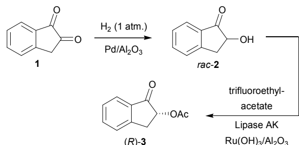
Scheme 1. One-pot reaction combining the regioselective hydrogenation of 1,2-indanedione ( 1 ) and chemoenzymatic dynamic kinetic resolution of the intermediate rac -2-hydroxy-1-indanone ( rac -2) producing ( R )-2-acetoxy-1-indanol [( R )- 3 ].
