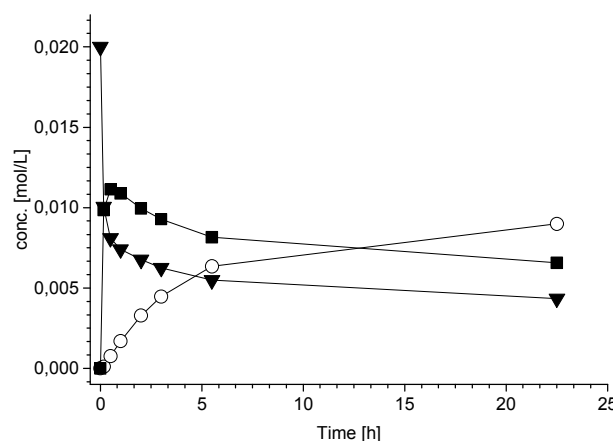
Figure 2. Concentration profiles of ▼ 1,2-indanedione, ■ 2-hydroxy-1-indanone, ○ 2-acetoxy-1-indanone for one-pot reaction using 51.6 mg Pd/Al 2 O 3 , 89.5 mg Ru(OH) 3 /Al 2 O 3 , 130 mg lipase AK and 4 equivalents (550 μL) of the acyl donor 9 at 40 °C.
