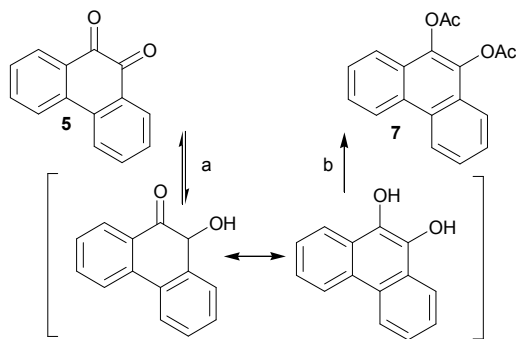
Scheme 4. Hydrogenation (a) and subsequent esterification (b) of 5 to 7 with H_2 (1 atm.) and Pd/Al_2O_3 as catalyst.
