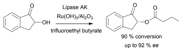
Scheme 5. DKR of rac - 2 using Ru(OH)_3/Al_2O_3 as the racemization catalyst in combination with lipase AK yielding ( R )-1-oxoindan-2-yl-butanoate with high ee 92 % and 90 % conversion. 8
