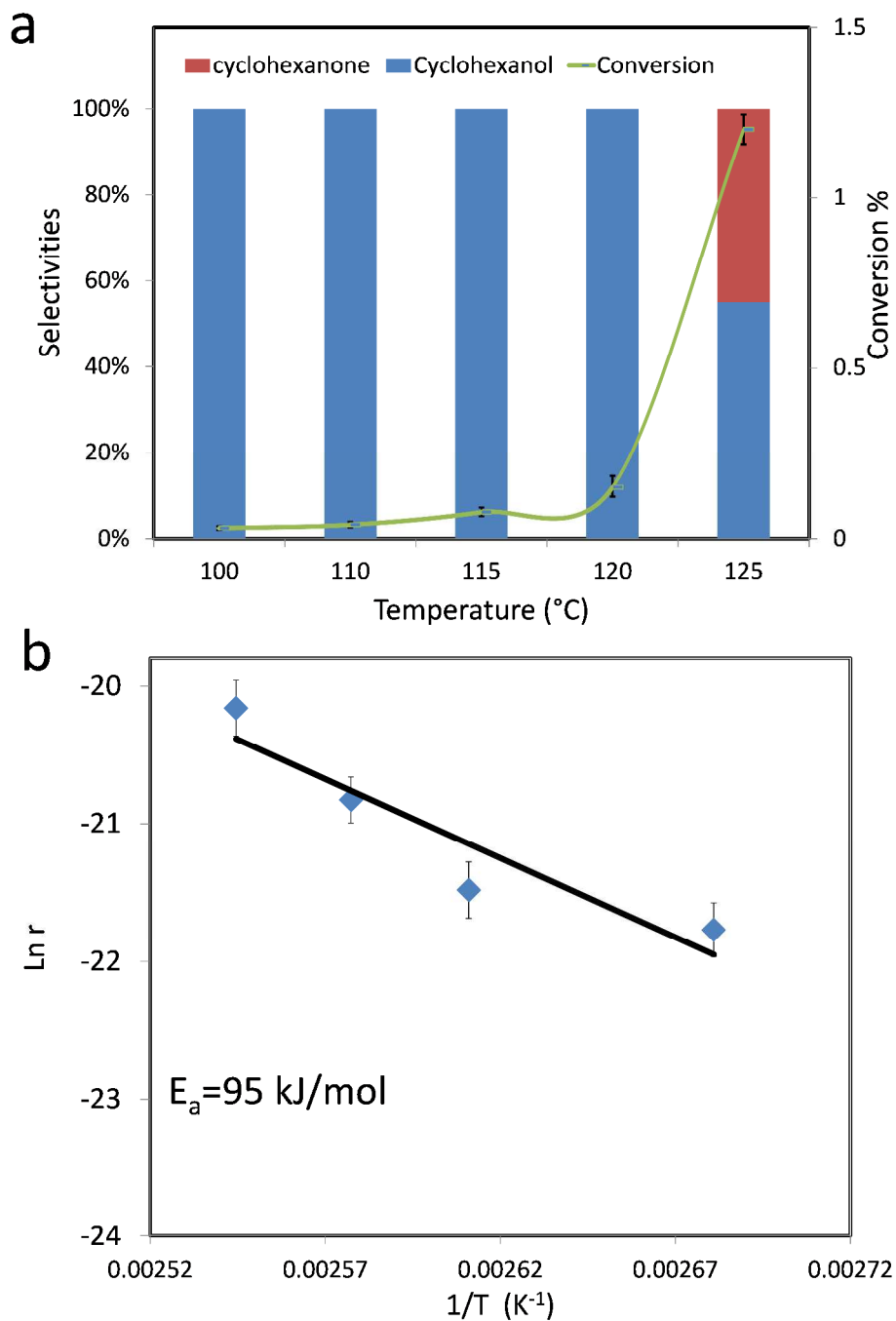
Figure 12. a) Catalytic performance of cyclohexane oxidation as a function of reaction temperature; b) Corresponding Arrhenius plot from 100°C to 120°C. Reaction conditions: 6 mg MB, 8.5 g cyclohexane, 3 bar O 2 , 24 h.
