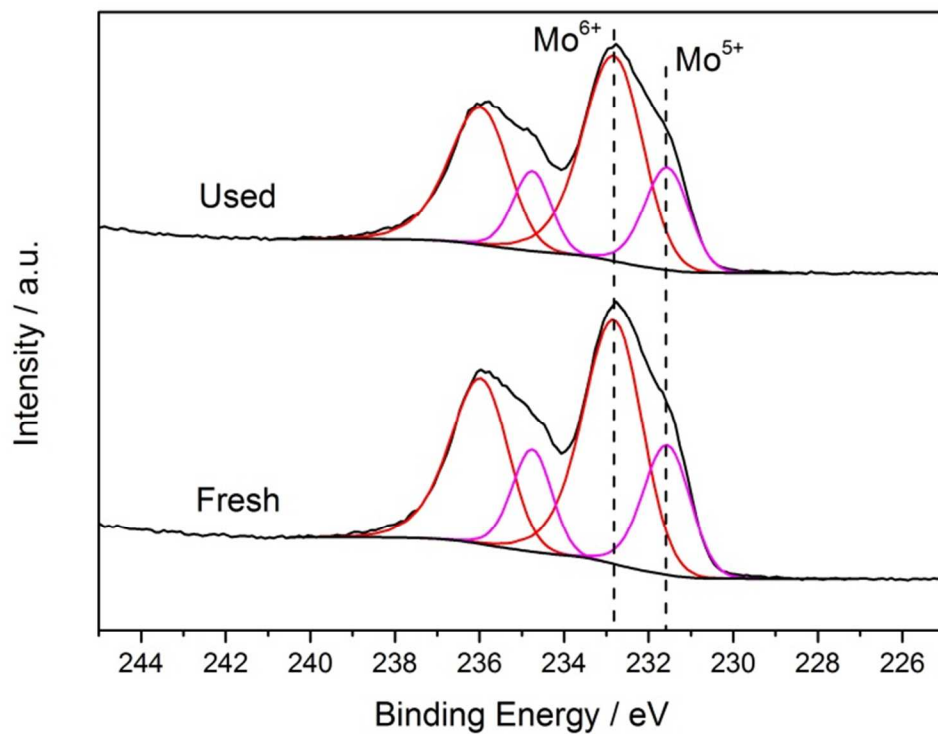
Figure 8. XPS profiles of fresh and used MB material; different Mo contributions are labelled with different colours. The relative fraction of Mo V cations present in the fresh and used MB remains constant at ~20%.
