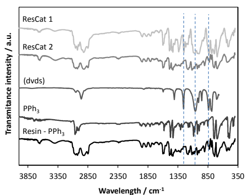
Figure 2: FTIR spectra of a. ResCat 1, b. ResCat 2, c. (dvds) from NIST database n. 2627-95-4, d. PPh 3 and e. Commercial triphenylphosphine-divinylbenzene copolymer (DVB) resin.
