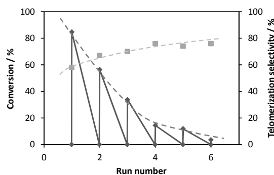
Figure 3: Reaction profile of consecutive telomerisation reactions of isoprene with methanol using ResCat 1 as catalyst.
