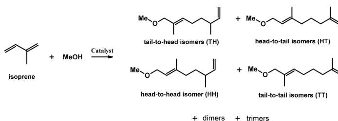
Figure 1: Potential products of telomerisation of isoprene with methanol.
