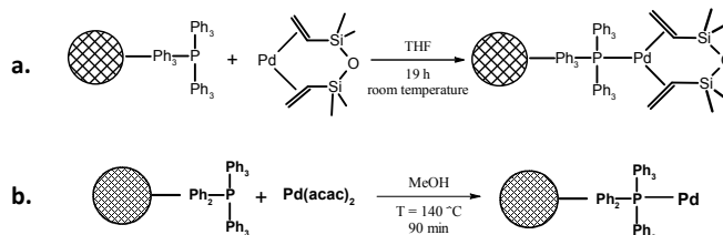
Figure 6: Synthesis of resin bound catalysts a. DVB-resin- \text{PPh}_3 -Pd-dvds (ResCat 1) and b. DVB-resin- \text{PPh}_3 -Pd (ResCat 2)
