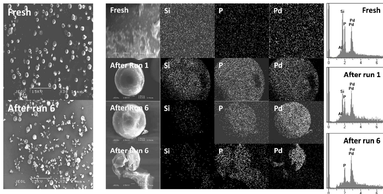
Figure 4: Scanning electron microscopy (SEM) and Energy dispersive X-ray spectroscopy (EDXS) elemental mapping of ResCat 1 catalysts fresh, after one catalytic run and after 6 catalytic runs.
