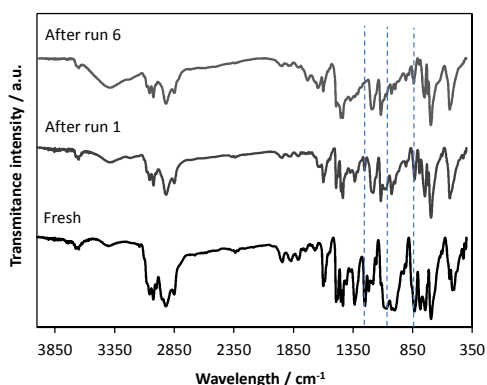
Figure 5: FTIR spectra of the ResCat 1 catalysts: fresh, after one and after six telomerisation recycling runs.
