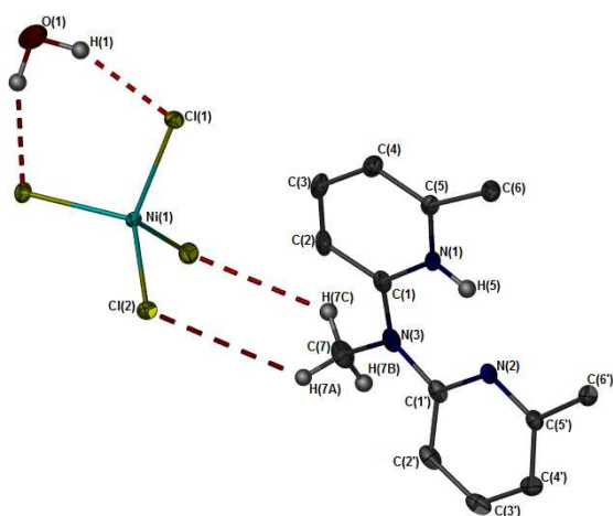
Fig. 2 Molecular structure of the crystals isolated as 1e-A , drawn at 50 % probability. Ni and O atoms located on a centre of inversion. Selected hydrogen atoms omitted for clarity.
