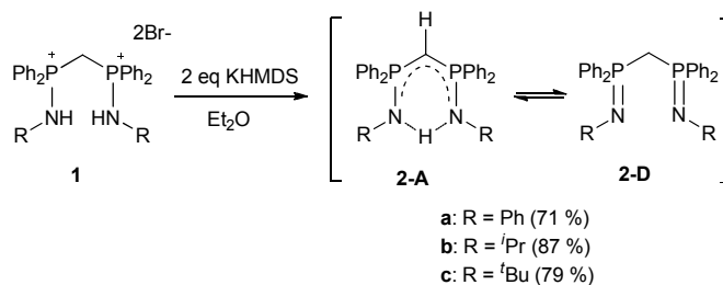
Scheme 1 Synthesis of BIP ligands 2a-c
