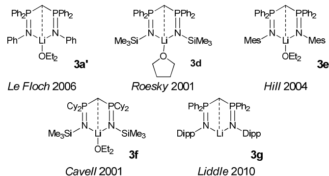
Fig. 4 Structurally characterised monomeric Li compounds 10, 15, 45–47
