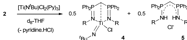
Scheme 2 Formation of BIPMH Ti-imido complexes 4
