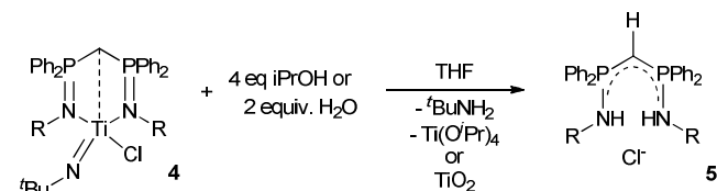
Scheme 6 Hydrolysis/alcoholysis of 4
