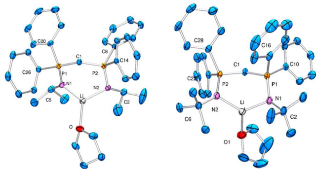
Fig. 3 POV-RAY depiction of 3b and 3c (thermal ellipsoids drawn at the 50 % probability level)
