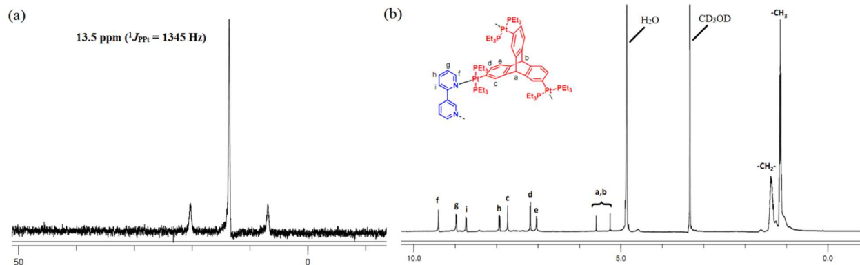
Figure 2: (a) ^{31}\text{P}\{^1\text{H}\} NMR and (b) ^1\text{H} NMR spectra of cage 5 in \text{CD}_3\text{OD}
