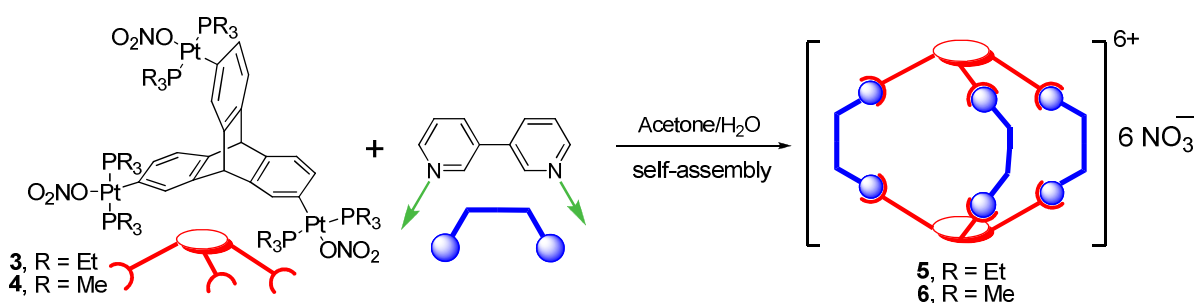
Scheme 3. Synthesis of metallasupramolecular cages 5 and 6
