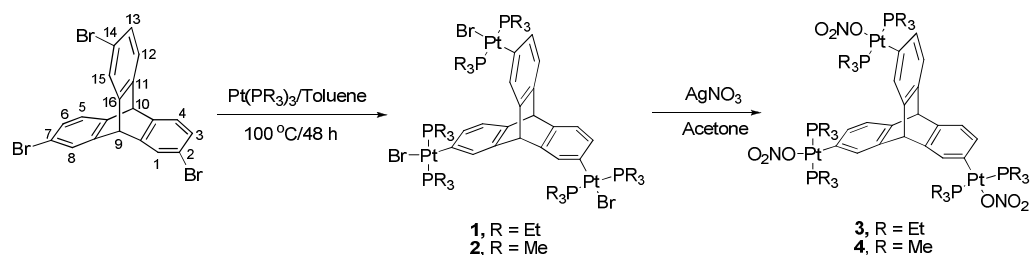
Scheme 1. Synthesis of triptycene based organoplatinum complexes ( 1-4 )
