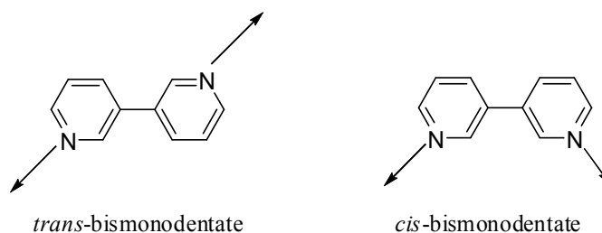
Scheme 2. cis - and trans - orientation of 3,3'-bipyridine as a bridging \mu -3,3'-bimonodentate ligand
