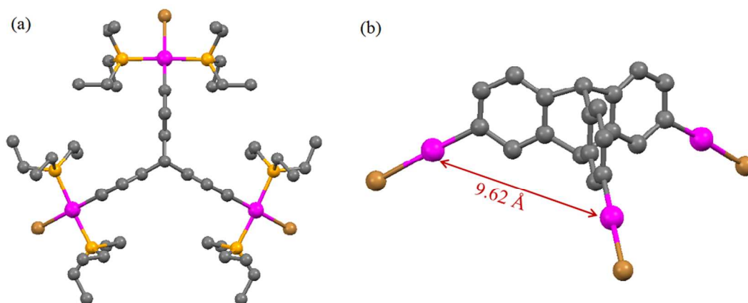
Figure 1. (a) Top view and (b) Side view (phosphine ligands are omitted) of crystal structure of complex 1 . Solvent molecules and hydrogen atoms are omitted for clarity (grey: C, pink: Pt, orange: P, brown: Br).
