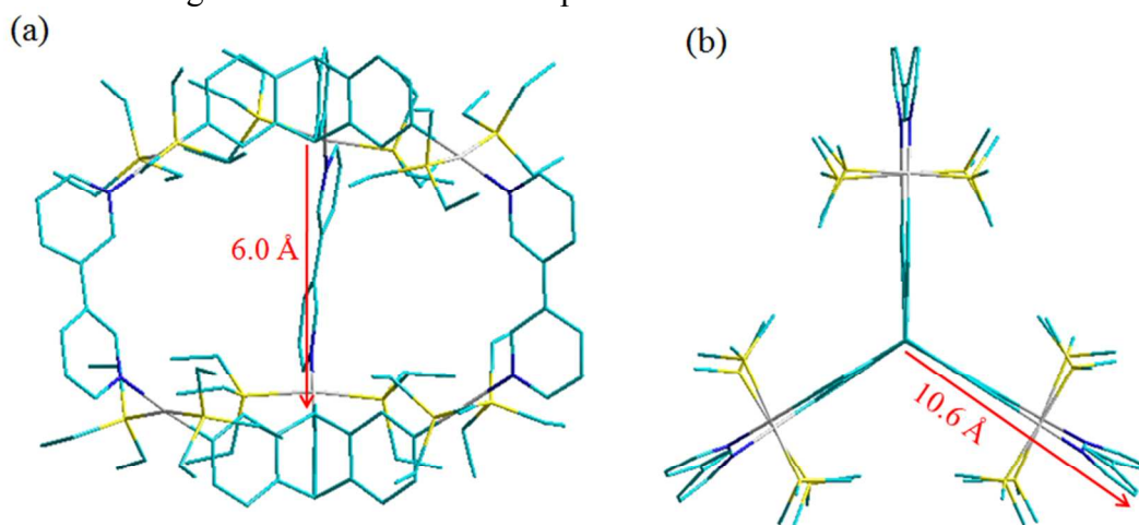
Figure 4: Simulated capped stick molecular model of (a) metallacage 5 and (b) metallacage 6 optimized by PM6 semiempirical molecular orbital methods (cyan: C, yellow: P, white: Pt, blue: N). H atoms are omitted for clarity.
