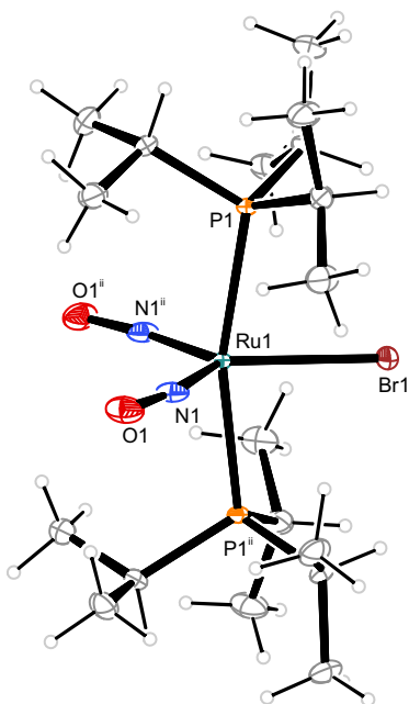
Fig. 11: Structure (50 % ellipsoids) of the TBPY-5 -type conformer 12b of the complex cation [\text{RuBr}(\text{NO})_2(\text{P}^i\text{Pr}_3)_2]^+ in crystals of 12 . Symmetry code: ^i -x + 1, y, -z + \frac{1}{2} .
