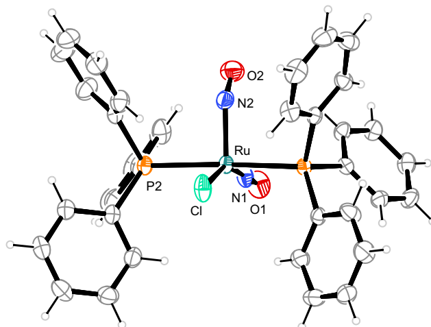
Fig. 5 Structure (50 % ellipsoids) of the vOC -5-type complex cation in crystals of [\text{RuCl}(\text{NO})_2(\text{PPh}_3)_2]\text{BF}_4 ( 1 ).
