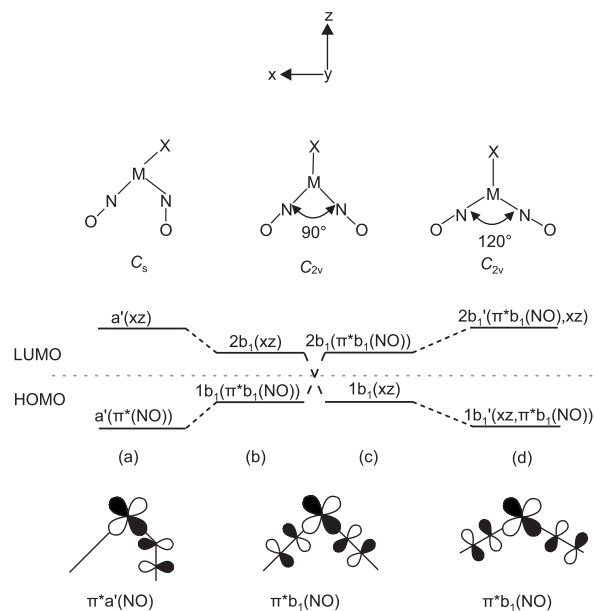
Fig. 17 Left: Correlation diagram showing the proposed behaviour of the 1b_1 and 2b_1 molecular orbitals in five-coordinate \{\text{M}(\text{NO})_2\}^8 complexes with a (1b_1)^2 electron configuration. Scheme (b) has \pi^*b_1(\text{NO}) lower in energy than d_{xz} and leads to structure (a). Scheme (c) has d_{xz} lower in energy than \pi^*b_1(\text{NO}) and leads to (d). Adapted from Ref. 2 . Right: The relevant orbital ( xz , \pi^*b_1(\text{NO}) ) which is metal-ligand non-bonding at an N-M-N angle of 90^\circ .
