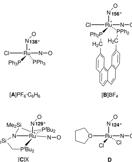
Fig. 2 Known \{\text{Ru}(\text{NO})_2\}^8 dinitrosyls (charges are drawn at the central metal atom); several publications deal with salts of A , including a tetrafluoroborate with a ^{14}\text{NO}/^{15}\text{NO} couple. 15, 17-19 The "X" in [C] X is [\text{Ru}(\text{NO})(\text{OH})(\text{NO}_2)_2\text{Cl}_2] . 20-22 Ru-N-O angles are given for the bent RuNO moiety.
