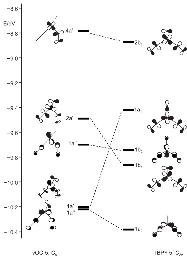
Fig. 18 Schematic representation of selected frontier orbitals for the C_{2v} ( TBPY-5 ) and the C_s ( vOC-5 ) conformer of 12 calculated by a DFT-based method.
