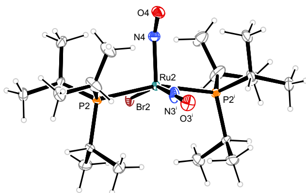
Fig. 12: Structure (50 % ellipsoids) of the vOC-5 -type conformer 12a of the complex cation [\text{RuBr}(\text{NO})_2(\text{P}^i\text{Pr}_3)_2]^+ in crystals of 12 . Symmetry code: ^i -x, y, -z + \frac{1}{2} . The linear NO group and the Br ligand are disordered in such a way as to be superimposed onto each other. The bent NO group is also disordered in such a way to ensure that the O4 atom is always inclined to the linear NO group. This kind of disorder corresponds to crystallographic mm2 site symmetry of the cations.
