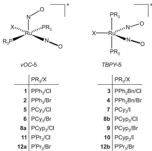
Fig. 4: The crystalline compounds of this work and their structure type (charges omitted). The abbreviations TBPY -5 and vOC -5 refer to IUPAC's configuration index and the definitions used by the Alvarez group in the context of Continuous Shape Measures (CShM) . 23
