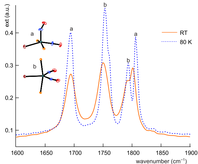
Fig. 15 IR spectrum of the ground state of 12a/b in the \nu(NO) range at RT (solid line) and 80 K (dashed line).
