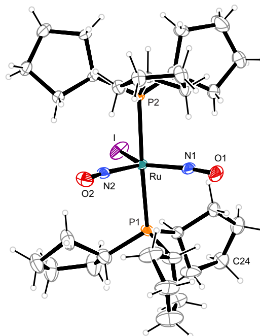
Fig. 10: Structure (50 % ellipsoids) of the TBPY-5-type complex cation [\text{RuI}(\text{NO})_2(\text{PCyp}_3)_2]^+ in crystals of 10 . C24 is disordered, the minor part (34%) is not shown.
