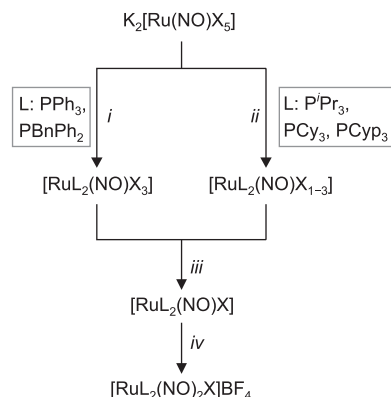
Fig. 3 Synthetic route to the [\text{RuL}_2(\text{NO})_2\text{X}]\text{BF}_4 dinitrosyls of this work. The employed phosphanes differ by their electronic and steric properties as given by their Tolman's parameters ( \nu in \text{cm}^{-1} and cone angle): triphenylphosphane ( \text{PPh}_3 ) 2068.9, 145^\circ ; benzyldiphenylphosphane ( \text{PBnPh}_2 ) 2068.4, 152^\circ ; trisopropylphosphane ( \text{P}^i\text{Pr}_3 ) 2059.2, 160^\circ ; tricyclohexylphosphane ( \text{PCy}_3 ) 2056.4, 170^\circ ; no values were available for tricyclopentylphosphane ( \text{PCyp}_3 ). Details of the individual steps: i 2.5 – 3 eq. L, EtOH/ \text{H}_2\text{O} ; ii 2.5 – 4 eq L, EtOH/ \text{H}_2\text{O} ; iii Zn, Cu, toluene; iv (\text{NO})\text{BF}_4 , toluene/EtOH. In the ii step, partial reduction of the Ru species by the more electron rich phosphanes took place prior to the final reduction step iii , hence the [\text{RuL}_2(\text{NO})\text{X}_{1-3}] formulation. Further details are collected in the Experimental Section.
