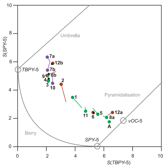
Fig. 14 Shape map for pentacoordinate complex ions [Ru(NO)_2(PR_3)_2X]^+ . The graph was drawn by using Fig. 6 of Ref. 23 as a template (from which the commentary printed in grey was transferred as well). Purple (X = I), reddish brown (X = Br) and green (X = Cl) circles are drawn at the experimental values; lines of the respective colour end at the DFT-calculated values; small black circles within larger coloured circles indicate that the DFT value gave a data point within the experimental value's circle radius.
