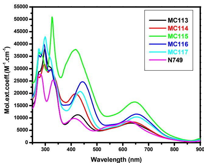
Fig. 2: Absorption Spectra of MC113-MC117 and N749 in DMF solution
