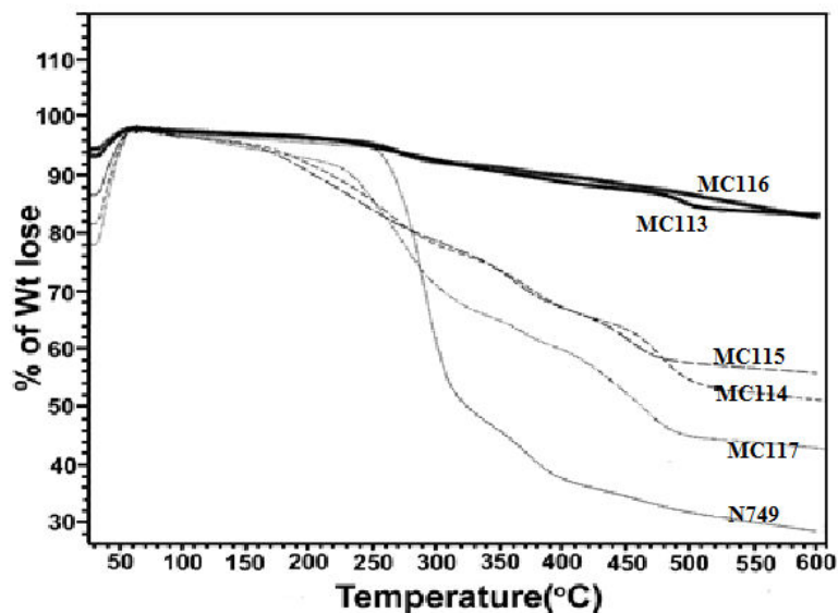
Fig. 4: Thermograms of the sensitizers MC113-MC117 relative to N749 .
