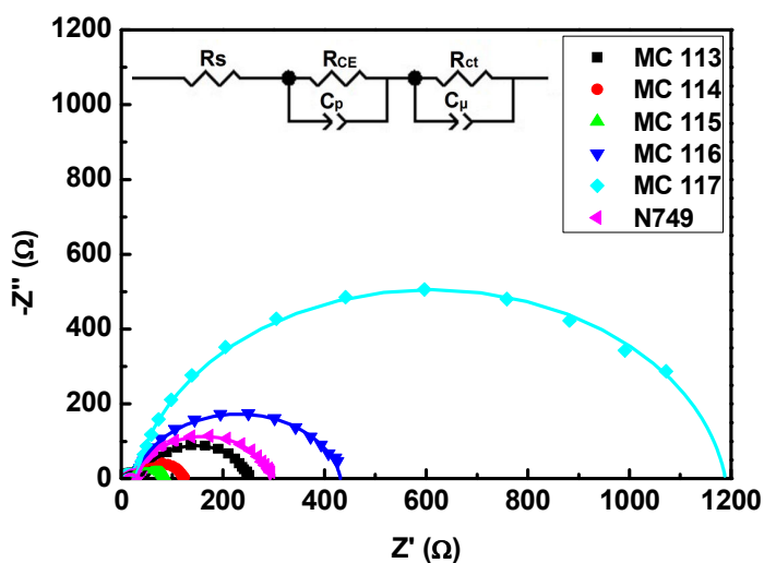
Fig. 7: EIS Nyquist plots for DSSCs based on MC113-MC117 sensitizers and N749 dye (measured under dark conditions with an external potential of -0.60 V. The inset shows the equivalent circuit).
