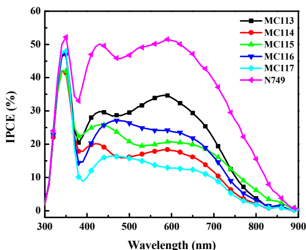
Fig. 5: Photocurrent action (IPCE) curves of the \text{TiO}_2 electrodes sensitized by MC113-MC117 and standard N749 .
