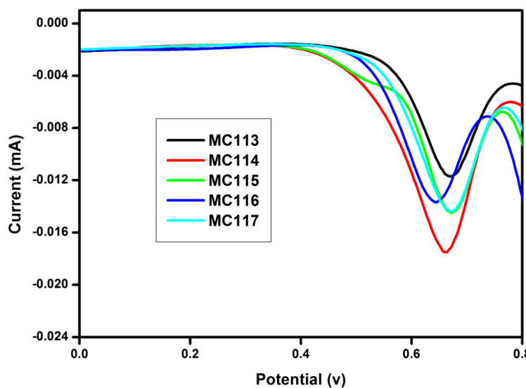
Fig. 3a: Oxidative Defferential Pulse Voltammetry of MC113-MC117
