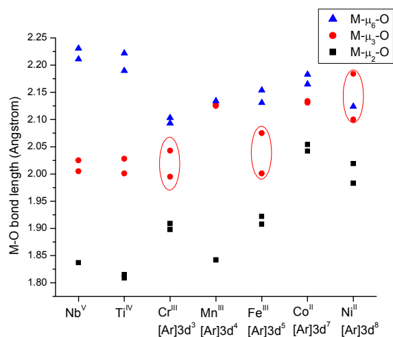
Fig. 3 The central M-O bond lengths in decaniobate and TM-substituted decaniobates. X-axis shows corresponding central atoms and their electron configurations.
