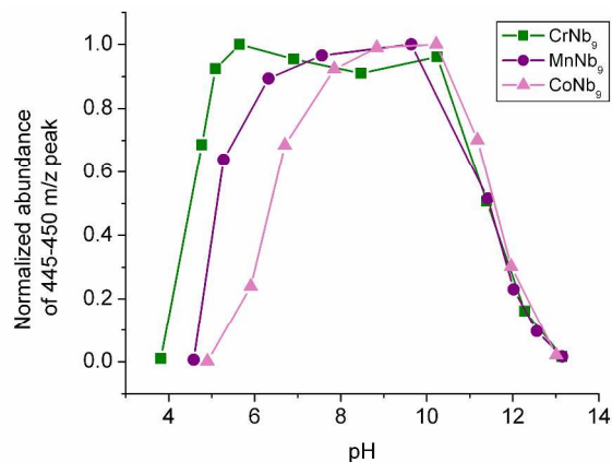
Fig. 4 Normalized peak intensity (strongest peak) in ESI-MS of 1-3 as a function of pH, based on Figures S1-S3
