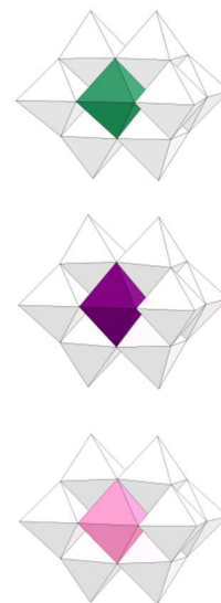
Fig. 1 Polyhedral model of MNB 9 clusters (M=Cr III , Mn III and Co II , from top to bottom) in 1-3 (white: Nb, green: Cr, purple: Mn, pink: Co).
