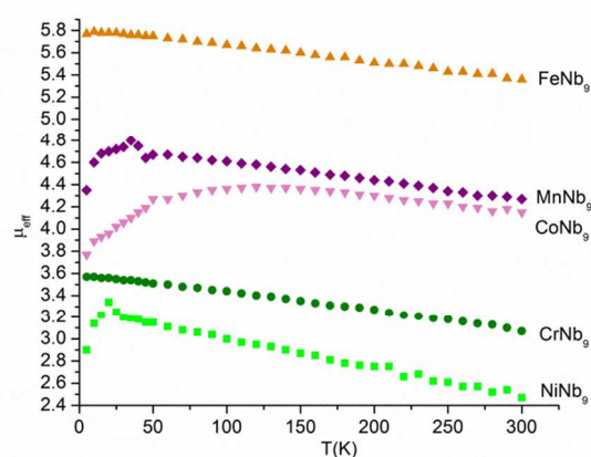
Fig. 5 \mu_{\text{eff}} vs Temperature for TMA salts of TM-substituted decaniobates.
