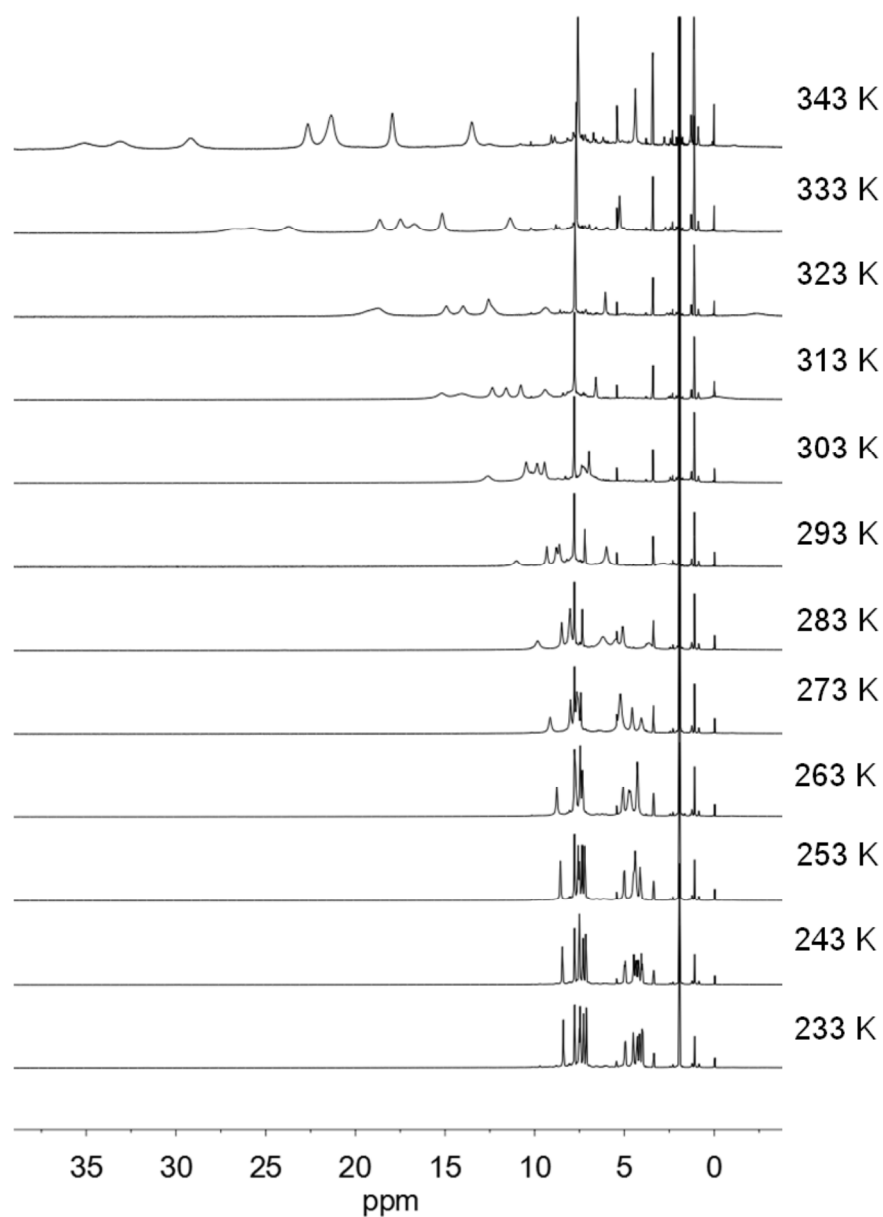
Figure 7. VT- ^1\text{H} NMR spectra of [\text{Fe}(\mathbf{5})(\text{OTf})](\text{OTf}) in \text{CD}_3\text{CN} .
