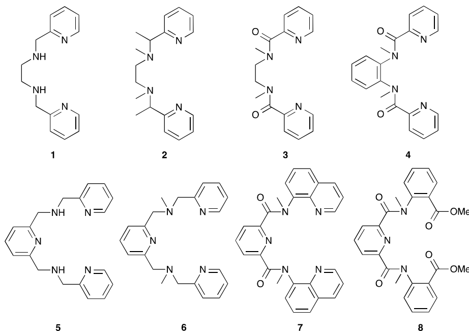
Figure 1. Overview of tetradentate and pentadentate pyridylmethylamine ligands ( 1 – 8 ).
