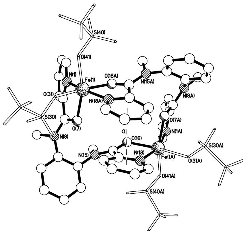
Figure 4. The crystal structure of the C_2 -symmetric complex [\text{Fe}(\mathbf{4})(\text{OTf})_2]_2 . Selected bond lengths ( \text{\AA} ) and angles ( ^\circ ); Fe(1)–N(1) 2.1674(15), Fe(1)–O(7) 2.1769(13), Fe(1)–O(31) 2.0948(13), Fe(1)–O(41) 2.1100(14), Fe(1)–O(16A) 2.0964(11), Fe(1)–N(18A) 2.1632(14), N(1)–Fe(1)–O(7) 75.19(5), N(1)–Fe(1)–O(31) 102.84(5), N(1)–Fe(1)–O(41) 88.85(6), N(1)–Fe(1)–O(16A) 86.60(5), N(1)–Fe(1)–N(18A) 161.27(5), O(7)–Fe(1)–O(31) 88.21(5), O(7)–Fe(1)–O(41) 161.14(5), O(7)–Fe(1)–O(16A) 94.02(5), O(7)–Fe(1)–N(18A) 99.13(5), O(31)–Fe(1)–O(41) 85.60(6), O(31)–Fe(1)–O(16A) 170.56(5), O(31)–Fe(1)–N(18A) 94.70(5), O(41)–Fe(1)–O(16A) 94.98(5), O(41)–Fe(1)–N(18A) 99.12(6), O(16A)–Fe(1)–N(18A) 75.90(5).
