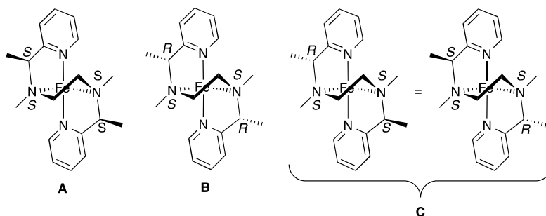
Figure 3. Four of eight possible isomers for complex [\text{Fe}(\mathbf{2})(\text{OTf})_2] with cis- \alpha geometry (the OTf ligands have been omitted for clarity).
