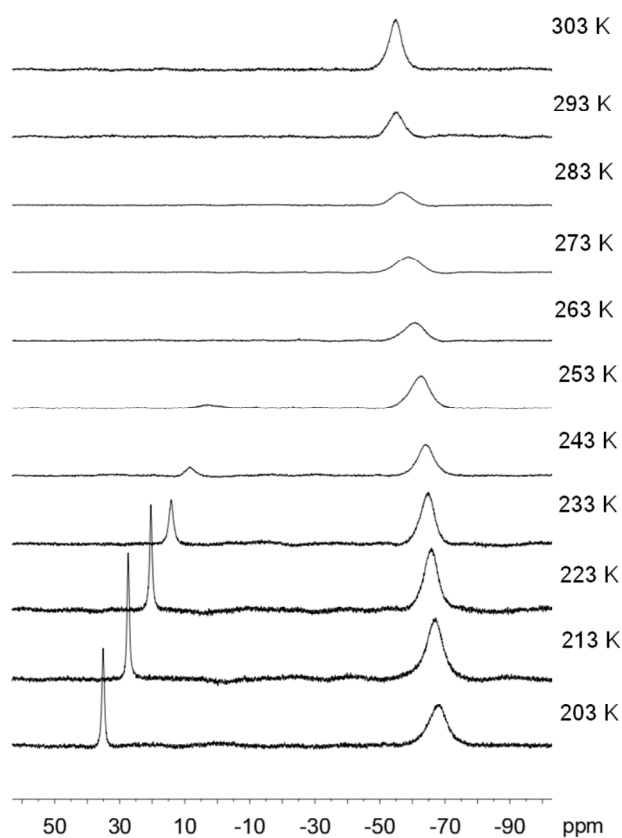
Figure 6. VT- ^{19}\text{F} NMR spectra of [\text{Fe}(\mathbf{5})(\text{OTf})](\text{OTf}) in \text{CD}_2\text{Cl}_2 from 203 to 303 K.
