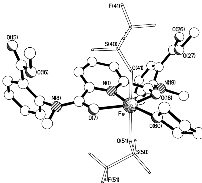
Figure 8. The crystal structure of [\text{Fe}(\mathbf{8})(\text{OTf})_2(\text{thf})] . Selected bond lengths (Å) and angles ( ^\circ ); Fe–N(1) 2.1259(14), Fe–O(7) 2.1139(12), Fe–O(18) 2.1178(13), Fe–O(41) 2.147(2), Fe–O(51) 2.1081(15), Fe–O(60) 2.091(3), N(1)–Fe–O(7) 74.00(5) , N(1)–Fe–O(18) 74.69(5) , N(1)–Fe–O(41) 93.66(9) , N(1)–Fe–O(51)
