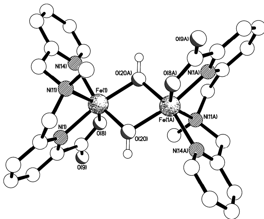
Figure 9. The structure of the C_2 -symmetric di-cation present in the crystal of [\text{Fe}(\mathbf{6}')(\text{OH})_2(\text{OTf})_2] . Selected bond lengths ( \text{\AA} ) and angles ( ^\circ ); Fe(1)–N(1) 2.085(2), Fe(1)–O(8) 1.9728(19), Fe(1)–N(11) 2.247(2), Fe(1)–N(14) 2.111(2), Fe(1)–O(20) 1.9664(17), Fe(1)–O(20A) 1.9700(17), N(1)–Fe(1)–O(8) 77.75(8), N(1)–Fe(1)–N(11) 73.70(8), N(1)–Fe(1)–N(14) 102.22(9), N(1)–Fe(1)–O(20) 93.18(8), N(1)–Fe(1)–O(20A) 169.40(8), O(8)–Fe(1)–N(11) 147.17(8), O(8)–Fe(1)–N(14) 93.70(9), O(8)–Fe(1)–O(20) 103.97(8), O(8)–Fe(1)–O(20A) 101.79(8), N(11)–Fe(1)–N(14) 77.08(8), N(11)–Fe(1)–O(20) 93.55(8), N(11)–Fe(1)–O(20A) 109.25(8), N(14)–Fe(1)–O(20) 158.72(9), N(14)–Fe(1)–O(20A) 88.38(8), O(20)–Fe(1)–O(20A) 76.60(8), Fe(1)–O(20)–Fe(1A) 103.40(8).
