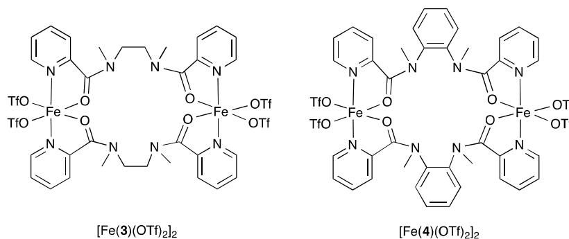
Figure 5. Molecular structures of iron(II) bis(triflate) complexes of ligands 3 and 4 .
