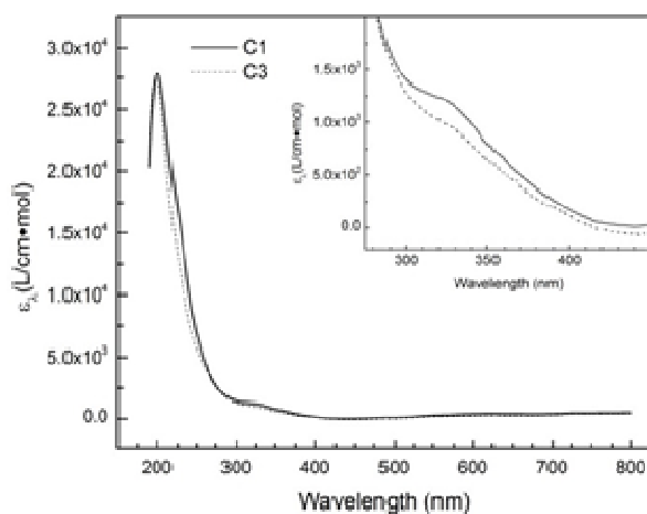
Fig. 4 UV-vis absorption spectra of aqueous C1 and C3 . Both species exhibit a strong charge transfer band ( \epsilon_{\max} \sim 200 nm) having a weak leading shoulder (inset).
