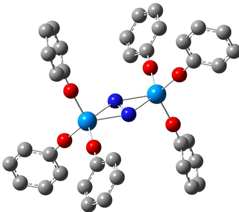
Figure 2: Ball and stick image of the optimised geometry of [\text{U}(\text{OPh})_3]_2(\mu\text{-}\eta^2\text{:}\eta^2\text{-N}_2)^{58} . Hydrogen atoms omitted for clarity.
