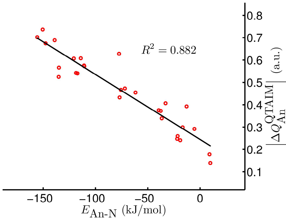
Figure 5: |\Delta Q_{\text{An}}^{\text{QTAIM}}| vs E_{\text{An-N}} for [\text{AnX}_3]_2(\mu\text{-}\eta^2\text{:}\eta^2\text{-N}_2) (An = Th–Pu; X = F, Cl, Br, Me, H). Data for [\text{Np}(\text{OPh})_3]_2(\mu\text{-}\eta^2\text{:}\eta^2\text{-N}_2) not included.
