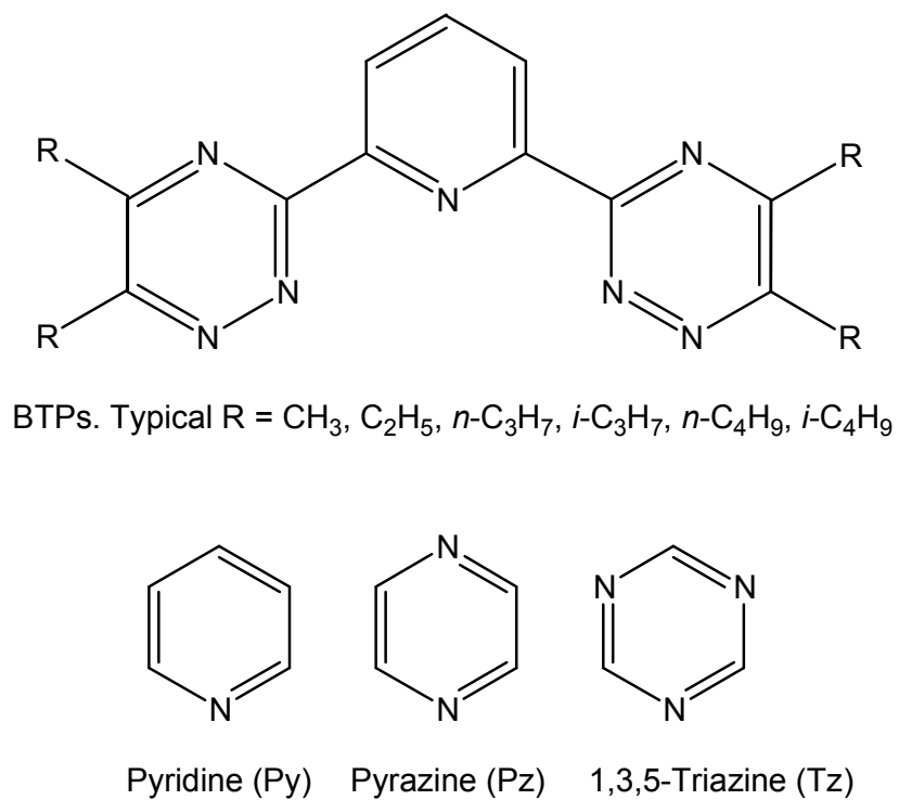
Figure 1: 2,6-bis(triazinyl)-pyridines (BTPs, upper) and the three L type nitrogen-donor ligands (lower).
