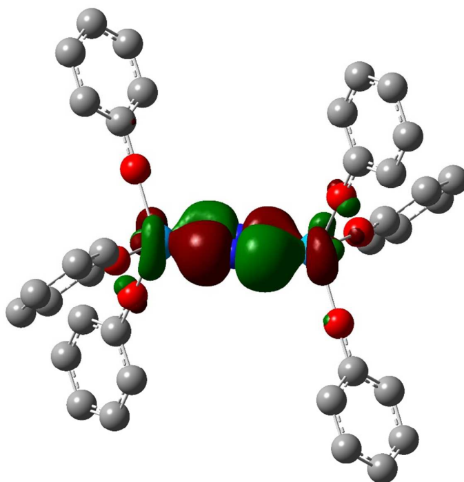
Figure 4: Three dimensional representations of the \alpha HOMO-8 (a) and \alpha HOMO-1 (b) molecular orbitals of [\text{Pa}(\text{OPh})_3]_2(\mu\text{-}\eta^2\text{:}\eta^2\text{-N}_2) . Isovalue = 0.04. Hydrogen atoms omitted for clarity. Orbital compositions (Mulliken analysis, %) are 18% Pa f, 12% Pa d, 50% N p and 22% Pa f, 8% Pa d, 68% N p respectively.
