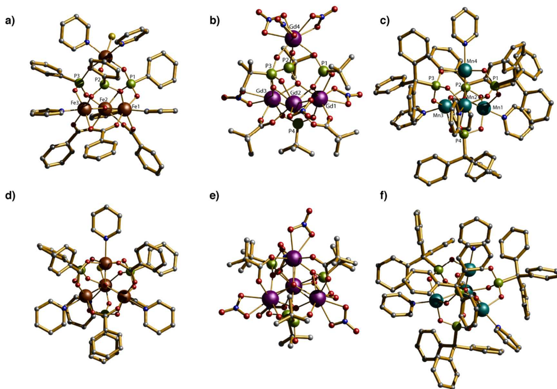
Figure 4. (a) and (d) side and top view of crystal structure of the \{\text{Fe}_4\text{P}_4\} cluster; (b) and (e) side and top view of Crystal structure of the \{\text{Ln}_4\text{P}_4\} cluster; (c) and (f) side and top view of Crystal structure of the \{\text{Mn}_4\text{P}_4\} cluster; Scheme: Ln, purple; Fe, brown; Mn, cyan; P, green; O, red; C, grey; N, cyan; (H omitted for clarity).
