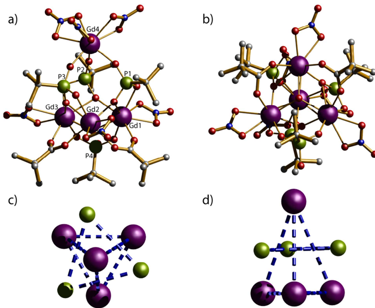
Figure 1. (a) and (b) side and top view of Crystal structure of the \{Gd_4P_4\} cluster. Scheme: Ln, purple; P, green; O, red; C, grey; N, cyan; (H omitted for clarity); (c) and (d) top and side view of metal and phosphonate core of the crystal structure of \{Gd_4P_4\} cluster.
