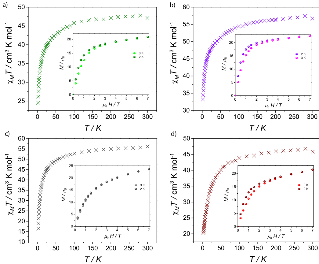
Figure 2. Molar magnetic susceptibility ( \chi_M T ) vs. T plot for 2–5 under 1 kG dc field and molar magnetization ( M ) as a function of applied magnetic field ( H ) at 2 and 3 K (inset) for a) 2, b) 3, c) 4 and d) 5.
