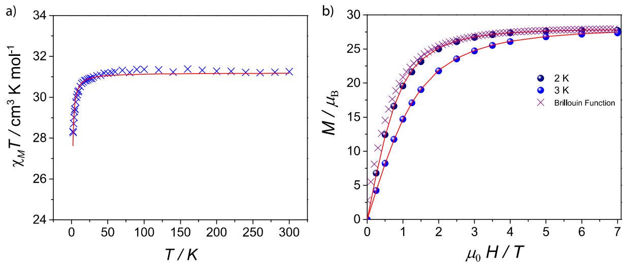
Figure 3. (a) Molar magnetic susceptibility ( \chi_M T ) vs. T and simulation plots for 1 under 1 kG dc field; (b) Molar magnetization ( M ) as a function of applied magnetic field ( H ) at 2 and 3 K for 1.
