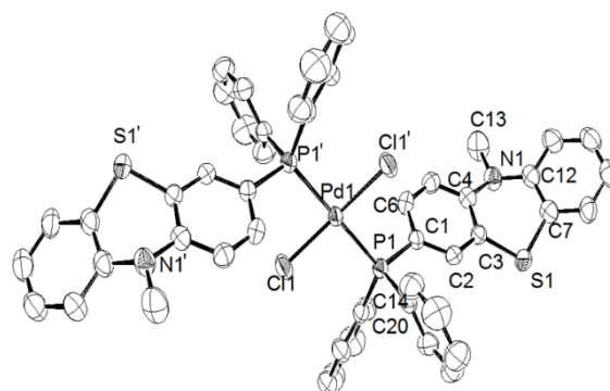
Fig. 5 ORTEP drawing of 10 . Thermal ellipsoids are drawn at 50% probability. Hydrogen atoms are omitted for clarity. Selected bond lengths (Å) and angles (°): Pd(1)–P(1) 2.3233(8), Pd(1)–P(1') 2.3233(8), Pd(1)–Cl(1) 2.2878(9), Pd(1)–Cl(1') 2.2878(9), P(1)–C(1) 1.811(3), P(1)–C(14) 1.813(3), P(1)–C(20) 1.825(3), S(1)–C(3) 1.759(3), S(1)–C(7) 1.759(3), N(1)–C(13) 1.464(4), N(1)–C(4) 1.404(4), N(1)–C(12) 1.414(4), P(1)–Pd(1)–P(1') 180.0(3), P(1)–Pd(1)–Cl(1) 91.55(3), Cl(1)–Pd(1)–Cl(1') 180.0, C(1)–P(1)–C(14) 105.6(1), C(1)–P(1)–Pd(1) 114.0(1), C(14)–P(1)–Pd(1) 110.3(1), C(14)–P(1)–C(20) 103.6(2), C(3)–S(1)–C(7) 98.9(2), C(4)–N(1)–C(12) 119.6(3), C(4)–N(1)–C(13) 117.0(3), P(1)–C(1)–C(2) 122.1(2).
