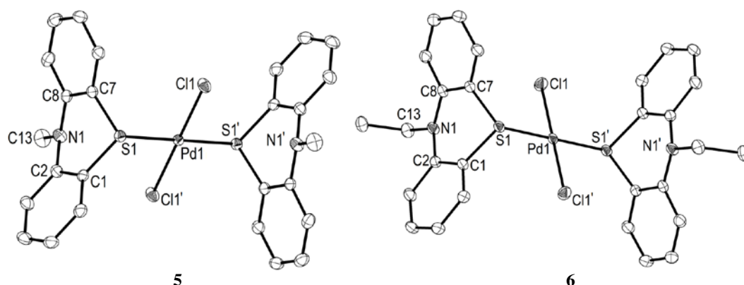
Fig. 2 Molecular structures of complexes 5 and 6 . Thermal ellipsoids are drawn at 50% probability. All hydrogen atoms are omitted for clarity. Selected bond lengths (Å) and angles (°) for 5 : Pd(1)–Cl(1) 2.3083(6), Pd(1)–S(1) 2.3267(6), S(1)–C(7) 1.770(2), S(1)–C(1) 1.756(2), N(1)–C(2) 1.396(3), N(1)–C(8) 1.395(3), N(1)–C(13) 1.452(3), Cl(1)–Pd(1)–S(1) 84.35(2), Cl(1')–Pd(1)–S(1) 95.65(2), C(1)–S(1)–C(7) 99.00(1), Pd(1)–S(1)–C(7) 103.06(8), Pd(1)–S(1)–C(1) 111.26(8), C(2)–N(1)–C(8) 119.3(2), C(8)–N(1)–C(13) 119.2(2); for 6 : Pd(1)–Cl(1) 2.2921(5), Pd(1)–S(1) 2.3338(5), S(1)–C(7) 1.749(2), S(1)–C(1) 1.761(2), N(1)–C(2) 1.400(2), N(1)–C(8) 1.401(2), N(1)–C(13) 1.472(2), C(13)–C(14) 1.528(3), Cl(1)–Pd(1)–S(1) 95.36(2), Cl(1')–Pd(1)–S(1) 84.64(2), C(1)–S(1)–C(7) 98.32(9), Pd(1)–S(1)–C(7) 110.19(7), Pd(1)–S(1)–C(1) 106.76(7), C(2)–N(1)–C(8) 120.4(2), C(8)–N(1)–C(13) 118.1(2).
