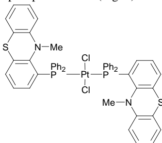
Fig. 4 Proposed structure for complex 9
