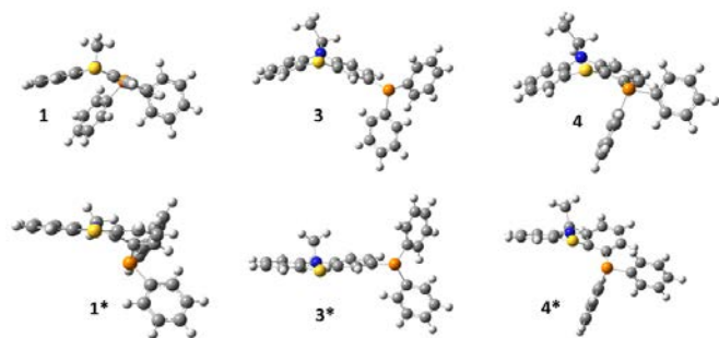
Fig. 1 Optimised geometries for 1 , 3 , 4 and their first excited singlet states ( 1* , 3* , 4* ), viewed along the N-S axis (N: blue, S: yellow, P: orange).
