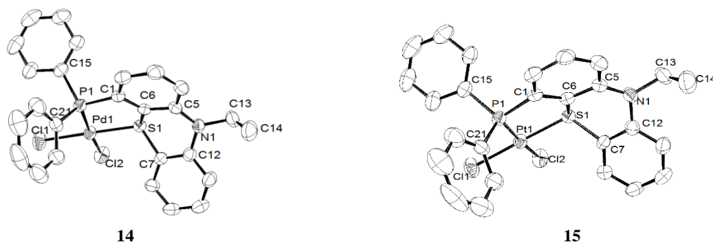
Fig. 6 Molecular structures of complexes 14 and 15 . Thermal ellipsoids are drawn at 50% probability. Hydrogen atoms are omitted for clarity. Selected bond lengths (Å) and angles (°) for 14 : Pd(1)–Cl(1) 2.310(1), Pd(1)–P(1) 2.2236(9), Pd(1)–S(1) 2.2575(8), Pd(1)–Cl(2) 2.3552(9), S(1)–C(6) 1.764(3), S(1)–C(7) 1.783(3), P(1)–Pd(1)–S(1) 88.21(3), P(1)–Pd(1)–Cl(1) 88.47(3), P(1)–Pd(1)–Cl(2) 173.69(4), Cl(1)–Pd(1)–Cl(2) 94.62(4), C(1)–P(1)–C(15) 107.4(2), C(1)–P(1)–Pd(1) 107.1(1), C(21)–P(1)–Pd(1) 114.9(1), C(15)–P(1)–C(21) 106.7(2), C(1)–P(1)–C(21) 105.0(2), C(6)–S(1)–Pd(1) 105.4(1), C(7)–S(1)–Pd(1) 114.3(1), C(6)–S(1)–C(7) 96.15(1), C(1)–C(6)–S(1) 121.0(2); for 15 : Pt(1)–Cl(1) 2.313(2), Pt(1)–P(1) 2.215(1), Pt(1)–S(1) 2.239(1), Pt(1)–Cl(2) 2.357(2), S(1)–C(6) 1.767(5), S(1)–C(7) 1.791(5), P(1)–Pt(1)–S(1) 88.71(5), P(1)–Pt(1)–Cl(1) 90.10(5), P(1)–Pt(1)–Cl(2) 174.69(6), Cl(1)–Pt(1)–Cl(2) 91.94(6), C(1)–P(1)–C(15) 107.4(3), C(1)–P(1)–Pt(1) 107.1(2), C(21)–P(1)–Pt(1) 115.4(2), C(15)–P(1)–C(21) 105.7(3), C(1)–P(1)–C(21) 105.5(2), C(6)–S(1)–Pt(1) 105.4(2), C(7)–S(1)–Pt(1) 114.3(2), C(6)–S(1)–C(7) 95.7(2), C(1)–C(6)–S(1) 120.7(4).
