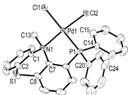
Fig. 3 Molecular structure of complex 7 . Thermal ellipsoids are drawn at 50% probability. Hydrogen atoms are omitted for clarity. Selected bond lengths (Å) and angles (°): Pd(1)–N(1) 2.161(1), Pd(1)–P(1) 2.1829(5), Pd(1)–Cl(2) 2.2936(4), Pd(1)–Cl(1) 2.3925(5), N(1)–C(1) 1.473(2), N(1)–C(7) 1.479(2), N(1)–C(13) 1.519(2), N(1)–Pd(1)–P(1) 86.18(4), P(1)–Pd(1)–Cl(2) 86.99(2), N(1)–Pd(1)–Cl(1) 94.68(4), P(1)–Pd(1)–Cl(1) 176.74(2), Cl(2)–Pd(1)–Cl(1) 92.44(2), C(12)–P(1)–C(14) 105.52(9), C(14)–P(1)–C(20) 108.01(9), C(12)–P(1)–Pd(1) 102.51(7), C(14)–P(1)–Pd(1) 119.60(6), C(20)–P(1)–Pd(1) 113.02(7), C(1)–N(1)–Pd(1) 117.70(1), C(7)–N(1)–Pd(1) 112.50(1), C(13)–N(1)–Pd(1) 98.90(1).
