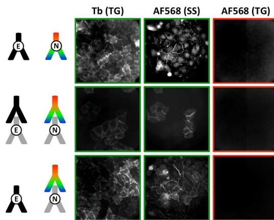
Figure 6: TG (0.01 - 2.51 ms after excitation pulse) and SS (excited at 520\pm 14 nm) images in the Tb detection channel (Tb, 542\pm 10 nm) and the AF568 detection channel (AF568, 607\pm 5 nm) of different FRET-pair antibody combinations to detect a possible E/N cadherin clustering. Costaining of Tb-antibodies (against E-cadherin) and AF568-antibodies (against N-cadherin) is clearly visible in the TG Tb and SS AF568 PL images. However, no FRET signal (TG AF568 signal) is detected, which shows that Tb-donor and dye-acceptor are not in close ( < ca. 12 nm) proximity. For better clarity, positive signal images have green frames whereas negative signal images have red frames. Control experiments using FITC, AF647, AF488, and AF594 antibodies against N-cadherin as acceptors and different primary/secondary antibody combinations led to the same results ( Figures S8 to S10 in the ESI).
