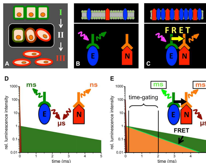
Figure 1: Schematic presentations of EMT ( A , cells in epithelial (I), intermediate (II) and mesenchymal (III) state) and the distinction between E-cadherin and N-cadherin coexpression ( B and D ) and E/N-cadherin clustering ( C and E ) by TG FRET using Tb-donor antibody (green) excitation (magenta arrow) and dye-acceptor antibody (orange) emission (orange arrow). D: When E- and N-cadherins are not in a close distance (>20 nm) UV-excitation of the immunostained cells leads to long-lifetime Tb PL (green), a strong nano- to microsecond autofluorescence (brown) and a weak short-lived (nanoseconds) acceptor PL. E: Clustering of E- and N-cadherins brings the Tb-donor and dye-acceptor in close proximity, which causes Tb-to-dye FRET. As the FRET efficiency \eta_{\text{FRET}} = 1 - (\tau_{\text{DA}}/\tau_{\text{D}}) , 23 FRET leads to millisecond Tb and dye emission (light green and orange, respectively) that is shorter than the pure Tb PL decay time. TG detection of the FRET quenched Tb-donor PL and FRET-sensitized dye-acceptor PL intensities several microseconds after the excitation pulse leads to specific PL signals for E/N clustering.
