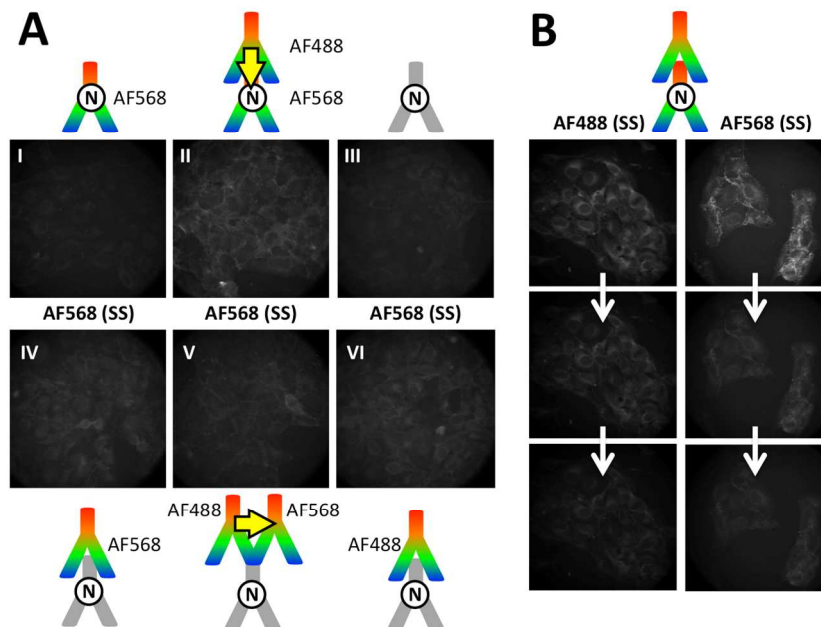
Figure 7: A: SS images of different combinations of AF488 donor antibodies with AF568 acceptor antibodies on M4-T cells were recorded in the AF568 PL emission channel upon excitation of AF488 ( 438\pm 12 nm, no significant direct excitation of AF568). Although the two possible AF488-AF568 FRET combinations (II and V) led to positive PL signals, the dye-dye FRET pair could not provide clear evidence for FRET because direct excitation of AF568 (I and IV), spectral crosstalk of AF488 PL in the AF568 detection channel (VI), and autofluorescence of immunostained cells without any dyes (III) also led to positive PL signals. Control experiments using specific excitation of only AF488 antibodies and AF568 antibodies confirmed that both dye-labelled antibodies were bound to the cell membranes ( Figure S12 in the ESI). B: Strong photobleaching (three serial image acquisitions from top to bottom) of both AF488 (excitation via 438\pm 12 nm and detection via 522\pm 6 nm transmission filters, 100 ms acquisition per image) and AF568 (excitation via 542\pm 10 nm and detection via 607\pm 5 nm transmission filters, 350 ms acquisition per image) with both dye-labelled antibodies against N-cadherin or with only one type of each dye-labelled antibody ( Figure S11 in the ESI).
