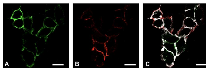
Figure 2: Confocal images of A549 cells, which coexpress E-cadherin (A, FITC dye) and N-cadherin (B, AlexaFluor594 dye). The overlay image (C) shows colocalization (indicated by the white pixels) with Mander's overlap coefficients of M1 = 0.95 (fraction of AF594 pixels overlapping FITC pixels) and M2 = 0.48 (fraction of FITC pixels overlapping AF594 pixels) but does not contain any information about the E-N cadherin distances (E/N cadherin clusters). Scale bars correspond to 20 μm.
