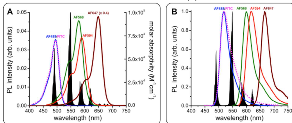
Figure 4: PL emission spectrum of Tb (black in A and B) and absorbance (A) and PL emission (B) spectra of FITC (magenta), AF488 (blue), AF568 (green), AF594 (red), and AF647 (brown, molar absorptivity spectrum in A multiplied by 0.4 for better visibility of all spectra). Förster distances of the different FRET pairs were calculated using equations 1 and 2: R_0(\text{Tb-FITC}) = 4.9 \text{ nm} , R_0(\text{Tb-AF488}) = 4.9 \text{ nm} , R_0(\text{Tb-AF568}) = 6.1 \text{ nm} , R_0(\text{Tb-AF594}) = 5.9 \text{ nm} , R_0(\text{Tb-AF647}) = 5.9 \text{ nm} , and R_0(\text{AF488-AF568}) = 6.2 \text{ nm} .
