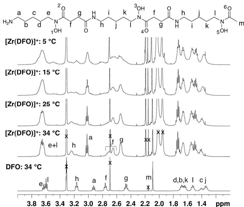
Figure 3: Variable temperature ^1\text{H} NMR spectra in of DFO and [\text{Zr}(\text{DFO})]^+ in methanol- d_4 . Additional resonances in [\text{Zr}(\text{DFO})]^+ spectra result from excess [\text{Zr}(\text{acac})_4] , acac, mesylate ion, acetone and solvent. In the case where chemically inequivalent atoms have the same label, the similar chemical environment of the atoms resulted in coincident resonances at 500 MHz for ^1\text{H} NMR, and coincident, or almost coincident resonances at 100 MHz (on a Bruker Avance 400 spectrometer) for ^{13}\text{C} NMR.
