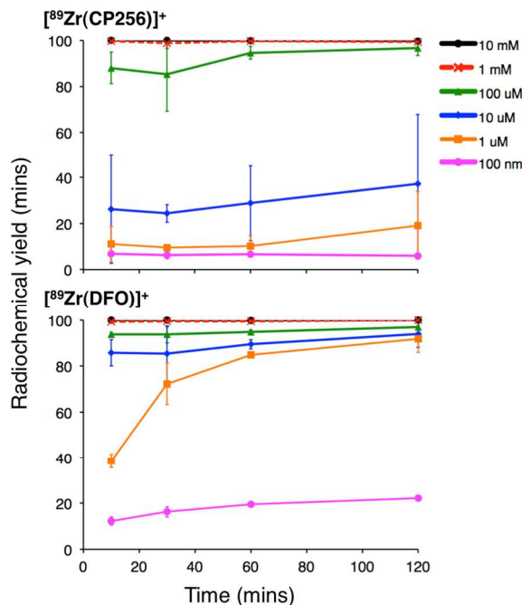
Figure 5: Radiochemical yield of [ ^{89}\text{Zr}(\text{CP256}) ] ^{+} (top) and [ ^{89}\text{Zr}(\text{DFO}) ] ^{+} (bottom) at different concentrations of chelator over the course of two hours. Error bars correspond to one standard deviation.
