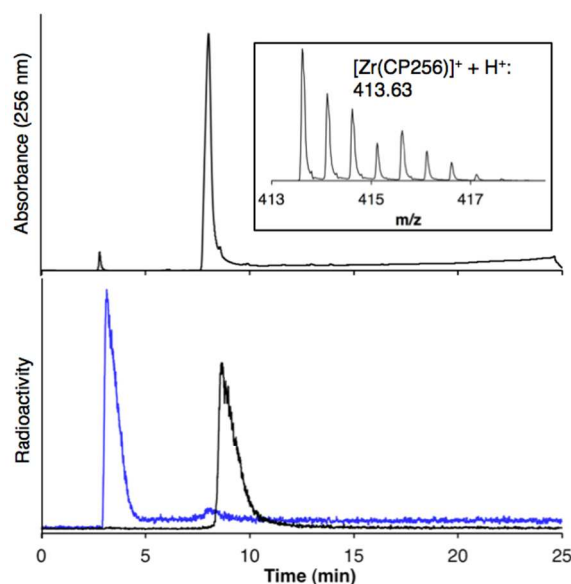
Figure 1: LCMS of [Zr(CP256)] + . Top: HPLC chromatogram with UV detection at λ 256 of [Zr(CP256)] + and corresponding MS signal (inset) of the fraction eluting at 8.0 min; Bottom: HPLC chromatogram of [ 89 Zr(CP256)] + (8.61 min) (black trace) and [ 89 Zr(ox) 4 ] 4- (blue trace) with radio-scintillation detection. Difference in retention times for the same species between UV and radio-scintillation HPLC chromatograms is a result of the configuration of the detectors in series.
