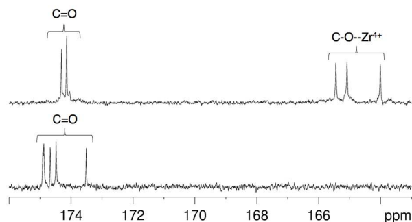
Figure 4: ^{13}\text{C} NMR spectra in of [\text{Zr}(\text{DFO})]^+ (top) and DFO (bottom) in methanol- d_4 at 25 °C, demonstrating the shift in ^{13}\text{C}=\text{O} resonances upon \text{Zr}^{4+} coordination.
