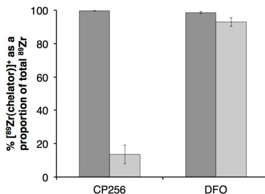
Figure 7: Stability of ^{89}\text{Zr}^{4+} complexes of \text{H}_3\text{CP256} (left) and \text{H}_3\text{DFO} (right): (■) % radiochemical yield of [\text{}^{89}\text{Zr}(\text{chelator})]^+ at 100 \mu\text{M} concentration of chelator; (▒) % intact [\text{}^{89}\text{Zr}(\text{chelator})]^+ as a proportion of total ^{89}\text{Zr}^{4+} (bound+dissociated) after 20 min incubation with 1 mM \text{Fe}^{3+} . Error bars correspond to one standard deviation.
