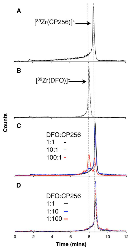
Figure 6: Reverse phase radiochromatogram of (A) [\text{}^{89}\text{Zr}(\text{CP256})]^+ (black) and (B) [\text{}^{89}\text{Zr}(\text{DFO})]^+ (dotted line); (C) A solution of [\text{}^{89}\text{Zr}(\text{CP256})]^+ incubated with \text{H}_3\text{DFO} ligand ( \text{H}_3\text{CP256}:\text{H}_3\text{DFO} = 1:1 , black line); ( \text{H}_3\text{CP256}:\text{H}_3\text{DFO} = 1:10 , blue line); ( \text{H}_3\text{CP256}:\text{H}_3\text{DFO} = 1:100 , red line); in all experiments, final [\text{H}_3\text{CP256}] = 500 \mu\text{M} . (D) A solution of [\text{}^{89}\text{Zr}(\text{DFO})]^+ incubated with \text{H}_3\text{CP256} ligand ( \text{H}_3\text{DFO}:\text{H}_3\text{CP256} = 1:1 , black line); ( \text{H}_3\text{DFO}:\text{H}_3\text{CP256} = 1:10 , blue line); ( \text{H}_3\text{DFO}:\text{H}_3\text{CP256} = 1:100 , red line); in all experiments, final [\text{H}_3\text{DFO}] = 500 \mu\text{M} .
