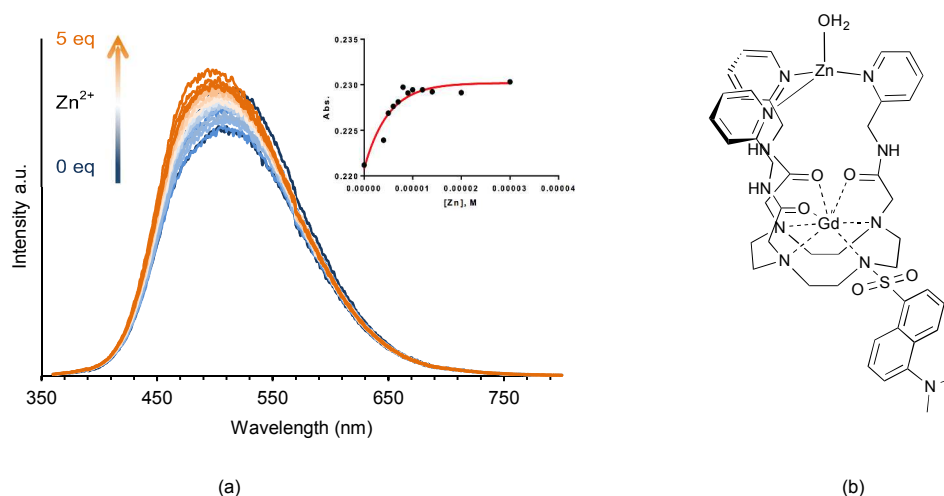
Figure 2: (a) Fluorescence spectrum of [\text{GdL}^1] (100 \mu\text{M} ) in MeOH in the presence of increasing concentrations (0 to 5 eq.) of \text{Zn}^{2+} ( \lambda_{\text{ex}} = 335 \text{ nm} ); (b) Proposed steric hindrance around the gadolinium centre induced by coordination of zinc to [\text{GdL}^1] .
