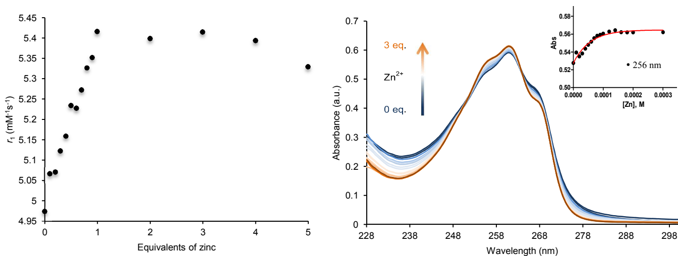
Figure 3: (Left) Water proton relaxivity of \text{GdL}^2 (pH 7.4, 5 mM) in the presence of increasing concentrations (0 to 5 eq.) of \text{Zn}^{2+} ; (right) UV/vis spectra of \text{GdL}^2 (100 \mu\text{M} ) in HEPES buffer (0.1 M; pH = 7.4) in the presence of increasing concentrations (0 to 3 eq.) of \text{Zn}^{2+} .
