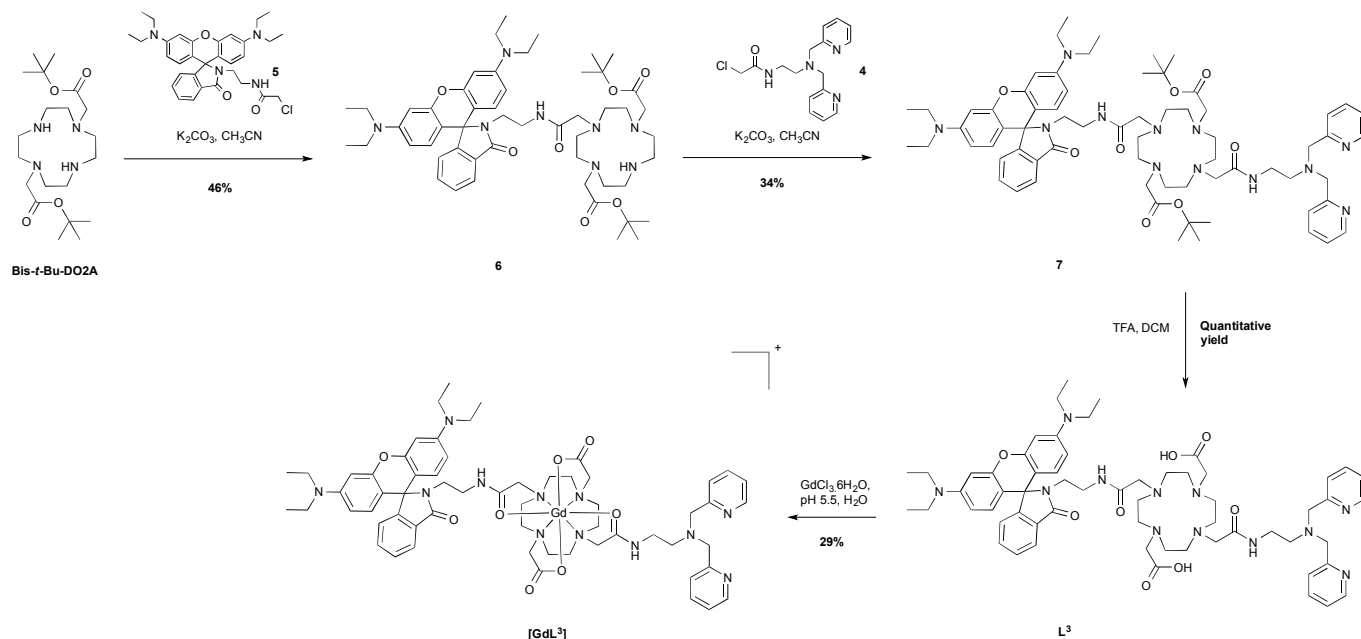
Scheme 3: Synthesis of the rhodamine-BPEN-DO2A conjugate [GdL 3 ] .
