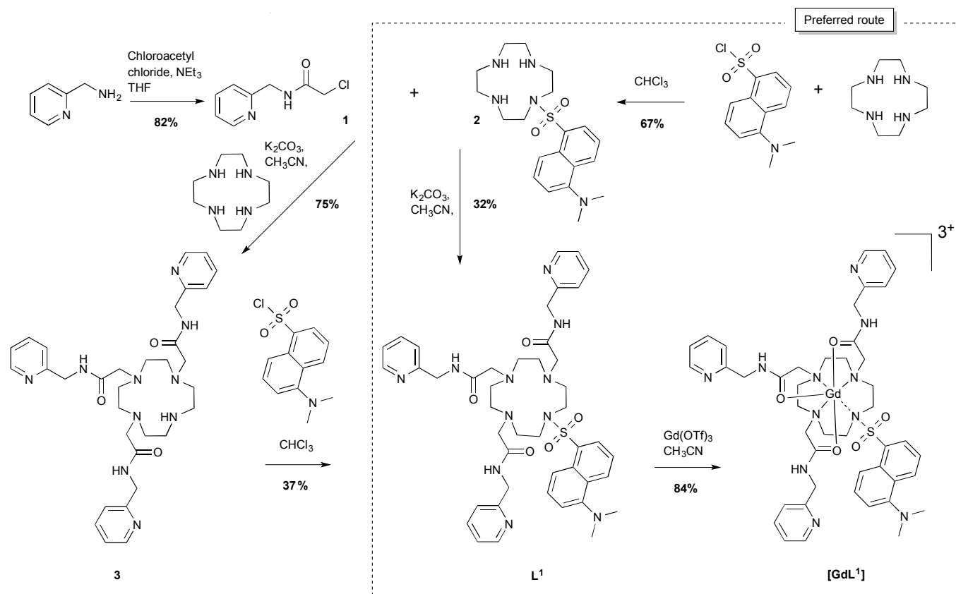
Scheme 1: Scheme of the synthesis of dansyl-DO3AMA complex [\text{GdL}^1] .
