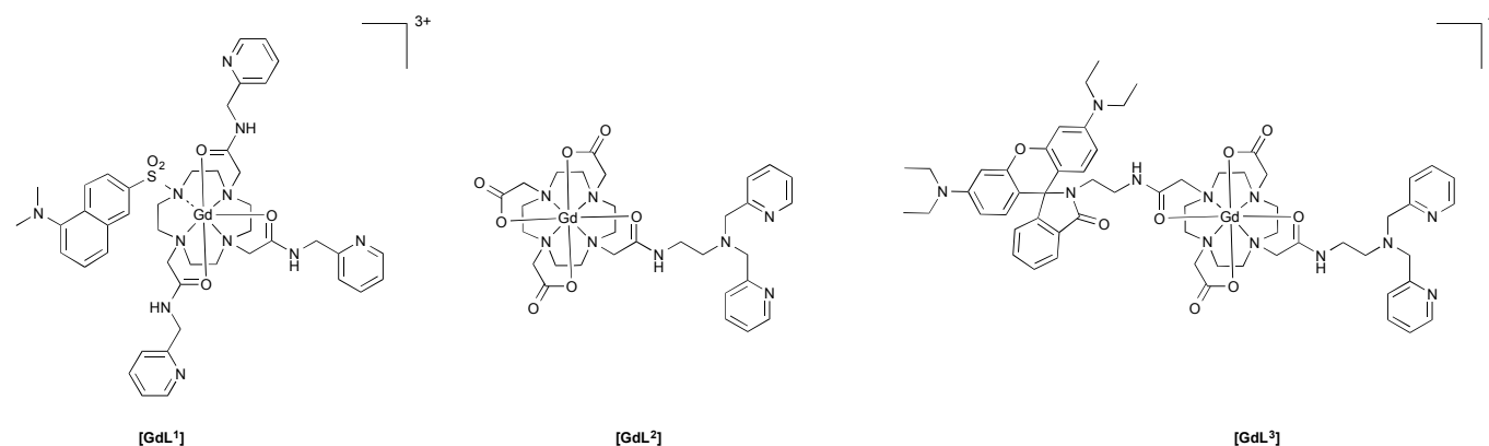
Figure 1: Structures of the [ GdL 1-3 ] complexes reported herein.
