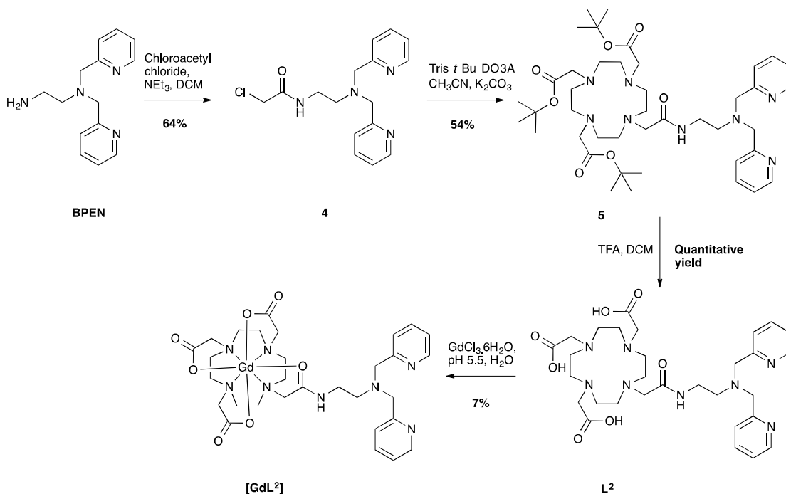
Scheme 2: Synthesis of BPEN-DO3A conjugate \text{GdL}^2 .
