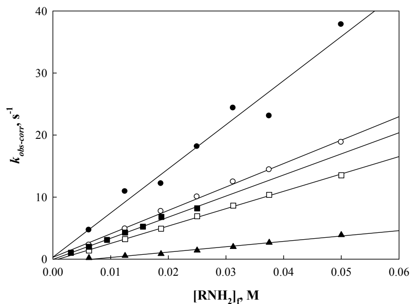
Figure 2. Plot of k_{obs-corr} vs. [RNH_2]_f for the reaction of 4W- t Bu in 50% MeCN-50% water with: (●) n -butylamine, pH = 10.4; (○) benzylamine, pH = 9.12; (■) methoxyethylamine, pH = 9.39; (□) furfurylamine, pH = 8.58; (▲) glycine ethyl ester, pH = 7.43, ionic strength = 0.1 M (KCl), 25 °C.
