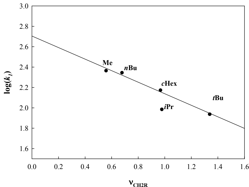
Figure 7. Plot of \log(k_1) vs. v_{CH_2R} for the reaction of 4W-R with glycine ethyl ester in 50 % MeCN – 50% water at 25 °C and ionic strength = 0.1 M (KCl).
