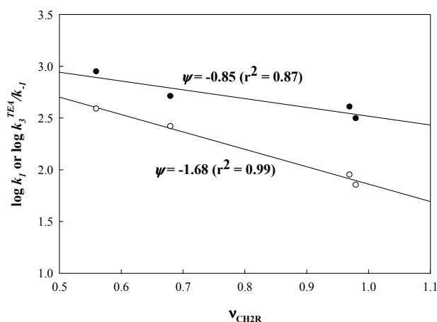
Figure 8. Plots of \log k_I (●) and \log k_3^{TEA}/k_{-1} (○) vs. \nu_{CH2R} for the reaction of 4W-R with morpholine in 50 % MeCN–50% at 25 °C and ionic strength = 0.1 M (KCl).
