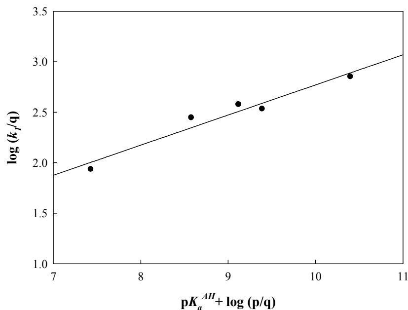
Figure 6. Brønsted plot for the reaction of 4W-tBu with primary amines in 50 % MeCN – 50% water at 25 °C, ionic strength = 0.1 M (KCl).
