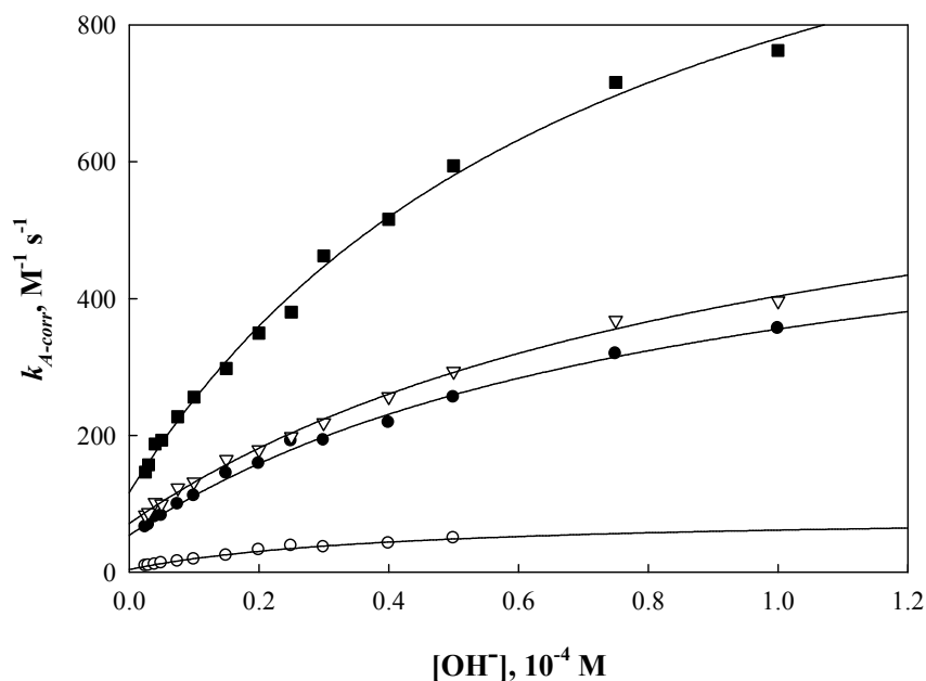
Figure 5. Plot of k_{A-corr} vs. [\text{OH}^-] for the reaction of morpholine with 4M-R in 50% MeCN-50% water; (■) 4W-nBu , (▽) 4W-cHex , (●) 4W-iPr and (○) 4Cr-cHex . Conditions: [\text{4M-R}]_0 = 1.0 \times 10^{-4} M, [\text{Morph}]_f = 0.01 or 0.02 M, [\text{TEA}]_f = 0.01 M, ionic strength = 0.1 M (KCl), 25 °C.
