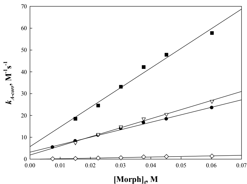
Figure 3. Plots of k_{A-corr} vs. [Morph]_f for the reaction of morpholine with (■) 4W- n Bu , (▽) 4W- c Hex , (●) 4W- i Pr and (◇) 4Cr- c Hex in 50% MeCN–50% water at pH = 8.88, ionic strength = 0.1 M (KCl), 25 °C.
