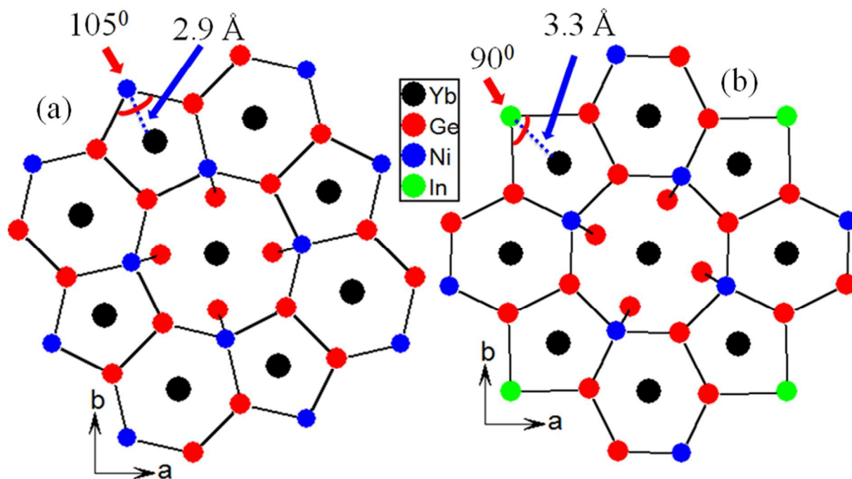
Figure 2. Crystal structure comparison of (a) \text{Yb}_5\text{Ni}_4\text{Ge}_{10} and (b) \text{Yb}_7\text{Ni}_4\text{InGe}_{12} is viewed in the ab -plane. Both structures consist of eight-membered ring with surrounding five and six membered rings.
