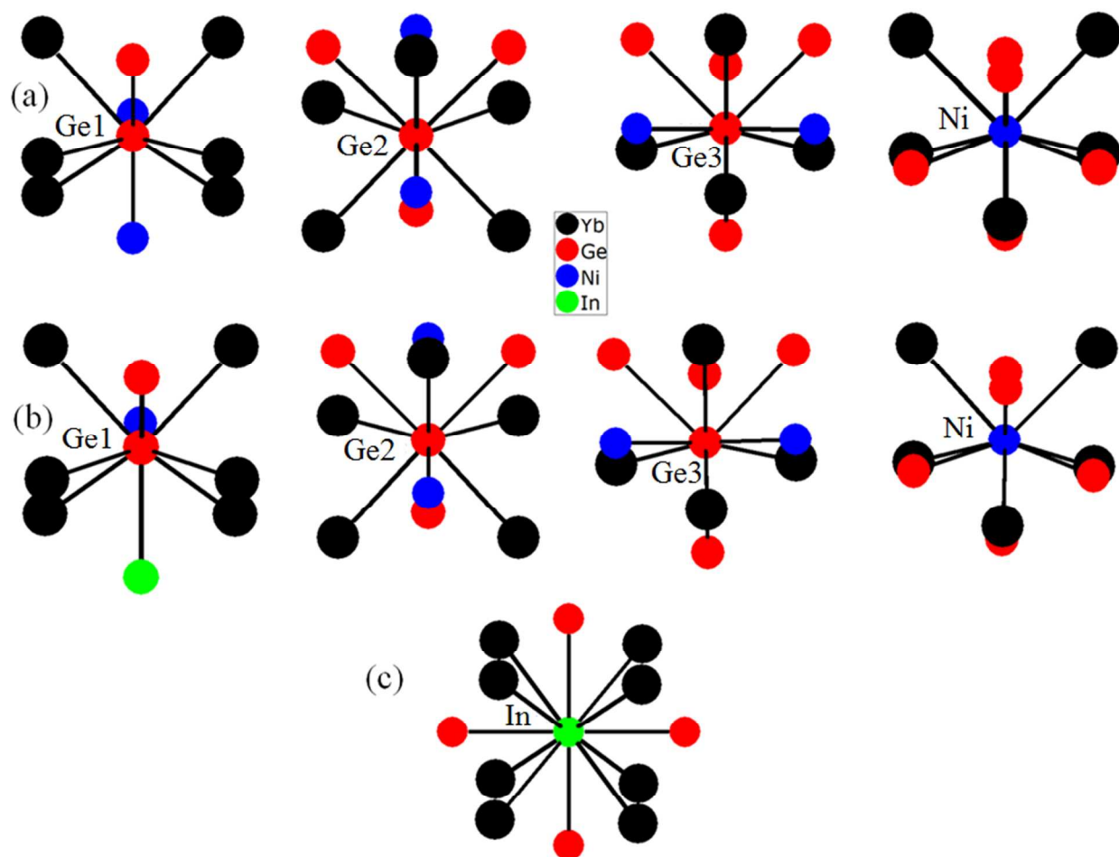
Figure 5. The coordination sphere of Ge and Ni and In atoms in (a) \text{Yb}_5\text{Ni}_4\text{Ge}_{10} and (b) \text{Yb}_7\text{Ni}_4\text{InGe}_{12} are presented. (c) the coordination environment of In atom in \text{Yb}_7\text{Ni}_4\text{InGe}_{12} .
