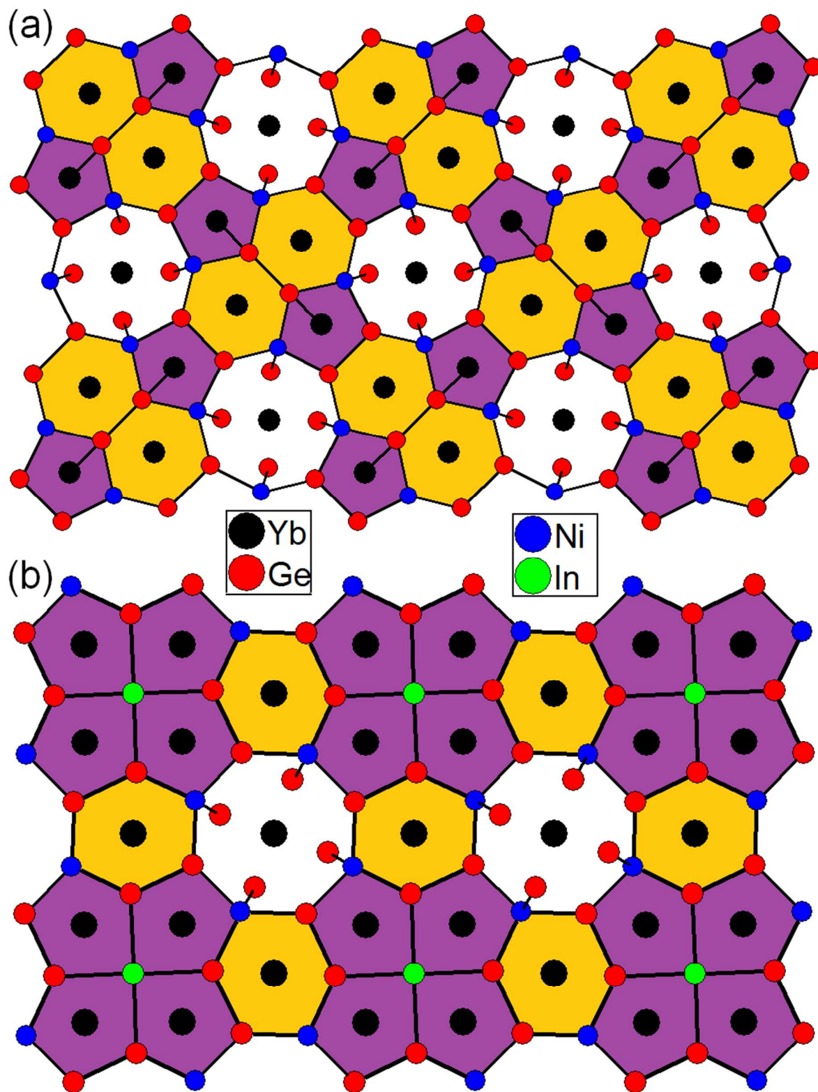
Figure 3. Comparison of the crystal structures of (a) Yb 5 Ni 4 Ge 10 and (b) Yb 7 Ni 4 InGe 12 viewed along the c -axis.
