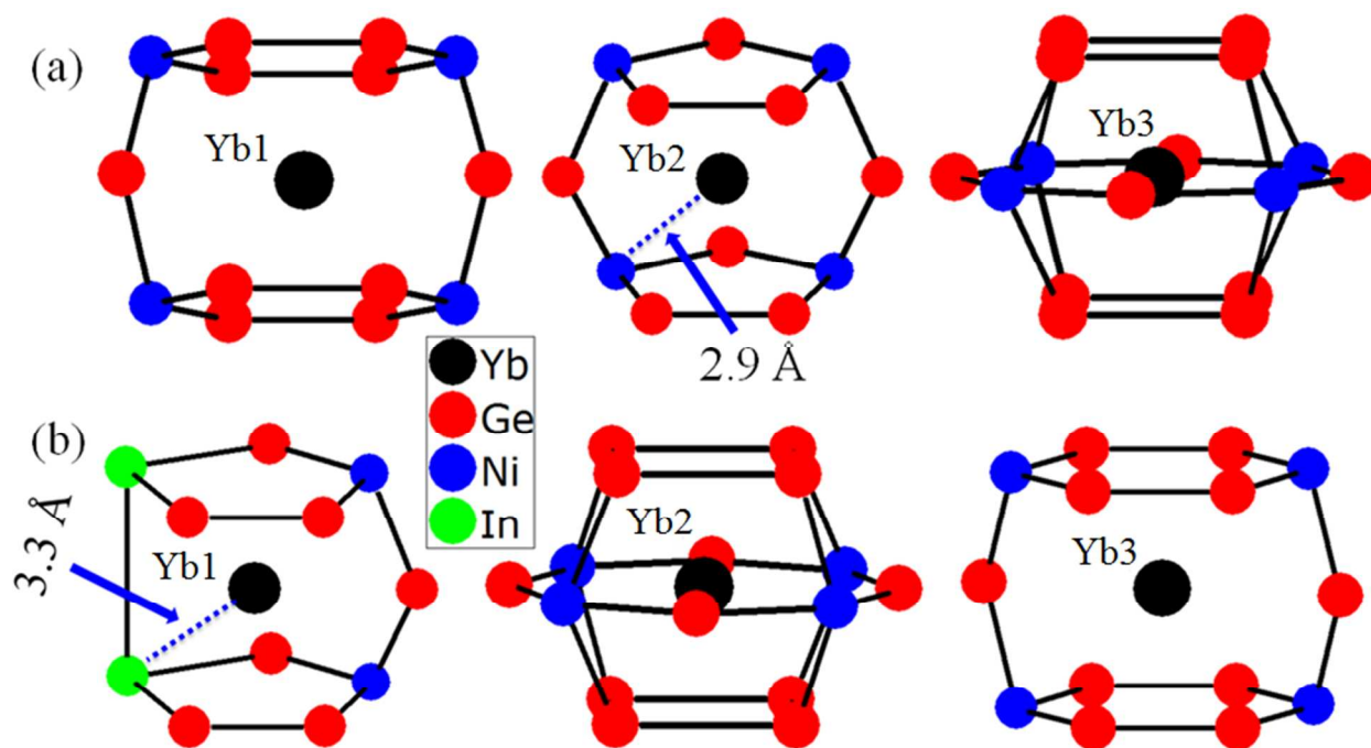
Figure 4. The coordination sphere of all Yb atoms in in (a) \text{Yb}_5\text{Ni}_4\text{Ge}_{10} and (b) \text{Yb}_7\text{Ni}_4\text{InGe}_{12} .
