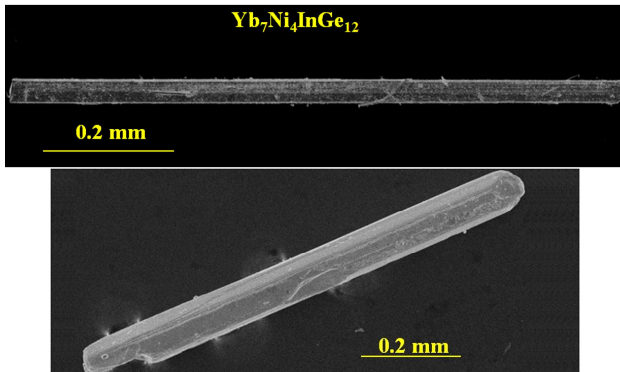
Figure 1. SEM images of the typical single crystals of \text{Yb}_7\text{Ni}_4\text{InGe}_{12} grown from indium flux.
