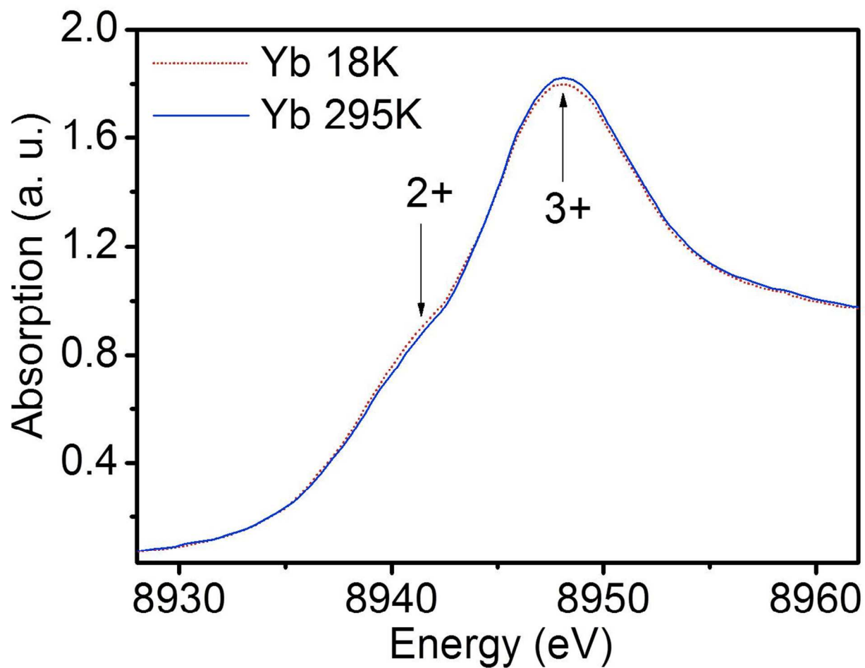
Figure 8. Yb L_{III} absorption edge spectra taken from a polycrystalline samples of \text{Yb}_7\text{Ni}_4\text{InGe}_{12} at 300 K and 18 K.
