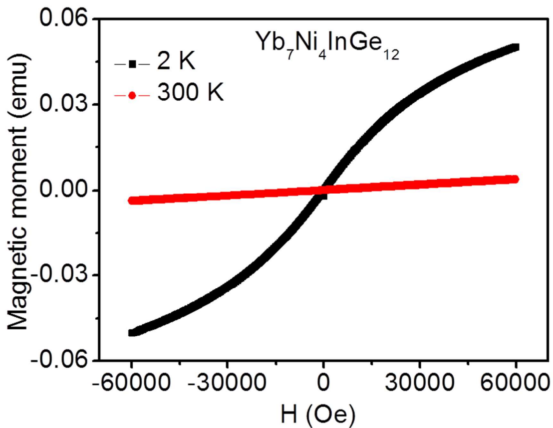
Figure 7. Magnetization as a function of applied magnetic field at 2 K and 300 K for \text{Yb}_7\text{Ni}_4\text{InGe}_{12} .
