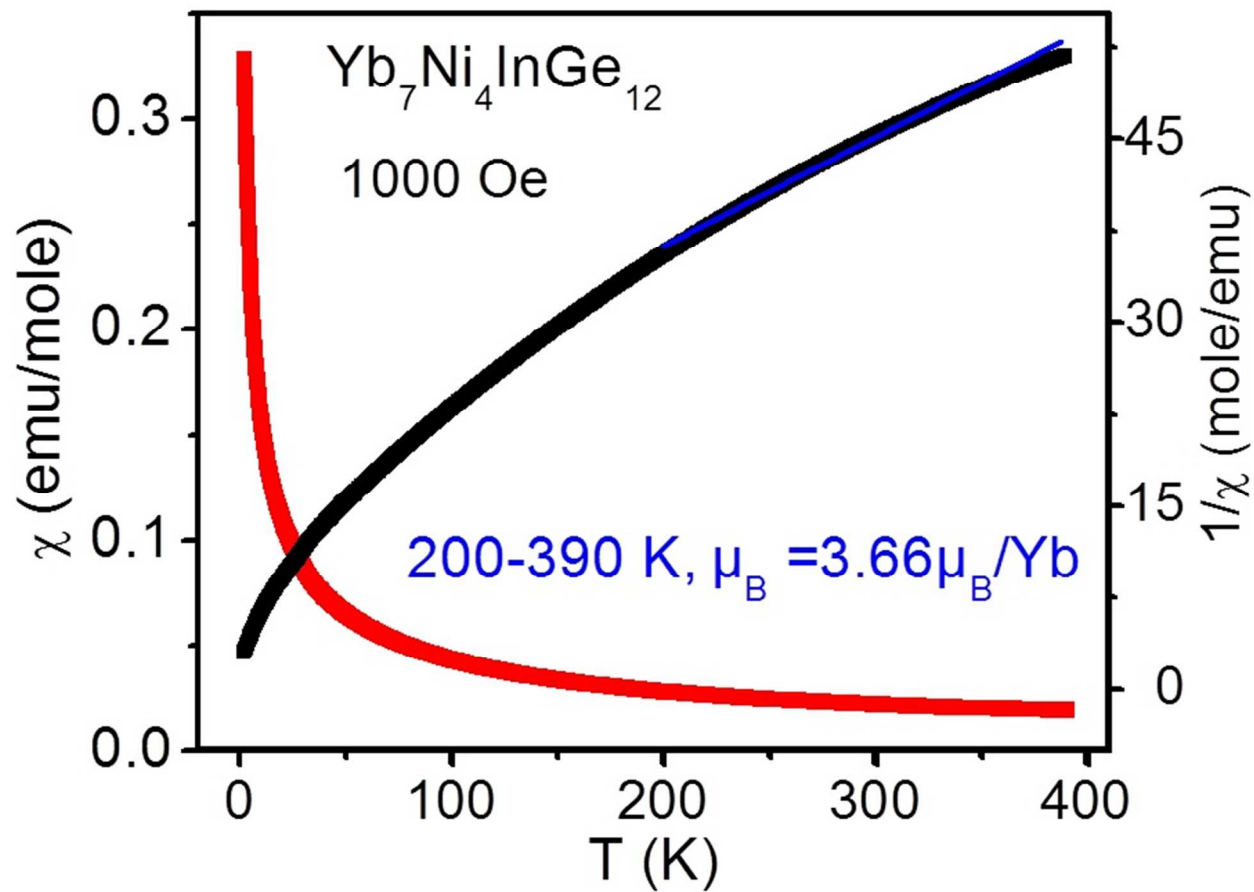
Figure 6. Temperature dependence of the magnetic susceptibility ( \chi_m ) and inverse susceptibility ( 1/\chi_m ) for a polycrystalline sample of \text{Yb}_7\text{Ni}_4\text{InGe}_{12} measured at 1000 Oe applied field.
