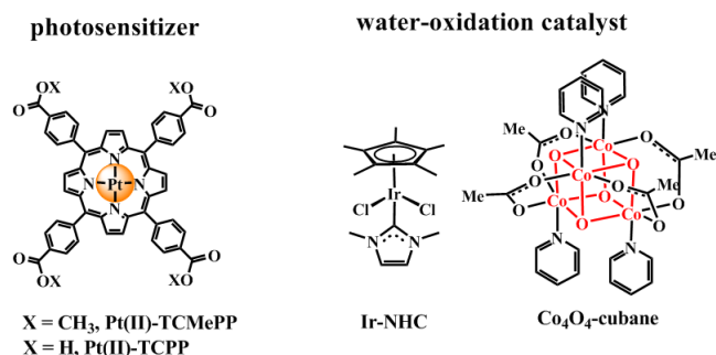
Figure 1. Chemical structures of the Pt(II)-porphyrin photosensitizers Pt(II)-TCMePP, Pt(II)-TCPP and two homogeneous water oxidation catalysts: Ir-NHC, Co 4 O 4 -cubane used in this study.
