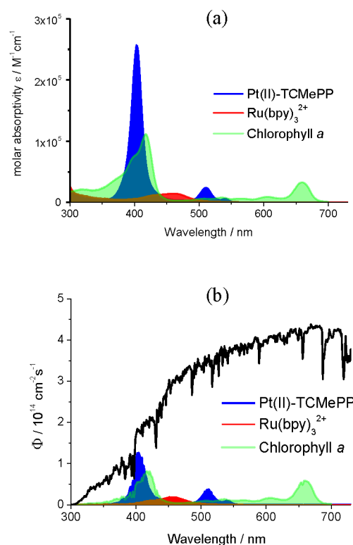
Figure 7. (a) UV-vis spectra and (b) solar irradiance photon flux AM1.5G (black) and photon absorption rate for 2 μM solution of Pt(II)-TCMePP (blue), Ru(bpy) 3 2+ (red), chlorophyll a (green) in a 1 cm path length cell.
