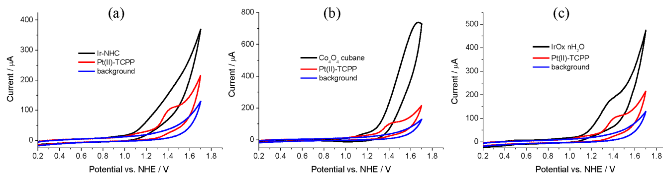
Figure 3. Cyclic voltammograms of (a) Ir-NHC (1 mM), (b) \text{Co}_4\text{O}_4 -cubane (1 mM), (c) \text{IrO}_x \cdot n\text{H}_2\text{O} nanoparticles (1.9 mM) compared with Pt(II)-TCPP (1 mM; red curves) and the \text{NaH}_2\text{PO}_4/\text{Na}_2\text{HPO}_4 (0.2 M, pH = 7.0) electrolyte background (blue curves).
