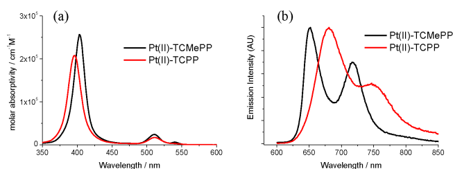
Figure 2. (a) Absorption spectra of Pt(II)-TCMePP (black) in dichloromethane and Pt(II)-TCPP (red) in phosphate buffer (0.1 M, pH = 7.0) solution. (b) Emission spectra upon 540 nm excitation at room temperature in the corresponding solvents.
