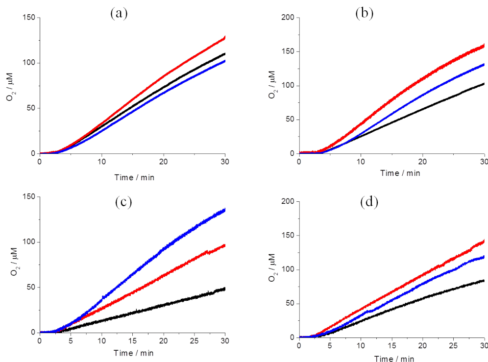
Figure 6. Photochemical water oxidation with different excitation powers (black = 5.2 mW, red = 21.2 mW, blue = 51.6 mW) of 532 nm green laser. Volume = 1.5 mL, pH 7.0, 0.1 M phosphate buffer, containing \text{Na}_2\text{S}_2\text{O}_8 ( 1.67 \times 10^{-2} M), Pt(II)-TCPP ( 2.23 \times 10^{-4} M) and catalysts: (a) Ir-NHC ( 1.67 \times 10^{-5} M), (b) \text{Co}_4\text{O}_4 cubane ( 1.67 \times 10^{-5} M), (c) \text{IrO}_x \cdot n\text{H}_2\text{O} nanoparticles ( 6.00 \times 10^{-5} M) and (d) \text{Co}_3\text{O}_4 nanoparticles ( 1.39 \times 10^{-5} g/mL).
