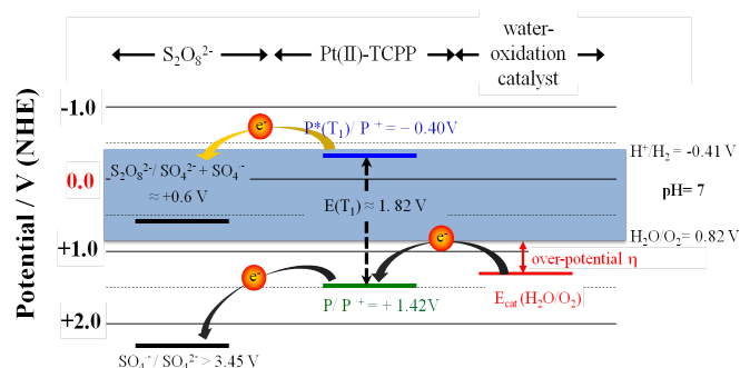
Figure 4. Energy scheme of Pt(II)-TCPP and water oxidation catalysts. Overpotential \eta : 380 mV for Ir-NHC, 500 mV for \text{Co}_4\text{O}_4 -cubane, 330 mV for \text{IrO}_x \cdot n\text{H}_2\text{O} nanoparticles and 350 mV for \text{Co}_3\text{O}_4 nanoparticles in phosphate buffer (0.2 M, pH = 7.0) solution..
