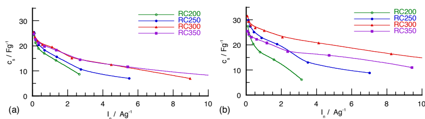
Fig. 7 Specific capacitance determined at different rates of constant current discharge between 0 and 3.0 V for cells using ammonium based ionic liquids and controlled porosity carbons. (a) [N 2224 ][Tf 2 N] and (b) [N 221(102) ][Tf 2 N]
