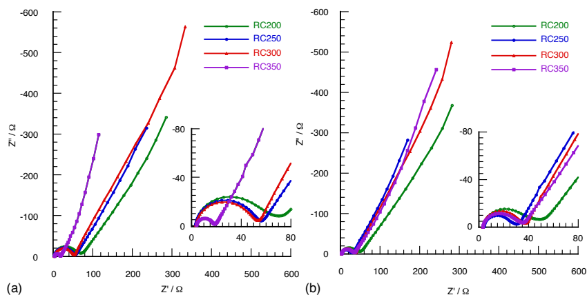
Fig.4 Nyquist plots obtained using electrochemical impedance spectroscopy for sulfonium based ionic liquids with controlled porosity carbons including magnified high-frequency regions (inset).
