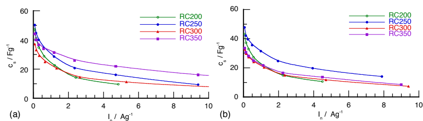
Fig. 5 Specific capacitance determined at different rates of constant current discharge between 0 and 2.5 V for cells using sulfonium based ILs. (a) [\text{S}_{221}][\text{Tf}_2\text{N}] and (b) [\text{S}_{222}][\text{Tf}_2\text{N}] .
