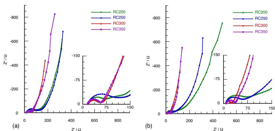
20 Fig. 6 Nyquist plots obtained using EIS for ammonium-based ILs with controlled porosity carbons including magnified high-frequency regions (inset). (a) [N_{2224}][Tf_2N] and (b) [N_{221(102)}][Tf_2N] .
