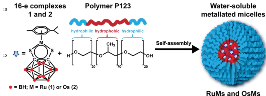
20 Figure 1. Self-assembly formation of RuMs and OsMs (the red dots in 1 and 2 are boron-hydrogen vertices).
