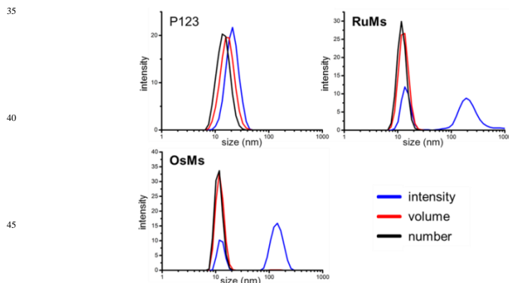
Figure 2. DLS spectra of P123Ms, RuMs , and OsMs (1 mg/mL, H 2 O).
