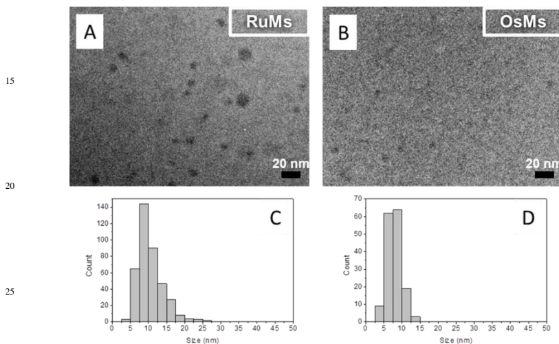
Figure 3. Cryo-TEM of the self-assembled block copolymer micelles containing encapsulated ruthenium and osmium carborane complexes. (A) and (B) images, and (C) and (D) particle counting/histogram analysis for RuMs and OsMs , respectively.
