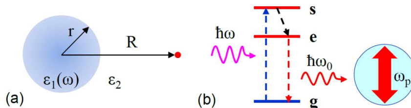
Fig. 1 Schematic of a system with a QDE placed near an MNP, indicating (a) system parameters and (b) QDE energetic levels along with an oscillating current associated with the LSP excitation.
