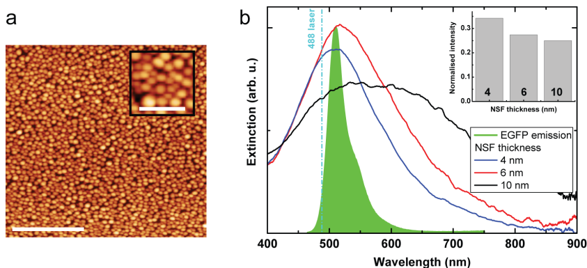
Figure 1. (a) AFM image of a silver film with a 6 nm nominal Ag thickness; scale bar is 2 \mu\text{m} . Inset: enlarged region; scale bar is 500 nm. (b) Extinction spectra for large area nanostructured silver films (NSF) of nominal thicknesses 4 nm (blue line), 6 nm (red) and 10 nm (black). Also shown is the emission spectrum of eGFP (filled green), and the 488 nm excitation laser. Inset: fluorescence intensity from cells on an NSF normalised to those on a nearby area of glass (a scratch in the silver film), for NSFs of different nominal thickness.
