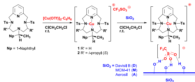
Scheme 1 General synthesis of the supported catalyst 1/D-M and 2/D
