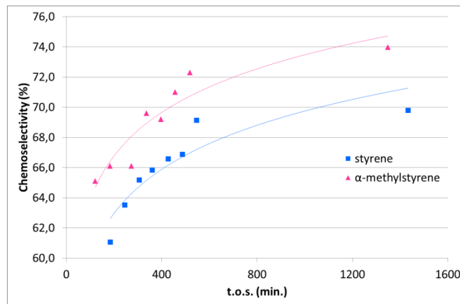
Figure 1. Chemoselectivity (%) vs t.o.s. (minutes) of styrene and \alpha -methylstyrene catalysed by 2/D .
