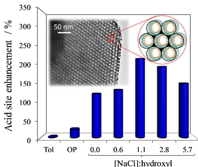
Figure 1. a) Effect of [\text{NaCl}]:\text{hydroxyl} ratio during \text{-PrSO}_3\text{H} grafting in \text{H}_2\text{O}/\text{NaCl} on resulting acid site loading, as compared to conventional toluene grafted and one-pot co-condensed materials. Inset shows HRTEM for [\text{NaCl}]:\text{hydroxyl} = 1.1 , confirming ordered mesoporosity is retained. (Hydroxyl density for parent SBA-15 calculated to be 3 \text{ mmol}\cdot\text{g}^{-1} from TGA over the range 200\text{-}1000 °C).
