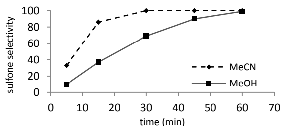
Figure 1 Influence of reaction conditions on the selectivity for methyl phenyl sulfone for the oxidation of thioanisole with \text{H}_2\text{O}_2 using 0.5 mol%
