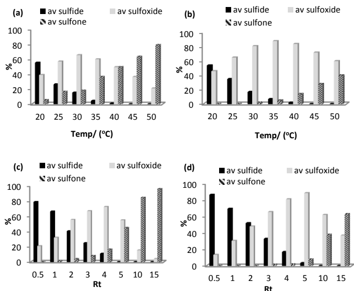
Figure 4 Conversion-selectivity profile as a function of temperature for the continuous flow [\text{PO}_4\{\text{WO}(\text{O}_2)_2\}_4]@ PIILP-catalysed sulfoxidation of thioanisole in (a) acetonitrile (b) methanol for a residence time of 4 min. Conversion-selectivity profile as a function of residence time (Rt) for the [\text{PO}_4\{\text{WO}(\text{O}_2)_2\}_4]@ PIILP-catalysed sulfoxidation of thioanisole in (c) acetonitrile (d) methanol at 30 °C. Reaction conditions: 0.1 g catalyst/2.0 g silica, 3 equiv. 35% \text{H}_2\text{O}_2 , solvent, residence time 0.5-15 min or temperature 20-50 °C.
