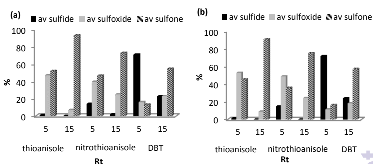
Figure 6 (a) Conversion-selectivity profile at residence times of 5 and 15 min for the continuous flow [\text{PO}_4\{\text{WO}(\text{O}_2)_2\}_4]\text{@PIILP} -catalysed consecutive sulfoxidation of three different substrates (i) thioanisole, (ii) 4-nitrothioanisole and (iii) dibenzothiophene with the same catalyst cartridge. (b) Conversion-selectivity profile at residence times of 5 and 15 min for the continuous flow [\text{PO}_4\{\text{WO}(\text{O}_2)_2\}_4]\text{@PIILP} -catalysed sulfoxidation using a fresh catalyst cartridge for each substrate. Reaction conditions: 0.1 g catalyst/2.0 g silica, 3 equiv. 35% \text{H}_2\text{O}_2 , MeCN, 30 °C, residence times 5 and 15 min.
