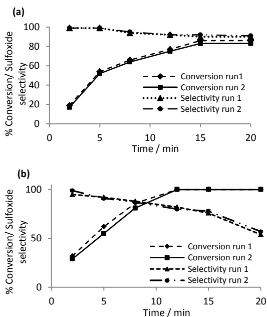
Figure 2 (a) Conversion and sulfoxide selectivity profiles as a function of time for a recycle [\text{PO}_4\{\text{WO}(\text{O}_2)_2\}_4]@\text{PIILP} -catalysed sulfoxidation of thioanisole in (a) methanol at room temperature (b) acetonitrile at room temperature, using 0.5 mol% 2 and a substrate: \text{H}_2\text{O}_2 ratio 1:2.5.
