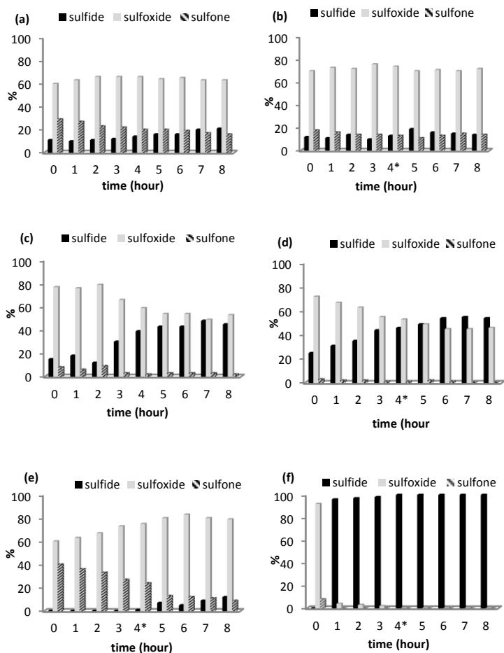
Figure 5 Conversion-selectivity profile as a function of time for an 8 h continuous flow [\text{PO}_4\{\text{WO}(\text{O}_2)_2\}_4]\text{@PIILP} -catalysed sulfoxidation of thioanisole at 30 °C with a residence time of 4 min in (a) acetonitrile, (b) acetonitrile with the \text{H}_2\text{O}_2 reservoir replenished after 4 h (*), (c) methanol, (d) methanol with the \text{H}_2\text{O}_2 reservoir replenished after 4 h (*). Conversion-selectivity profile as a function of time for an 8 h continuous flow sulfoxidation of thioanisole using [\text{nBu}_4\text{N}]\text{[PO}_4\{\text{WO}(\text{O}_2)_2\}_4] as catalyst at 30 °C with a residence time of 4 min in (e) acetonitrile and (f) methanol.
