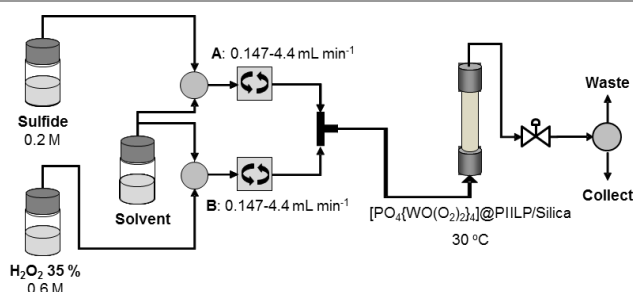
Figure 3 Schematic representation of the set-up for segmented and continuous flow sulfoxidations catalysed by [\text{PO}_4\{\text{WO}(\text{O}_2)_2\}_4]@\text{PIILP} (2).
