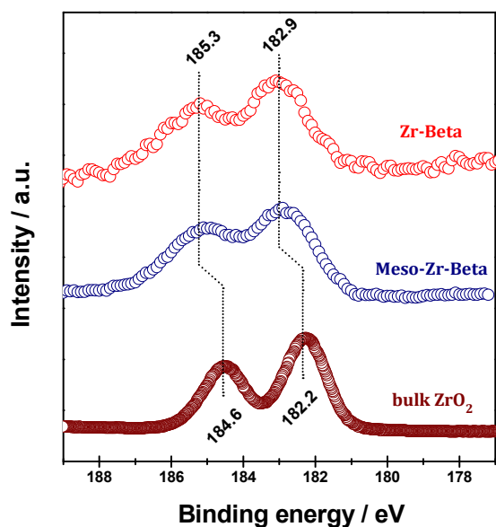
Figure 6 Zr 3d XPS of Zr-Beta, Meso-Zr-Beta, and ZrO_2 samples.
