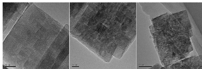
Figure 3 TEM micrograph images of parent H-Beta (left), Zr-Beta (middle), and Meso-Zr-Beta (right).
