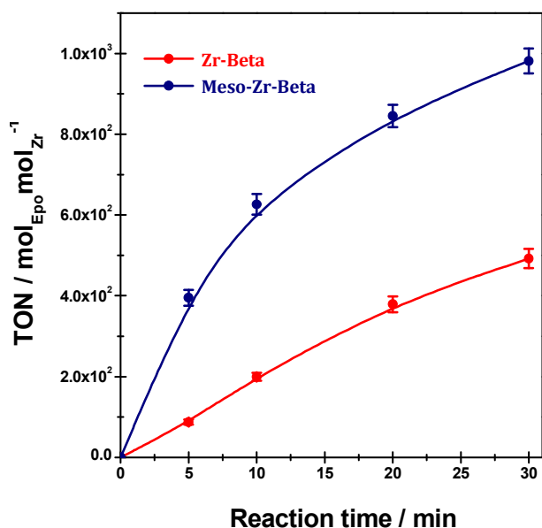
Figure 8 Time-dependent ring-opening aminolysis activity of Zr-Beta and Meso-Zr-Beta samples. Reaction conditions: 5 mmol epoxide, 5 mmol amine, 25 mg catalyst, temperature = 308 K.
