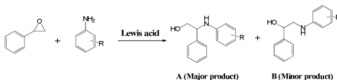
Scheme 2 Ring-opening of epoxide with amines over a solid Lewis acid catalyst.
