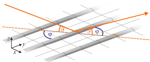
Fig. 2 Principle layout of the sample. The Cr stripes are parallel to the y -axis and lie in the x - y -plane. The angle between the incident radiation and the x - y -plane is represented by \vartheta ; the tilt angle between the y -axis and the projection of the incident beam on the x - y -plane is denoted by \varphi .
