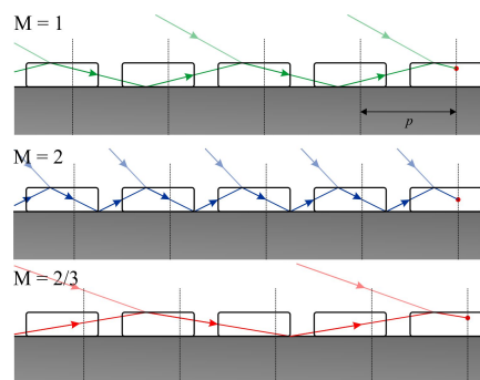
Fig. 6 Sketch showing possible ray paths for multiple reflections. M stands for the number of reflections which take place within one period of the structure (see Eq. 1).
