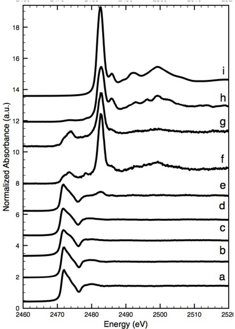
Sulfur K-edge XANES: para-realgar (a), realgar (b), orpiment (c), intact (para)realgar particle in the lower part of the paint layer in Coorte sample, see point 1 in Fig. 5B (d), (para)realgar particle in the upper part of the paint layer in Coorte sample, see point 2 in Fig. 5B (e), at the interface between the ground and the paint layer in Coorte sample, see point 3 in Fig. 5B (f), arsenic rich area in the paint layer of Saybrook X4, see point 4 in Fig. 8B (g), next to the arsenic rich area in the paint layer of Saybrook X4, see point 5 in Fig. 8B (h) and reference of gypsum (i). 190x265mm (72 x 72 DPI)
