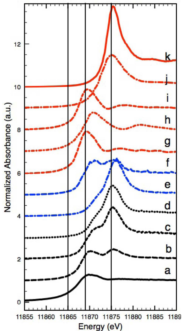
Arsenic \rightarrow K-edge XANES: intact arsenic sulfide particle in Coorte sample, see point 1 in Fig. 2I (a), at the interface between the ground and the paint layer in Coorte sample, see point 2 in Fig. 2I (b), in the photo-degraded upper part of the paint in Coorte sample, see point 3 in Fig. 2I (c), in the ground layer of Coorte sample, see point 4 in Fig. 2I (d), in the ground layer of Saybrook sample X8 (e), in the paint layer of Saybrook sample X8 (f) and references: Realgar (g), As 2 O 3 (h), Orpiment (i), As 2 O 5 (j) and Ca 3 (AsO 4 ) 2 (k). The vertical lines indicate the energies selected for multiple energy XRF mapping (Fig. 5), because they show the largest differences in XRF intensities with respect to the different As oxidation states.
