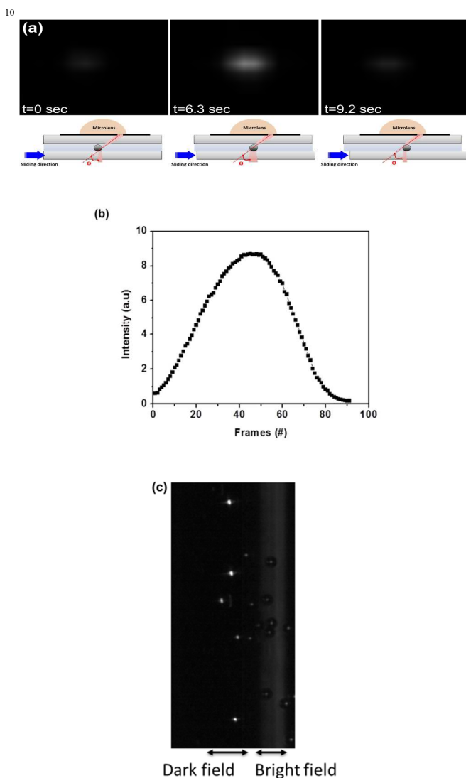
Figure 2 (a) Snapshots of a 15\mu\text{m} bead traveling the sensing area at different times. \Theta , shown in the schematics, is the scattering angle between the optics axis and the transmitted light sheet beam. (b) The intensity plot of the large angle scattering by a 15\mu\text{m} bead (each frame represents a physical distance of 0.416\mu\text{m} in this case). (c) A snapshot of 15\mu\text{m} polystyrene beads interrogated with the scattering-imaging-based cytometer platform, showing the dark-field scattering images and the bright-field image right next.
