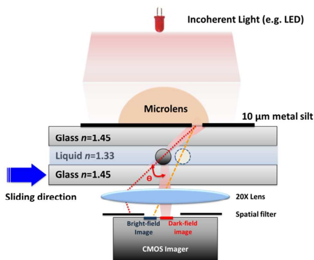
Figure 1 Design of the scattering-imaging-based cytometer. Incoherent light is used to form a light sheet beam by the microlens and the slit to scan through the cells. The autofluorescence of the lens material is used to form a transmitted bright-field image and the light sheet beam is used to form the dark-field scattering image. The two images occur at different locations of the CMOS imager and can be overlaid to produce the complete cell image. Autofluorescent light by the lens material is used as
