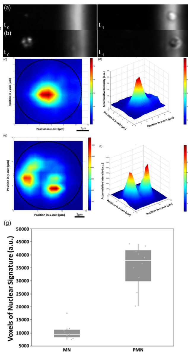
Figure 4 (a) Snapshots of mononuclear cells, e.g. lymphocytes, and (b) Snapshots of polymorphonuclear cells, e.g. neutrophils. All cells travelled through the dark-field imaging area first and then the bright-field imaging area. (c) and (d) are 2-dimensional and 3-dimensional contour plots of a mononuclear cell, respectively. (e) and (f) are 2-dimensional and 3-dimensional contour plots of a polymorphonuclear cell, respectively. (g) Box chart of voxels under 3-dimensional contour plot for mononuclear and polymorphonuclear cells, indicating the accumulative voxels, being proportional to the total volume of the nucleus, have a relatively tight distribution for each cell type.
