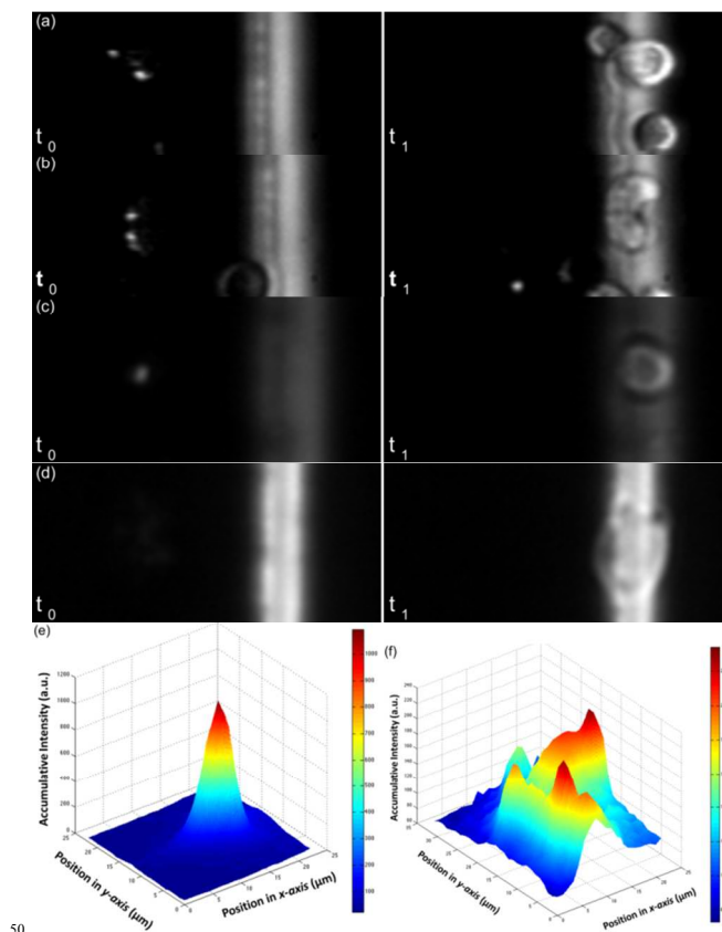
Figure 3 (a) and (b) Snapshots of uncontrolled HEK293 cells taken by a CMOS imager, where HEK293 cells were first imaged for the scattering patterns in the dark field, and then imaged in the bright field to delineate the cell boundaries. (c) and (d) Snapshots of HEK293 cells arrested at the G1/S phase and the prometaphase stage, respectively. The time lapse between t_0 and t_1 is 9.8 \pm 0.2 sec for (a) to (d). The exposure time in (d) is 3 times as long as (c) to underline the large difference in nucleus scattering intensity for cells in two different phases. (e) and (f) 3-dimensional contour plots of nucleus for HEK293 cells arrested at G1/S stage and at prometaphase stage.
