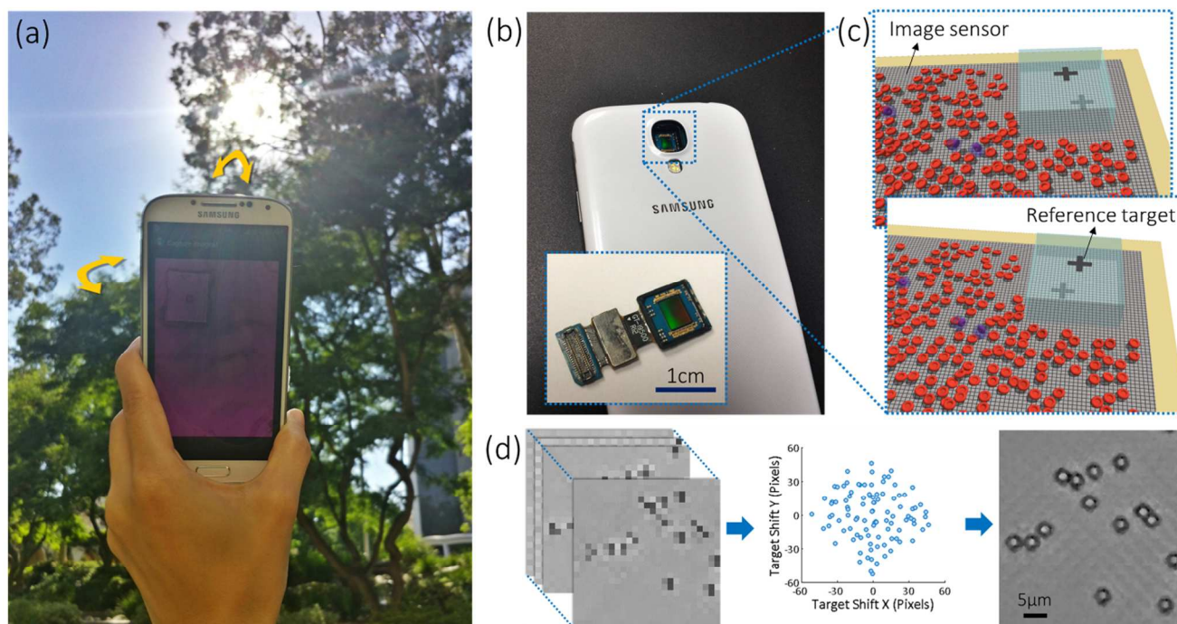
Figure 1. (a) Working principle of the smartphone-based chip-scale microscope using sunlight as the light source for imaging. For image capturing, the user holds the smartphone with the back camera module facing the sun and slowly moves the device to capture multiple images with varying angle of illumination. (b) The prototype device uses the back camera module of an android phone. We remove the lens module of the camera and place the sample directly on the surface of the image sensor. The inset shows the image sensor module with the lens removed. (c) As the user tilts the device around, we trace the shadow of a reference target placed on a corner of the image sensor to calculate sub-pixel shifts of the sample shadows. The reference target also allows us to check the quality of illumination, such that it creates a single, sharp shadow. (d) Raw (Left) and reconstructed (Right) images of 2.5\mu\text{m} microspheres. 100 images were taken while we manually tilt the device and the tilt angle for each image is shown in the plot (centre).
