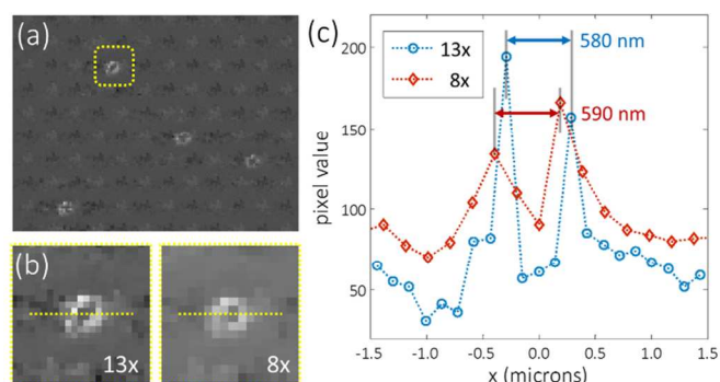
Figure 4. (a) Images captured with 500-nm polystyrene microspheres on the image sensor. We used 1.12- \mu\text{m} pixel sensors (effective low-resolution pixel size of 1.58 \mu\text{m} ) (b) Magnified images of the microsphere marked in (a). We used 13 \times and 8 \times enhancement for high resolution reconstruction. One pixel in each image measures 120 and 200nm, respectively. (c) Line trace of a microsphere images with 13 \times and 8 \times enhancement. In both cases, the centre of the microsphere is resolved.
