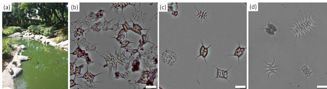
Figure 5. Portable microscopy of fresh-water microorganisms for water quality monitoring. (a) We took the fresh-water sample directly from a koi pond. 20- \mu\text{L} of sample was dispensed on the image sensor and the particles were let settle down for few minutes before image acquisition. (b-c) Reconstructed images of green algae found in the pond. (d) Conventional microscope images of same sample taken with 20 \times (0.4 Numerical Aperture) objective lens. The green algae found in the sample are different species of Scenedesmus , a genus of Chlorophyceae . All scale bars indicate 20 \mu\text{m}
