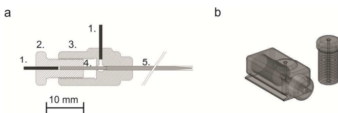
Fig. 2 Schematic of the microcapillary connector. (a) Assembly of a 2-piece connector made of: two steel pins (1), a screw (2) and a nut (3) that holds the inner and outer capillaries (4 and 5), respectively. Both pieces provide access to fluid inlets by steel pins that are connected with tubing. (b) 3D view of the screw and nut components.
