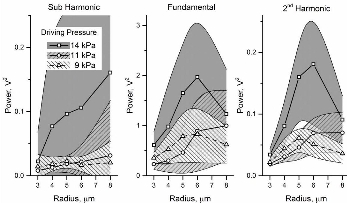
Figure 9: SonoVue ® mean subharmonic, fundamental and 2 nd harmonic light scattered power vs radius. Over 12,000 individual SonoVue ® microbubbles were analysed. Ultrasound parameters: 10 cycles of 3.5 MHz at varying driving pressures. Samples are divided into radius bins such that there are no less than 100 samples in each bin. Shaded areas represent \pm 0.5 standard deviation, demonstrating a large variability in acoustic response.
