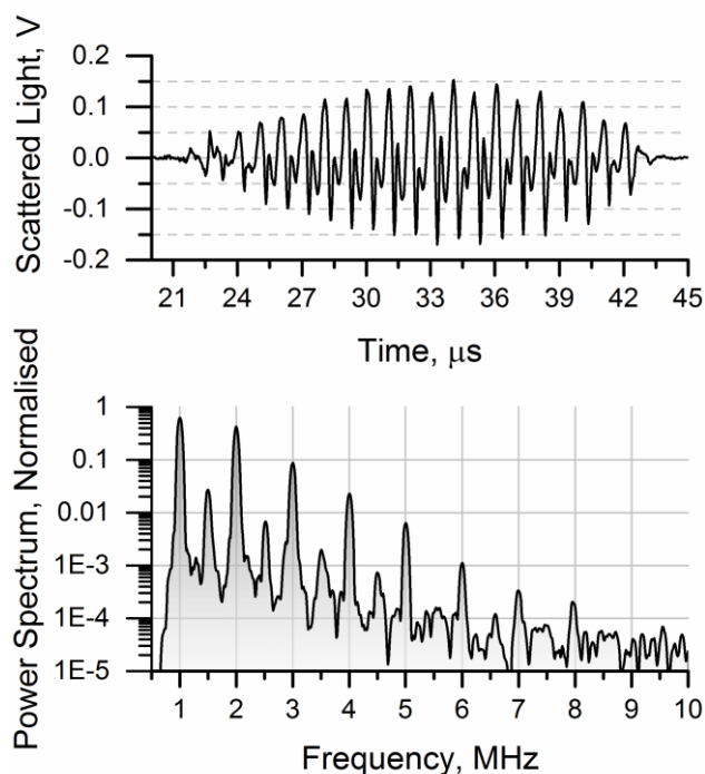
Figure 10: Example of light scattering due to the vaporisation of a liquid PFP droplet. Power spectrum demonstrates high bandwidth of light scattering method. Ultrasound parameters: 25 cycle of 1 MHz at 1 MPa peak negative pressure.
