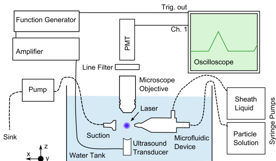
Figure 3: Schematic diagram (not in scale) for the characterisation of single echogenic particles using light scattering. The coaxial device and suction element are shown in greater detail in figure 2. Dotted lines indicate fluid flows.
