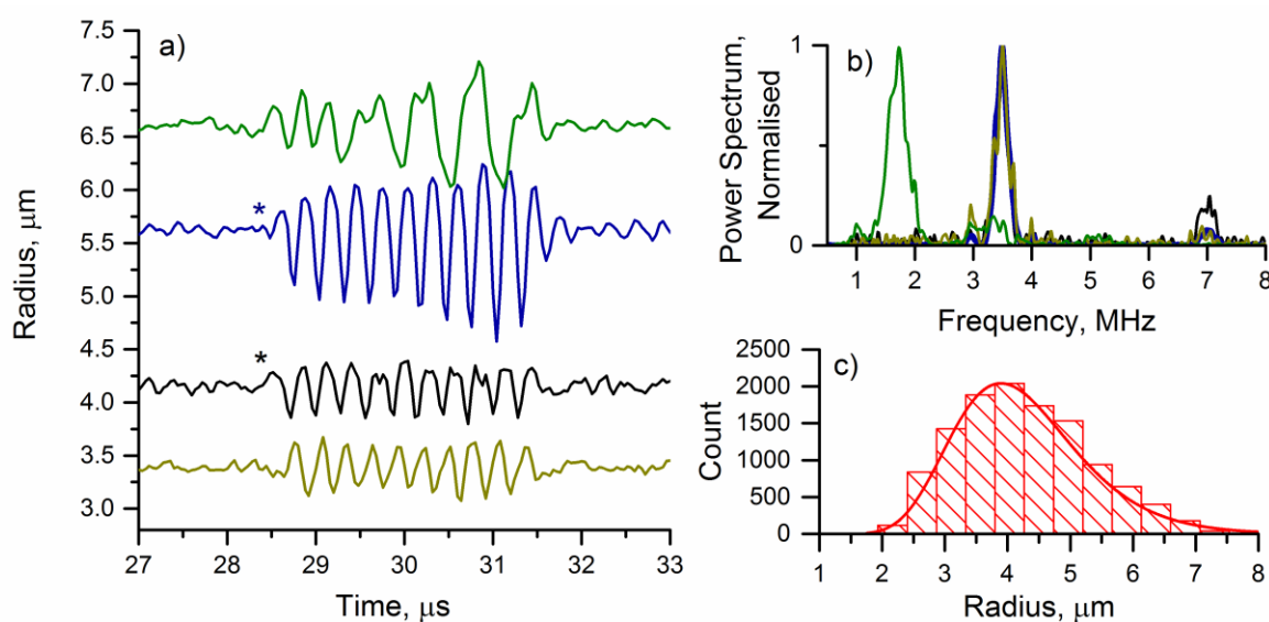
Figure 8: Examples of a) radius – time curves from SonoVue® microbubbles of different radii, the corresponding b) power spectra and c) the measured size distribution estimated from the light scattering data and Mie theory. Ultrasound parameters: 10 cycles of 3.5 MHz at peak negative pressure of 14 kPa. * indicates compression-only behaviour.
