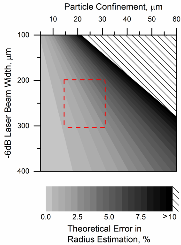
Figure 11: Theoretical error in particle radius estimation due to the variation in a particle's confinement while travelling through a Gaussian laser beam. Conditions are shown for varying laser beam width and particle confinement; the red dashed box indicates approximate operating area for the conditions described in this study.
