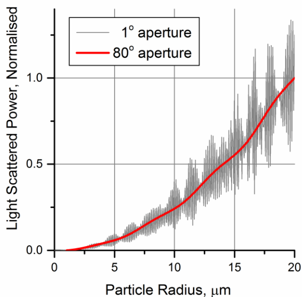
Figure 1: Mie scattering simulations of the scattered light power (normalised to the scatter from a 20 \mu\text{m} sphere) vs microcavity radius (in \mu\text{m} ) and light collection aperture. Increasing the aperture provides a monotonic relationship suitable for experimentally estimating a micro-cavity's radius.
