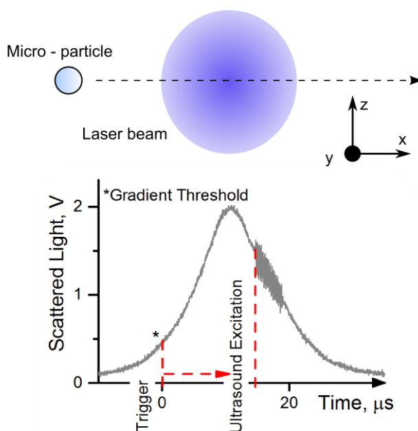
Figure 4: Demonstration of particle detection and ultrasound excitation. Ultrasound excitation is triggered from a gradient threshold (in the scattered light signal) as the particle enters the laser beam. After a short delay the ultrasound wave reaches the particle while it is still traversing the laser beam and the resulting volume oscillation is recorded. Data shown is of a SonoVue ® microbubble.
