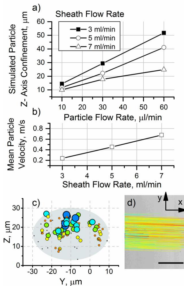
Figure 6: Simulations from particle tracking (density 1.331 \text{ kg}/\text{m}^3 , radii between 1 to 15 \mu\text{m} with a mean radius of 3.5 \mu\text{m} ). a) Confinement of particles in z axis, where confinement is the largest distance between two particles b) Particle velocities as a function of outer flow rate. c) Example of particle spatial spread ( n = 93 ) downstream, 6 mm away from the nozzle exit, particle radius is represented by the marker size, larger microbubbles tend towards the top of the distribution due to the likely combined effect of buoyancy and lift forces. Outer flow rate = 3 ml/min, inner flow rate = 20 \mu\text{l}/\text{min} . d) Experimental data of SonoVue® microbubbles at same flow conditions at c, recorded using a high speed camera at 50 kfps, each line represents the path of a single bubble which could be compared with the simulated trajectories. Scale bar = 20 \mu\text{m} .
