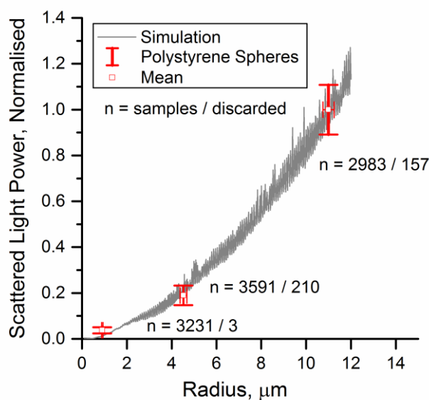
Figure 7: Sizing and sensitivity calibration using size standard polystyrene microparticles. Light scattering results (vertical red bars represent \pm standard deviation in light scattering intensity, horizontal red bars represent standard deviation in microparticles size from manufacturer's specification) are compared to Mie Scattering simulations of the polystyrene microparticles (refractive indices of water = 1 and microparticles = 1.6, unpolarised light at 405 nm, 80° aperture). Discarded samples refer to particles outside of the normal transit time through the laser beam. The scattered light intensity is normalised with respect to the Mie scattering estimation for a 11 \mu\text{m} microsphere.
