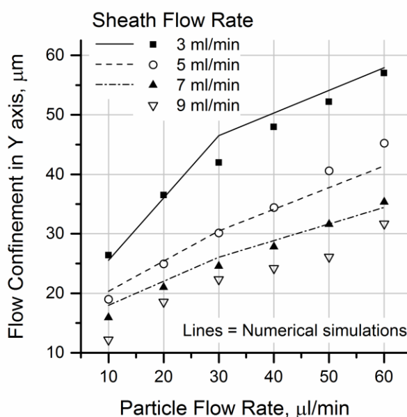
Figure 5: Effect of sheath and particle flow rates on the hydrodynamic flow confinement 6 mm downstream from the exit of the microfluidic device. Numerical simulations (lines) are shown together with the experimental points (symbols). Please see also figure S3.
