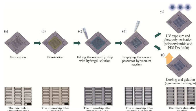
Figure 2. Fabrication process flow for custom hydrogel patterning in a closed microfluidic chip. Scale bars indicate 15 \mu\text{m} for all images.
