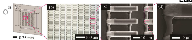
Figure 1. (a) 2D sketch of the microchip with sample inlets (*), microfluidic inlets and outlets, glass pillars and capillary barriers. (b) Optical microscopy image of glass pillar (rectangle) array, capillary barriers (structures between glass pillars) and air filled channels (light colored areas). (c) Tilted top view image of the glass capillary barriers between glass pillars under SEM; (d) a closer tilted top view of capillary barriers under SEM. The depth, width, and length of pillars and capillary barriers are 20 \times 4 \times 5 \mu\text{m} and 4 \times 1 \times 3 \mu\text{m} , respectively.
