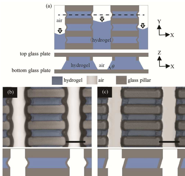
Figure 3. (a) Top and cross sectional schematic views of meniscus pinning at capillary barriers. Direction of hydrogel flow in channels during vacuum suction is indicated by arrows and cross sectional planes are shown by dashed lines. Phase contrast microscopy image of custom patterned polyacrylamide trapped in between glass pillars after photopolymerization using (b) parenthesis-shaped capillary barriers and (c) slash-shaped capillary barriers (the images are artificially colored on the basis of gray-scale differences). Scale bars indicate 10 μm for all images.
