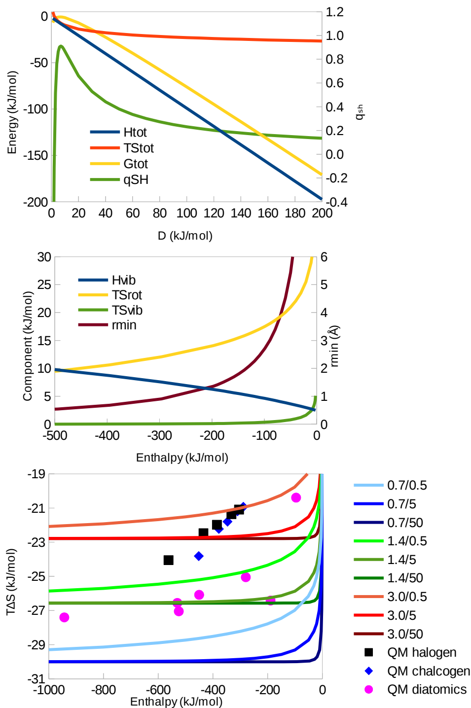
Figure 3. (a) Enthalpy, entropy, free energy, and q_{SH} as a function of D for the formation of a covalent bond with m_1 = m_2 = 19 Da (F), C = 8.87 \text{ \AA}^{-1} , and r_0 = 1.42 \text{ \AA} \times 181.6 \text{ kJ/mol} / D (which reproduces the QM results for F_2 , D = 181.6 \text{ kJ/mol} , r = 1.42 \text{ \AA} , and \nu = 1004 \text{ cm}^{-1} ). (b) The enthalpy, entropy terms, and the minimum distance ( r_{min} ) as a function of \Delta H for the same parameters. (c) Correlation between the enthalpy and entropy as a function of D for different values of r_0 and C (indicated in units of \text{\AA} and \text{\AA}^{-1} in the legend; still with m_1 = m_2 = 19 Da). QM results for HF, HCl, HBr, HI, HAt, HO^- , HS^- , HSe^- , HTe^- , HPO^- , H_2 , Li_2 , C_2 , N_2 , O_2 , and F_2 are also included with symbols.
