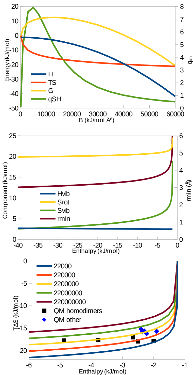
Figure 1. (a) Enthalpy, entropy, free energy (left axis), and the quotient q_{SH} (right axis) as a function of the dispersion parameter B for the purely dispersive interaction of two neutral argon-like atoms with m_1 = m_2 = 40 Da and A = 2.2 \times 10^7 \text{ \AA}^{12} \text{ kJ/mol} . (b) The enthalpy and entropy contributions (left axis), as well as the distance between the two atoms (right axis) as a function of \Delta H for the same values of m_1 , m_2 , and A . (c) Correlation between the enthalpy and entropy as a function of B for different values of A (still with m_1 = m_2 = 40 Da). QM results for noble-gas dimers ( \text{He}_2 , \text{Ne}_2 , \text{Ar}_2 , \text{Kr}_2 , \text{Xe}_2 , and \text{Rn}_2 ) and pairs ( \text{HeNe} , \text{NeAr} , \text{NeKr} , \text{NeXe} , and \text{NeRn} ) are also included with symbols.
