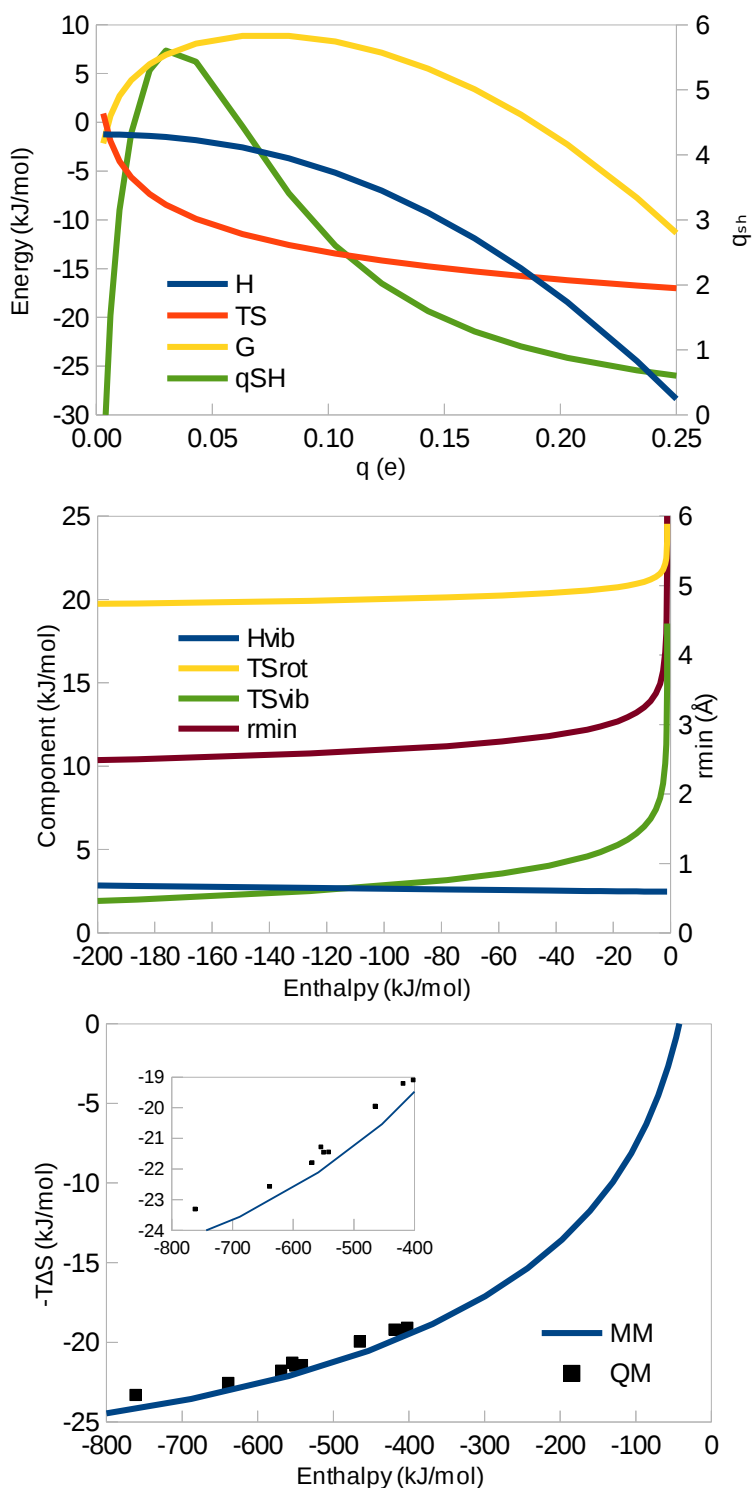
Figure 2. (a) Enthalpy, entropy, free energy (left axis), and q_{SH} (right axis) as a function of the charge q for the interaction of two oppositely charged ions with A = 1.0 \times 10^6 \text{ \AA}^2 \text{kJ/mol} . (b) The enthalpy, entropy terms, and the minimum distance ( r_{min} ) as a function of \Delta H for the same value of A . (c) Enthalpy and entropy as a function of A with q = 1.0 e . QM results for LiF, NaCl, KBr, RbI, CsAt, NaF, KF, RbF, and CsF are also included as black squares. The inset shows a magnification of the QM results. In all figures, m_1 = 23 \text{ Da} (Na) and m_2 = 35 \text{ Da} (Cl).
