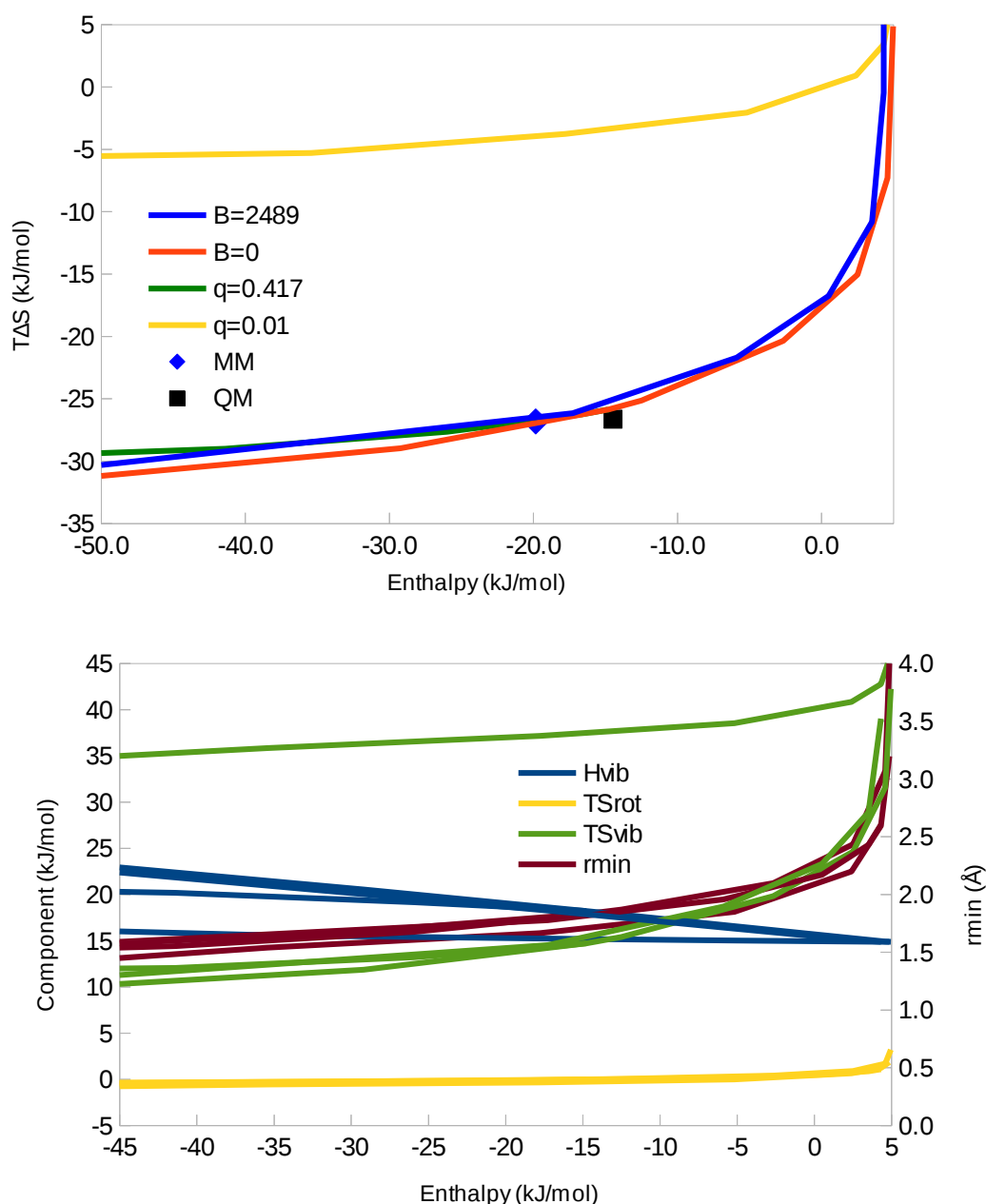
Figure 4. (a) Correlation between the enthalpy and entropy as a function of either q_H or B and with the other parameter fixed at the values given in the legend (and with 2.435 \times 10^6 \text{ \AA}^{12} \text{ kJ/mol} , m_H = 1.008 \text{ Da} , and m_X = 15.9994 \text{ Da} ). The QM and MM results for (\text{H}_2\text{O})_2 are also included with symbols. (b) The enthalpy and entropy components, as well as the minimum distance ( r_{\min} ) as a function of \Delta H for the same parameters, i.e. for each property, the same four lines as in (a) are given. The four lines almost coincide for T\Delta S_{\text{rot}} and r_{\min} , whereas the one for q_H = 0.01 e differs for \Delta H_{\text{vib}} and T\Delta S_{\text{vib}} .
