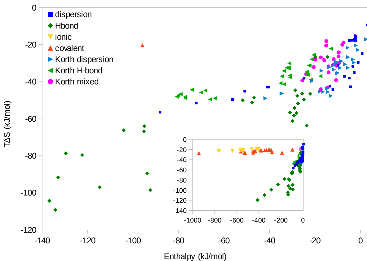
Figure 8. Scatter plots of \Delta H vs. T\Delta S for our 89 molecular complexes and Korth's results for the S22 and S60 sets. The complexes are grouped after the major interactions as dispersive, hydrogen bond, ionic, covalent, or mixed. The inset shows the full range of \Delta H values.
