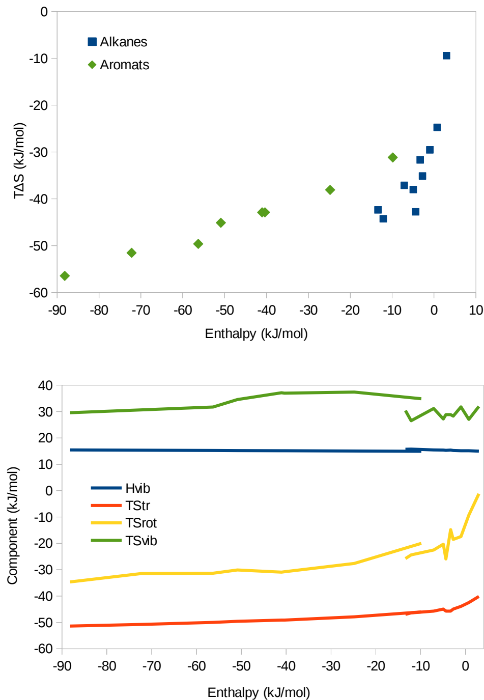
Figure 5. (a) Correlation between the enthalpy and entropy, and (b) the enthalpy and entropy components as a function of the enthalpy for homodimers of the seven smallest n -alkanes, and three simplest branched alkanes (isobutane, isopentane, and neopentane), as well as for eight simple polyaromatic homodimers (benzene, naphthalene, anthracene, phenanthrene, tetracene, pyrene, pentacene, and hexacene).
