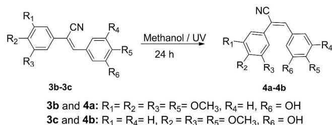
Scheme 2 Synthesis of ( E )-substituted diarylacrylonitrile analogues ( 4a and 4b ).
