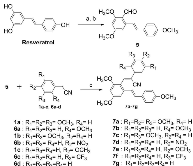
Scheme 3 Synthesis of ( Z )-3-(2,4-dimethoxy-6-(4-methoxystyryl)-2-phenylacrylonitrile analogues ( 7a-7g ). (a) MeI, K 2 CO 3 , acetone; (b) POCl 3 , DMF, 0 °C, 69% yield; (c) NaOMe, EtOH, 6h reflux.
