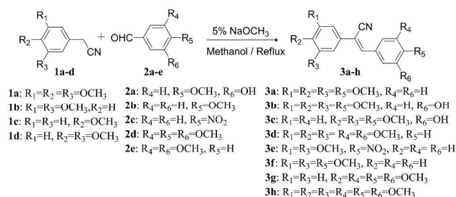
Scheme 1 Synthesis of ( Z )-substituted diarylacrylonitrile analogues ( 3a-3h ).
