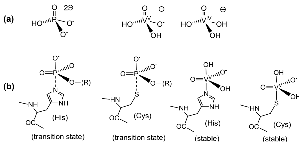
Fig. 1 Analogies and differences between phosphate and vanadates. (a) The predominant protonation states of phosphate and of the vanadates(V) and -(IV) at neutral pH. Due to the low solubility of \text{VO}(\text{OH})_2 , dissolved vanadate(IV) \text{H}_3\text{VO}_4^- (the coordination sphere of \text{V}^{\text{IV}} can be expanded by aqua ligands) is restricted to the nanomolar concentration range. (b) Penta-coordinate species evolving from the interaction between phosphate (and phosphate esters) or vanadate with peptide/protein residues: phosphate forms labile transition states only, symbolized here by a dashed P---N bond to histidine or a P---S bond to cysteine (serinate – not shown – is a third alternative), while vanadate ascertains stable complexes. Examples are
