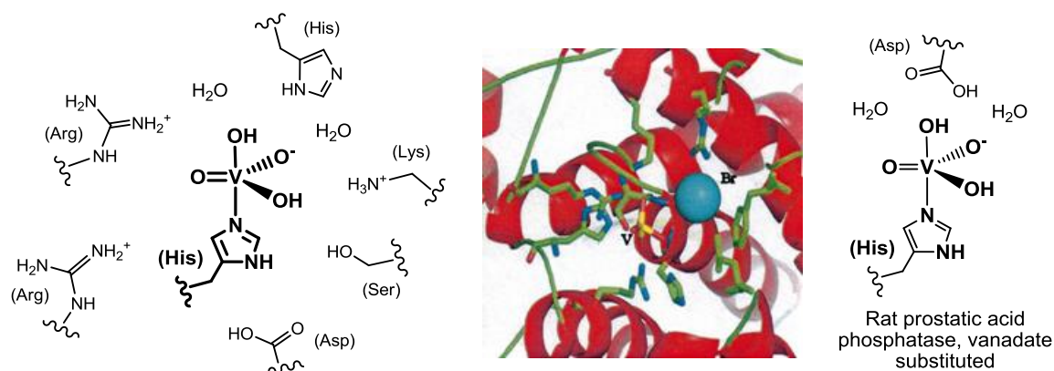
Fig. 4 Left: The vanadate(V) center of the vanadate-dependent bromoperoxidase from A. nodosum . Most of the close-by amino acid residues in (hydrogen-bonding) contact with the active center, plus two water molecules, are shown. Centre: The environment of vanadate (yellow), and the location of bromide (blue) in the C. pilulifera peroxidase. 42 Bromide is positioned within hydrogen bonding distance (ca. 3.0 Å) between vanadate and an arginine residue. Reproduced with permission, © Elsevier. Vanadate, deeply buried in the protein, is accessible via a positively charged channel. Right: The vanadate center in the vanadate variant of rat prostatic acid phosphatase.
