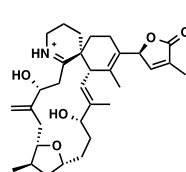
gymnodimine C
