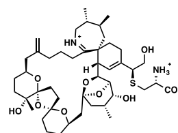
pteriatoxin C
