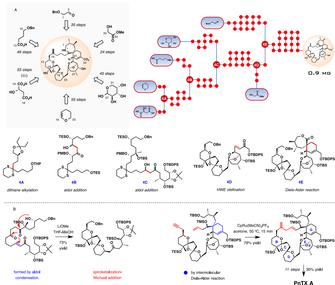
Scheme 4. Total synthesis of (+)-pinnatoxin A by Nakamura, Hashimoto, and co-workers. (A) Schematic outline, a dot graph of the synthesis and central intermediates at points of convergence. (B) Selected key transformations in the synthesis.
