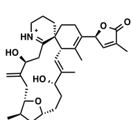
gymnodimine B
