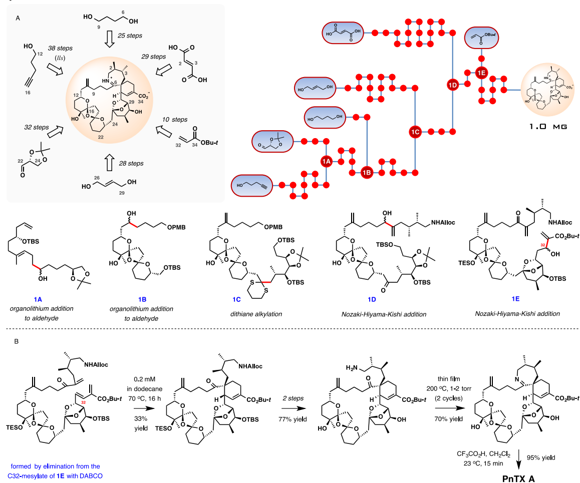
Scheme 1. Total synthesis of (–)-pinnatoxin A by Kishi and co-workers. (A) Schematic outline, a dot graph of the synthesis and central intermediates at points of convergence. (B) Selected key transformations in the synthesis.
