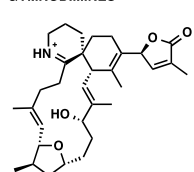
gymnodimine A
