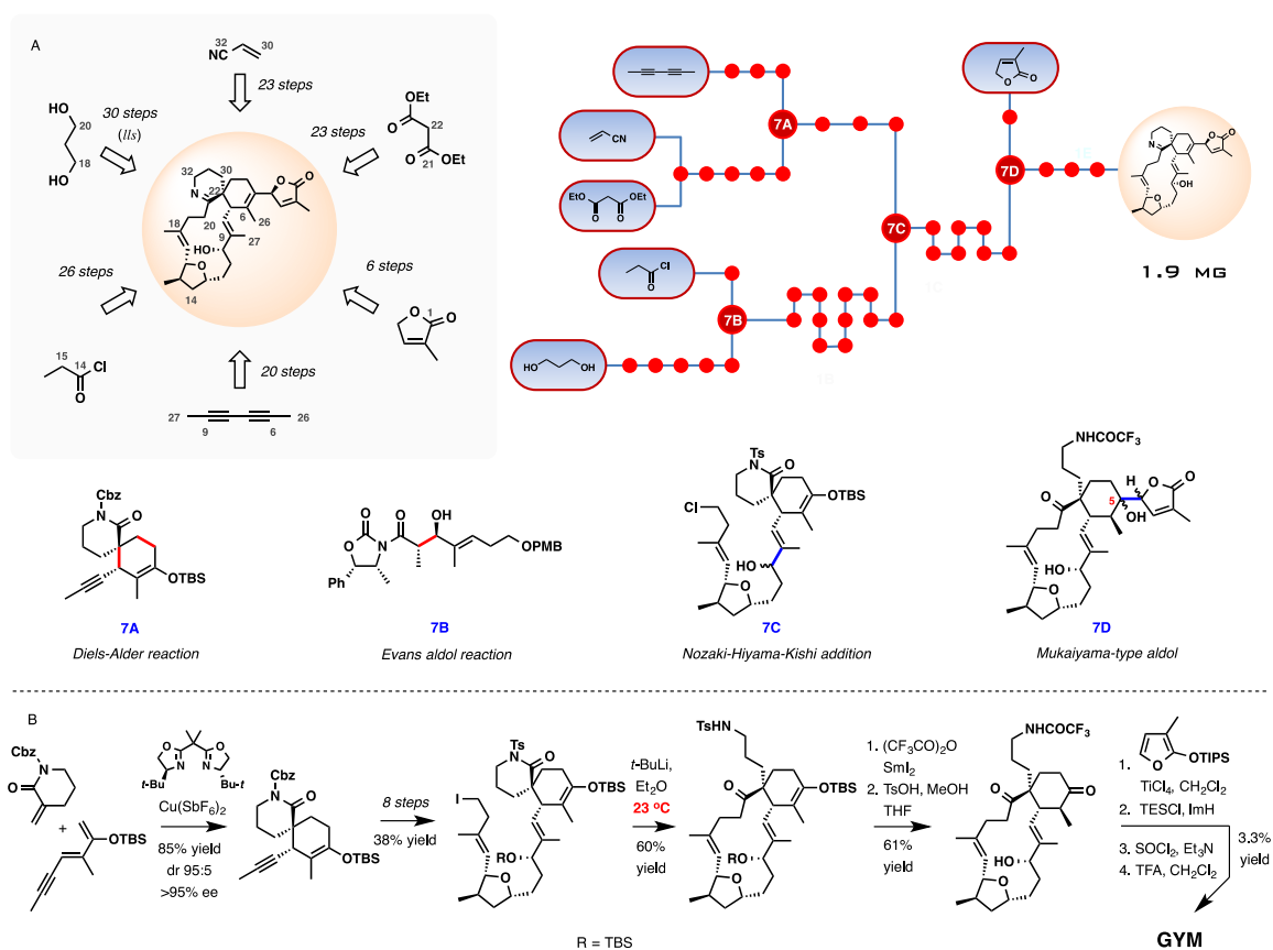
Scheme 7. Total synthesis of (–)-gymnodimine by Romo and co-workers. (A) Schematic outline, a dot graph of the synthesis and central intermediates at points of convergence. (B) Selected key transformations in the synthesis.
