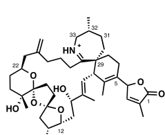
spirolide A
