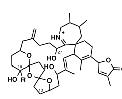
R = Me: 27-hydroxy-13-desmethyl spirolide C R = H: 27-hydroxy-13,19-didesmethyl spirolide C
