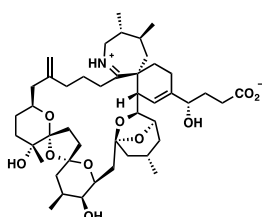
pinnatoxin E
