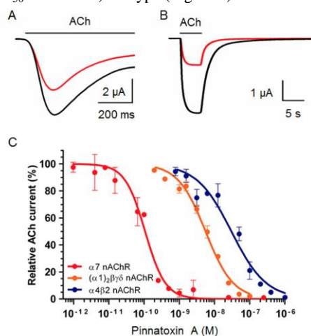
Figure 4. Synthetic PnTX A blocks nAChRs in Xenopus Oocytes. A, B. ACh-evoked nicotinic currents recorded in Xenopus oocytes expressing the human \alpha 7 (A) and human \alpha 4\beta 2 (B) nAChRs, before (black tracing), and after (red tracing) 125 pM (A) and 50 nM (B) PnTX A treatment, respectively. ACh was microperfused, as indicated by the lines above nicotinic current tracing, at concentrations corresponding to the half maximal activation of nAChRs previously determined experimentally ( EC_{50} ; 350 \mu M for human \alpha 7 and 150 \mu M for human \alpha 4\beta 2 ). The holding membrane potential during recordings was -60 mV. C. Concentration-dependent inhibition of ACh-evoked currents by synthetic PnTX A in Xenopus oocytes expressing the human \alpha 7 (red circles and curve) and human \alpha 4\beta 2 (blue circles and curve) neuronal nAChRs, or having incorporated into their membranes the Torpedo \alpha 1\beta 1\gamma\delta muscle type nAChR (orange circles and curve). Amplitudes of the ACh-current peak recorded at a holding membrane potential of -60 mV, in the presence of PnTX A were normalized to control currents and fitted to the Hill equation. Data with error bars represent the mean \pm S.E.M. ( n = 5 ).
