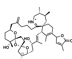
R = Me: spirolide C R = H: 13-desmethyl spirolide C
