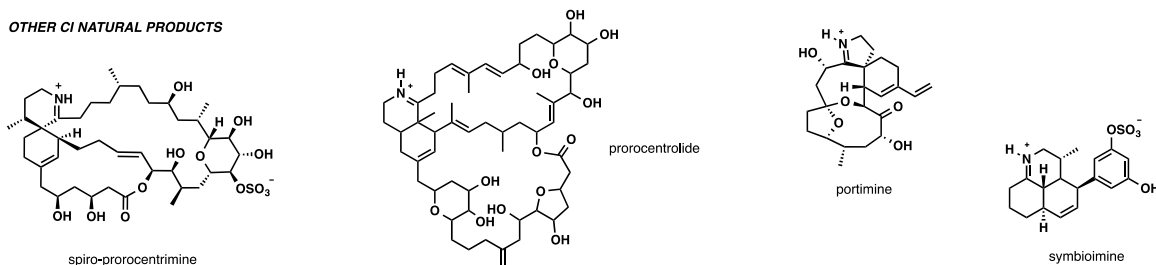
Figure 2. Cyclic Imine toxins and closely related natural products identified as of May 2014.
