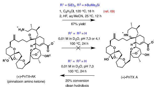
Scheme 5. PnTX A imine condensation/hydrolysis studies.
