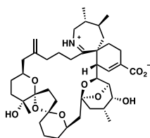
pinnatoxin A
