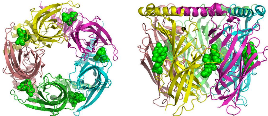
Figure 6. Aplysia -AChBP pentamer in complex with gymnodimine A. Bottom (left) and side (right) views of the X-ray crystallographic structure of gymnodimine A (in green, sphere representation) imbedded at the interfaces of the five subunits of the Aplysia -AChBP pentamer (pdb code 2X00).
