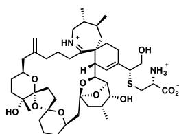
pteriatoxin B
