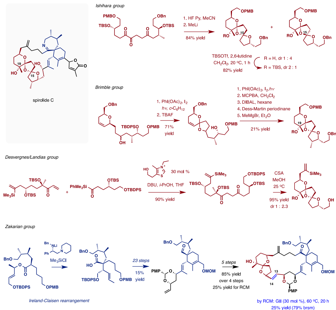
Scheme 6. Synthetic studies directed towards the spiroketal subunit of 13-desmethyl spirolide C.
