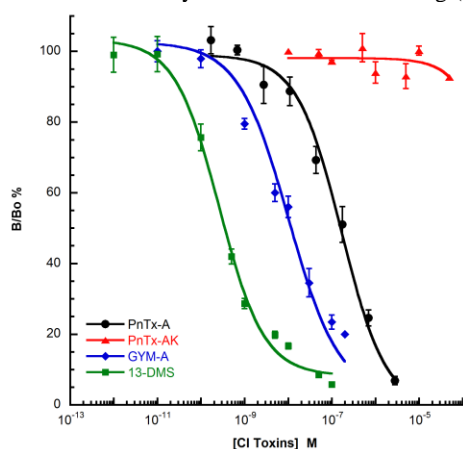
Figure 5. Competition binding curves of pinnatoxin A (PnTX A), pinnatoxin AK (PnTX AK), gymnodimine A (GYM A) and 13 desmethylspirolide C (13-DMS) on \alpha_3\beta_2 nAChRs expressed on HEK-293 cells that interact with ^3\text{H} -epibatidine. The results are expressed as the ratio of specific radiotracer binding measured with (B) or without (Bo) competitive ligand expressed as a percentage. Curve fitting was based on non-linear regression analysis using the Hill equation. Data are mean values \pm SEM of at least three experiments.
