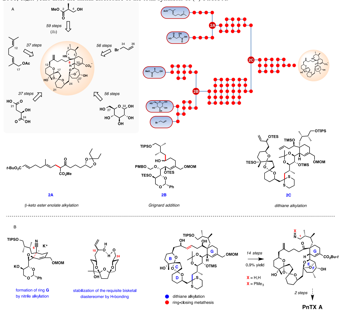
Scheme 2. Formal synthesis of (+)-pinnatoxin A Hirama, Inoue, and co-workers. (A) Schematic outline, a dot graph of the synthesis and central intermediates at points of convergence. (B) Selected key transformations in the synthesis.
