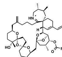
28-O-fatty acyl pinnatoxins G
