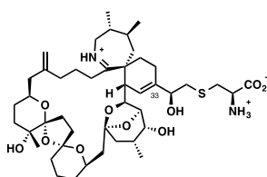
pteriatoxin A
