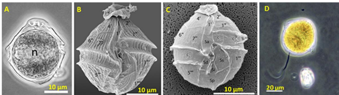
Figure 3. Contrast phase (A) and scanning electron micrographs (B and C) of the dinoflagellate Vulcanodinium rugosum . Note in (A), the cell nucleus (n). (B) Ventral view of the dinoflagellate. Note the small indentation in the c6 plate (white arrow). (C) Smaller form of the dinoflagellate revealing the arrangement of its thecal surface. Adapted with permission from Nézan and Chomérat (2011; Figures 4, 7 and 25). (D) Producer of the spiro sides, Alexandrium ostenfeldii . 39 Scale bar = 20 µm.
