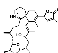
12-methyl gymnodimine (not fully assigned, configurations by analogy)
