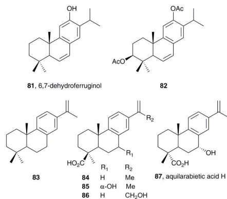
Figure 9. Abietatetraenes 81-87 .
