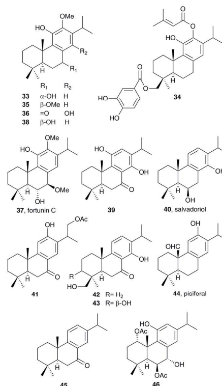
Figure 4. Abietatrienes 33-46 .
