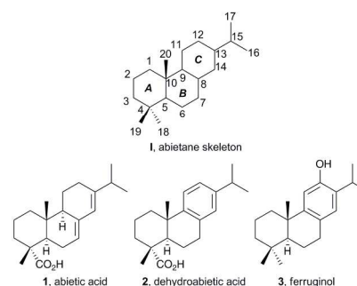
Figure 1. Abietane numbering system and abietic acid ( 1 ).
