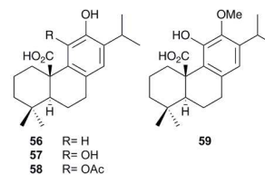
Figure 6. Pisiferic acid ( 56 ) and related metabolites.
