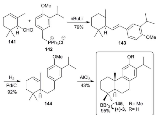
Scheme 15. Matsumoto's enantioselective synthesis of ferruginol ( 3 ).
