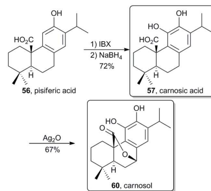
Scheme 9. Tada's synthesis of carnosic acid ( 57 ) and carnosol ( 60 ).
