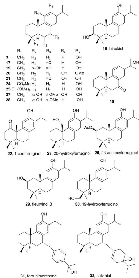
Figure 3. Ferruginol ( 3 ) and related metabolites.
