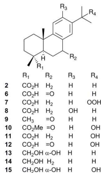
Figure 2. Dehydroabietic acid ( 2 ) related metabolites.
