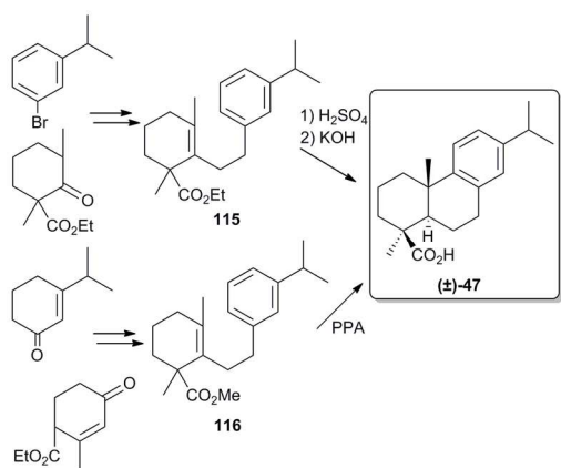
Scheme 11. Haworth's and Sharma's syntheses of callitricic acid (47).
