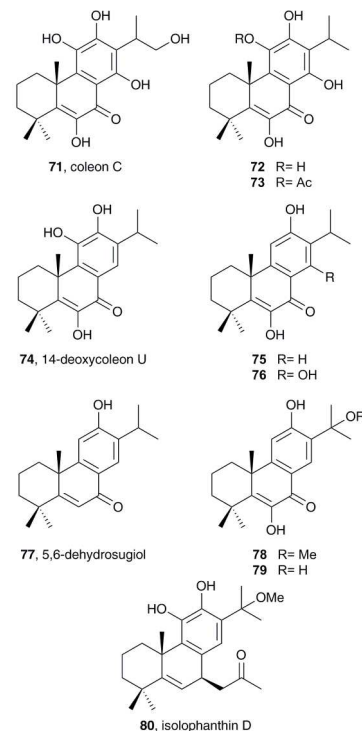
Figure 8. Abietatetraenes 71-80 .
