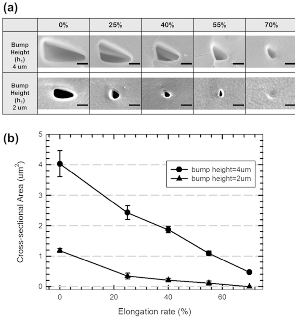
Figure 3. Tunable size and shape of PNSA. (a) SEM image of the size/shape variation of nanochannels as a function of the elongation rate (scale bar: 500 nm). (b) Size characteristic curve of the cross-sectional area of the nanochannel according to the elongation rate. 90x98mm (300 x 300 DPI)
