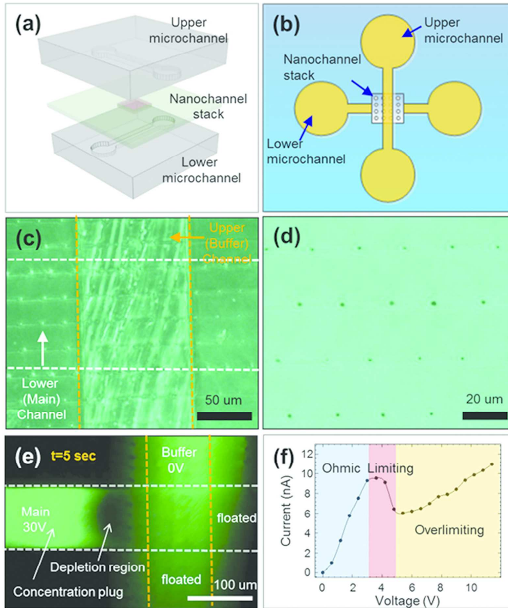
Figure 4. Ion concentration polarization (ICP) phenomenon using PNSA. (a) Schematic illustration of the microchip used for testing ICP, which consisted of three PDMS layers. (b) Schematic illustration of the orthogonal alignment of each layer. (c) Microscopic image of the 3-D micro/nano-hybrid system. (d) Magnified view of PNSA at the junction of the upper and lower microchannels. (e) Fluorescent image of the development of the ion depletion zone by applying an external voltage of 30 V for 5 s. (f) I-V characteristics when applying an external electric field to the device; ohmic limiting and overlimiting regions appeared sequentially.
