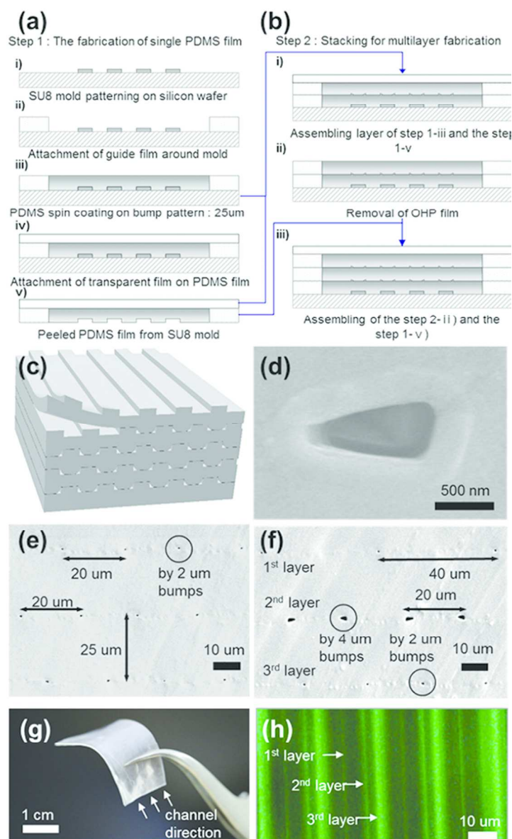
Figure 1. Fabrication method and the resulting polymeric nanochannel stack array (PNSA). (a) Fabrication process flow of the PDMS film with bump patterns, (b) assembling process flow of the stacking method, and (c) schematic diagram of the PNSA. Each layer contained numerous nanochannels of constant pitch at each layer. (d) Scanning electron microscopy (SEM) image of individual nanochannel openings created by PDMS-to-PDMS bonding (bump height = 2 \mu\text{m} ). (e) SEM image of the PNSA structure, including nanochannels having a constant pitch of 20 \mu\text{m} . Each layer had a thickness of 25 \mu\text{m} , created by spin-coating the PDMS mixture at speeds of 4000 rpm. (f) SEM image of PNSAs of various sizes and pitches at each inner layer. The first layer had a pitch of 40 \mu\text{m} ; the second layer had a larger nanochannel than the third layer. (g) Image of the PNSA created by the aforementioned stacking technique. This structure has flexibility, an ultra-high aspect ratio, and orthogonality. (h) Fluorescent image inside the nanochannels of each inner layer. 82x140mm (300 x 300 DPI)
