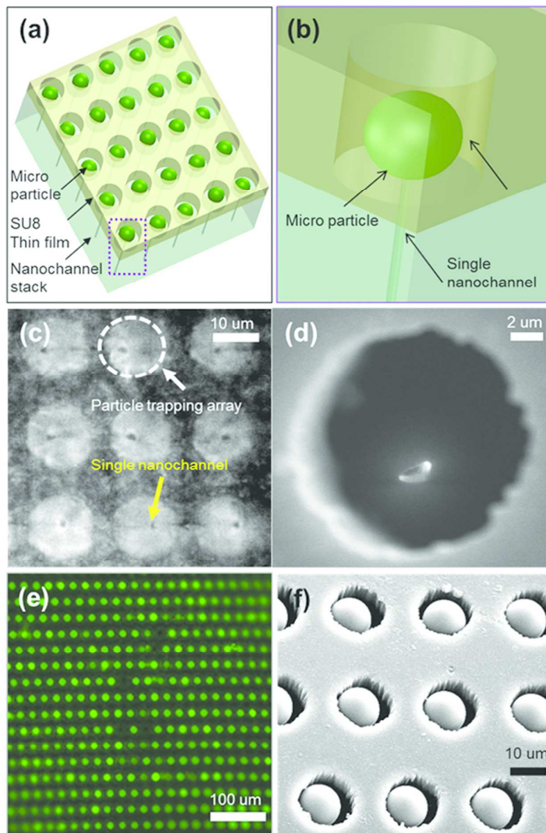
Figure 5. Multiplexed one microstructure-on-one nanostructure interfacing using PNSA. (a) Schematic illustration of micro-particle/nanochannel interfacing using a support layer on top of PNSA. (b) Magnified schematic view of one chamber loaded with one microparticle. (c) Microscopic image of the positioning of a single nanochannel with the microchamber. Two images are overlaid: one shows the nanochannel and the other shows the microchamber. (d) SEM image of a single chamber aligned on top of a single nanochannel. (e) Fluorescent image of multiplexed one microstructure-on-one nanostructure interfacing of fluorescent particles and nanochannels. (f) SEM image of (e). 82x124mm (300 x 300 DPI)
