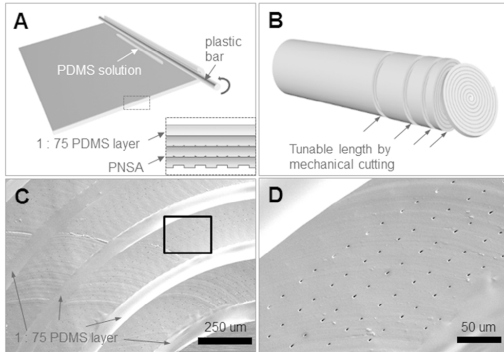
Figure 2. Large-area integration by PNSA rolling. (a) Schematic illustration of large-area integration using a sticky (1:75) PDMS layer. Magnified inset image showing a cross-sectional view before rolling. (b) Schematic illustration of the rolled PNSA structure; this structure can be mechanically cut on demand. (c) SEM image of the radially formed PNSA and PDMS films of 1:75 weight ratio and (d) magnified view of (c). 83x57mm (300 x 300 DPI)
