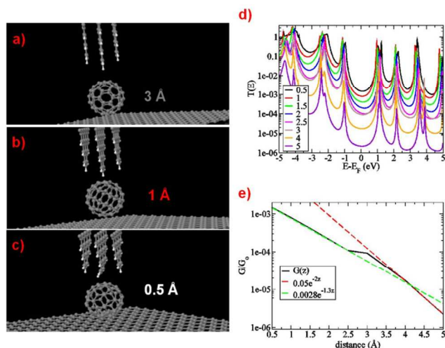
Figure 4 Geometric representation of the graphene tip interacting with a C_{60} molecule adsorbed on graphene (a) at a large distance, (b) at an intermediate regime and (c) the short
