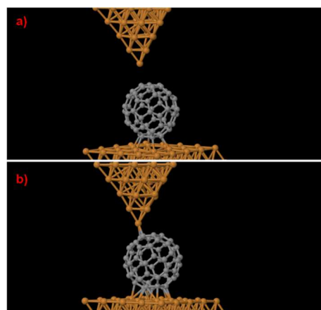
Figure 5 Calculated geometries of a Cu-tip- C_{60} junction calculated for different positions: a)-far distance, and b)-contact mode. One can observe the formation of a molecular contact between the tip and the molecule, to the contrary of the situation with the carbon tip.
