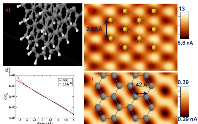
Figure 1. (a) Geometric model for the hydrogen decorated graphitic tip. The tip is formed by three triangular graphene sheets, stacked together through van der Waals interactions at an equilibrium distance of 3.1 Å. (b) Computed STM image of Au(111) surface. The tip-sample distance was fixed to 4 Å and the bias voltage was 0.1 V. The gold surface atoms are superimposed. (c) Computed STM image of a graphene plane in the same conditions as in (b). The corresponding structure has also been superimposed. (d) conductance (black line) in units of G_0 on a logarithmic scale versus vertical tip displacement above the graphene plane. The red curve corresponds to a fit to an exponential function, as indicated in the legend. (e) Computed STM image of a graphene plane with a tip-sample distance of 1.42 Å and bias voltage of 0.1 V. The corresponding structure has also been superimposed.
