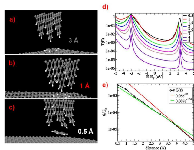
Figure 3. Geometric representation of the graphene tip in interaction with a benzene molecule adsorbed on graphene (a) at a large distance, (b) at an intermediate distance, and (c) in short distance regime (notice the deformation of the tip). (d) Transmission as a function of energy on a logarithmic scale for benzene on graphene using the graphene tip, at different vertical distances (in Å). (e) Conductance as a function of the tip-molecule distance on a logarithmic scale (black line). The red and green lines correspond to exponential fits in different distance regions (the functions are indicated in the legend).
