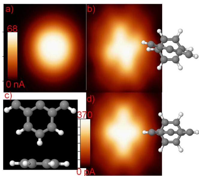
Figure 2 Comparison of STM image calculations of benzene on graphene using (a) the Cu tip and (b) and (d) the graphitic tip for two orientations. The corresponding geometries of the benzene with the graphitic tip are presented on the right side. In (c) a lateral view of the tip falling over the center of the hexagon is shown. All the calculations were performed using a voltage of 0.1 V and a tip-benzene distance of 4 Å.
