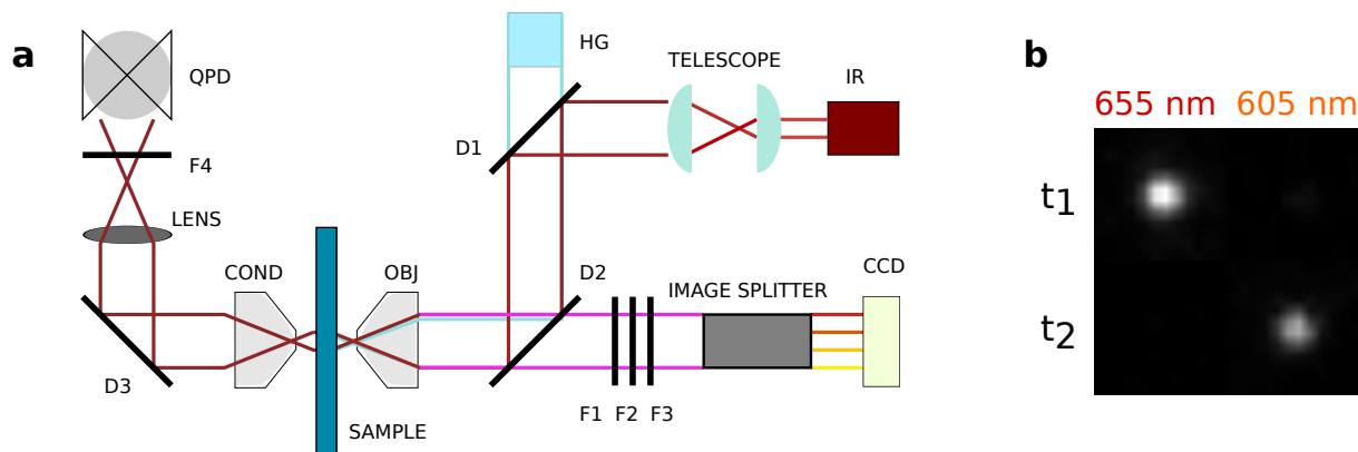
Fig. 1 a: Schematic of the experimental setup. The 1064 nm trapping laser beam (IR) is expanded by a telescope and deflected by two dichroic mirrors (D1, D2) before it enters the sample trough through the objective (OBJ) of an inverted Leica SP5 microscope. The positions visited by the trapped object are measured by a quadrant photodiode (QPD) using the forward scattered light that is collected by the condenser (COND) and deflected by a dichroic mirror (D3). A lens focuses the forward scattered light onto the QPD and a filter (F4) reduces the intensity. Excitation light from a mercury lamp (HG) facilitates navigation in the sample, but during the experiments the QDs are solely excited by the IR laser beam. The fluorescent emission from a single QD is filtered by two hot mirrors and color filters (F1, F2, F3). Spectral selection is performed with an image splitter and projected onto the sensitive EMCCD. b: Snapshots at two different times ( t_1 and t_2 ) of an immobilized QD blue-shifting from an emission wavelength of (655 \pm 20) nm to (605 \pm 20) nm.
