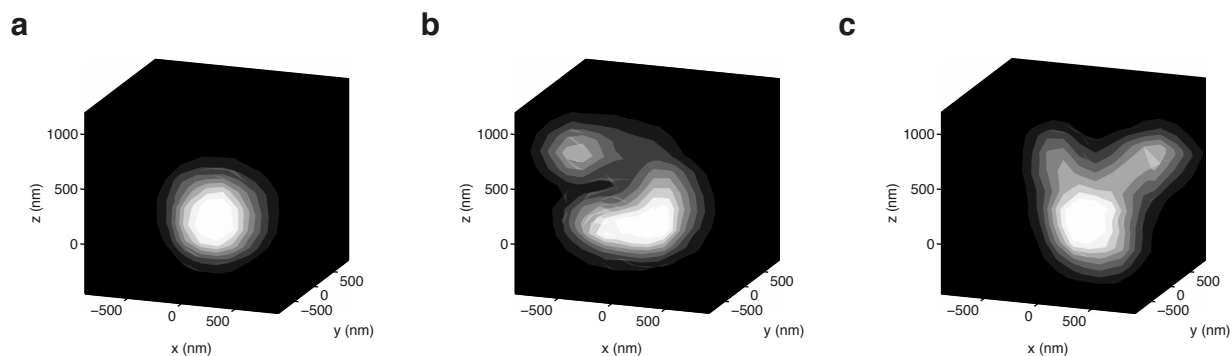
Fig. 3 Three dimensional histograms of the positions visited by three individual colloidal quantum dots ( a , b and c ) moving in an optical trapping potential where the laser power at the sample was 250 mW. The contours signify percentage of the counts in 10% steps and z = 0 nm is set as the mean value of (a).
