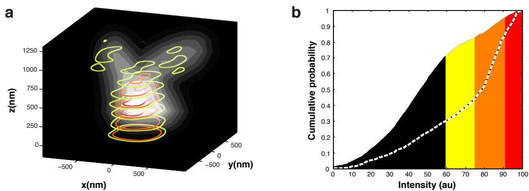
Fig. 5 Comparison of the focal intensity distribution to the positions visited by the trapped QD. a: Overlay of 3D histogram of positions visited by a colloidal QD (the contours signify 10% steps of the counts) with an intensity contour plot of the focal region. b: Probability that a trapped QD is located within a region with at least a certain intensity level. The color coding is the same in (a). The black-white dashed line shows an estimate of the accumulated probability of detecting a photon emitted from a QD as function of focal intensity.
