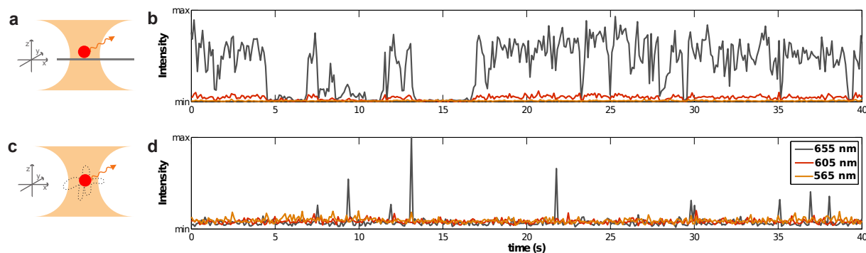
Fig. 2 Two-photon excitation of an immobilized or optically trapped QD. a: Sketch of the experiment where a QD, adhered to the surface, is two-photon excited by the trapping laser. b: Emitted intensity versus time from a single QD adhered to the surface. The sketch is not to scale. c: Sketch of the experiment where a QD is optically trapped and two-photon excited in the solution. The QD performs significant thermal fluctuations within the trapping volume; indicated by the punctuated line. The sketch is not to scale. d: Emitted intensity versus time from a single QD optically trapped in solution \sim 5 \mu\text{m} above the surface. The intensity at different emission wavelengths (655 nm, 605 nm, and 565 nm) are denoted with different colors. A clear signal is only recorded in the spectral 655 nm spectral window but the two other windows (605 nm and 565 nm) are included for comparison.
