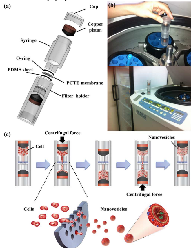
Fig. 1 (a) Sectional view of device. (b) Photograph of device in operation. (c) Schematic process of nanovesicle generation. After cells were loaded into the syringe, centrifugal force was applied to extrude them. During extrusion, the polycarbonate filter imposes surface tension and generates nanovesicles when they pass through the filter pores.
