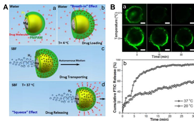
Fig. 4 A) Schematic demonstration of the drug (a, b) loading, (c) transporting, and (d) releasing behaviors of the Mg/Pt-PNIPAM Janus micromotors. B) Fluorescent images representing the drug release from the Mg/Pt-PNIPAM Janus microspheres (a) and the normalized average cumulative drug release profiles (b) at 20 and 37°C versus time. Scale bars: 10 \mu\text{m} . (Reproduced from ref 40, American Chemical Society 2014)
