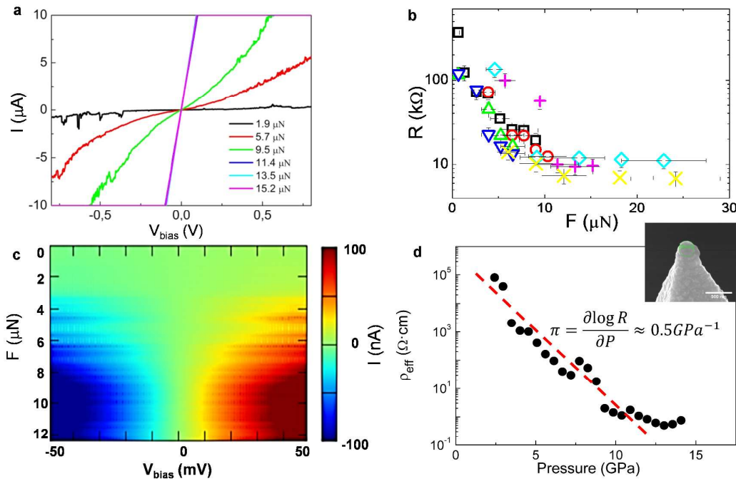
Figure 2. Local transport measurements a. I(V_{\text{bias}}) characteristic curves obtained for applied loads ranging from 1.9 to 15.2 \mu\text{N} (Note that the three curves under higher loads overlap within this scale). b. Resistance as a function of the applied load. Data include different sets of experiments using PtIr coated tips ( r_{\text{tip}} \sim 50 nm) at a single point for diverse loads (black squares and red circles), at different points for each specific load (all the others), and at reduced relative humidity (pink crosses). c. 3D map of conductivity (color scale) as a function of tip-sample voltage ( V_{\text{bias}} ) and normal force ( F ), obtained with a B-doped diamond coated tip of r_{\text{tip}} \sim 150 nm as determined by the SEM after the measurements (inset in d, bar scale is 500nm) d. Effective resistivity as a function of the applied pressure, both obtained from the 3D map. c. The red dashed lines are meant to guide the eyes. Note the evident logarithmic decay over pressure.
